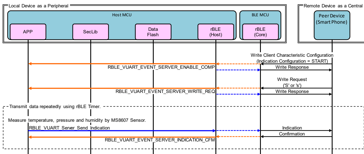
Figure 7-10 Profile Communication sequence chart
