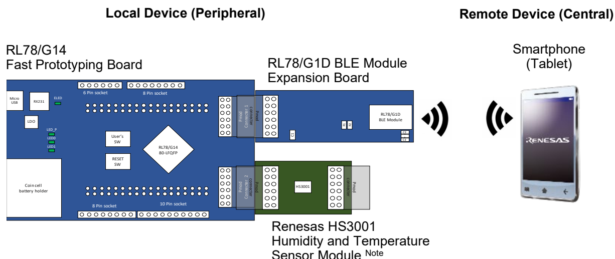
Figure 3-1 Device Compositions
