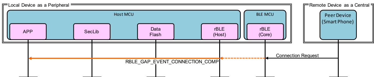
Figure 7-5 Connection sequence chart
