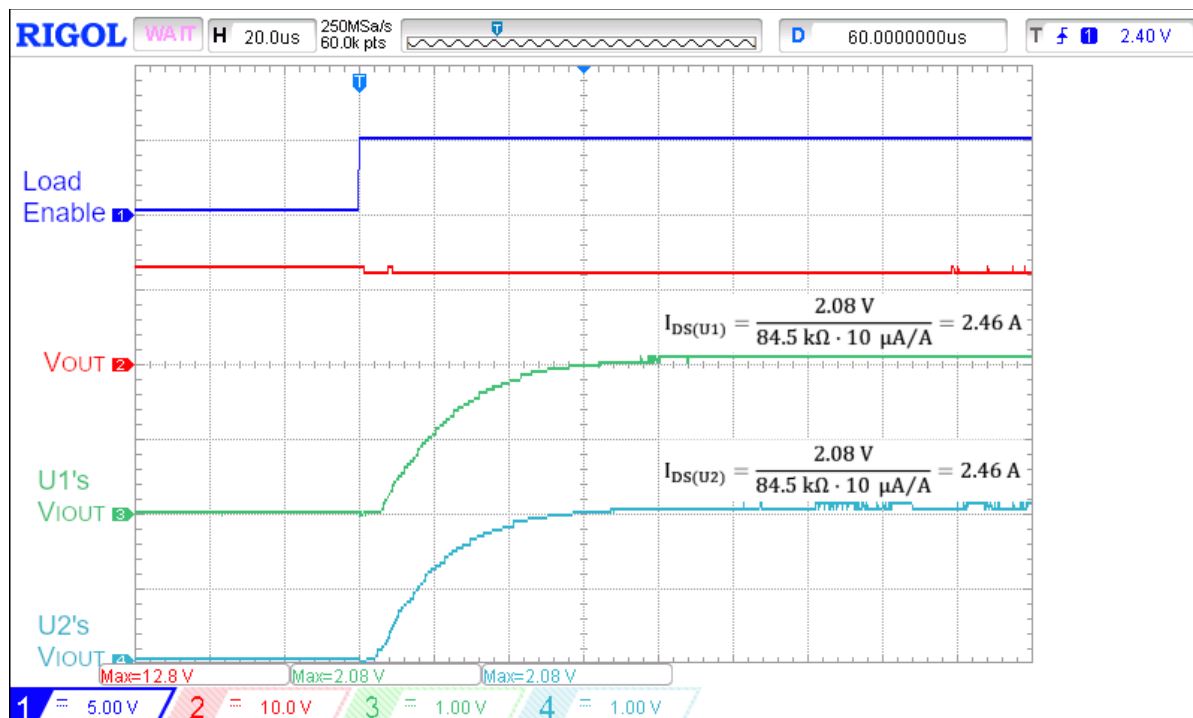
Figure 10: Two SLG59H1006Vs Operating in Parallel: IOUT operation; V_{\text{LOGIC}} = 5\text{ V} , V_{\text{IN}} = 12\text{ V} , I_{\text{DS}} = 5\text{ A} R_{\text{IOUT\_U1}} = 84.5\text{ k}\Omega , C_{\text{IOUT\_U1}} = 180\text{ pF} , R_{\text{IOUT\_U2}} = 84.5\text{ k}\Omega , C_{\text{IOUT\_U2}} = 180\text{ pF} , ON = HIGH
