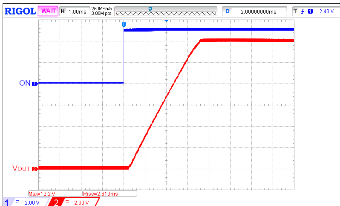
Figure 3: Two SLG59H1006Vs Operating in Parallel: Turn ON Operation; V_{\text{LOGIC}} = 5\text{ V} , V_{\text{IN}} = 12\text{ V} , C_{\text{SLEW}} = 18\text{ nF} , R_{\text{LOAD}} = 100\text{ }\Omega , C_{\text{LOAD}} = 10\text{ }\mu\text{F} , Load Enable = HIGH
