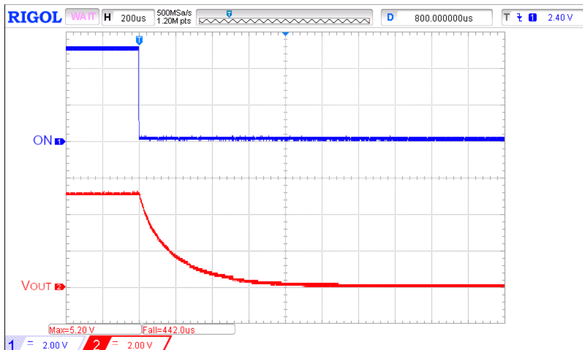
Figure 24: SLG59M1568V Turn OFF Operation; V_{DD} = 5\text{ V} , V_{IN} = 5\text{ V} , C_{SLEW} = 4.7\text{ nF} , R_{LOAD} = 20\text{ }\Omega , C_{LOAD} = 10\text{ }\mu\text{F} , Load Enable = HIGH
