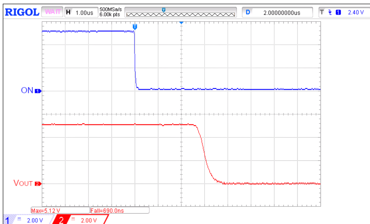
Figure 15: Two SLG59M1714Vs Operating in Parallel: Turn OFF Operation; V_{DD} = 5 V, V_{IN} = 5 V, R_{LOAD} = 100 \Omega , no C_{LOAD} , Load Enable = HIGH
