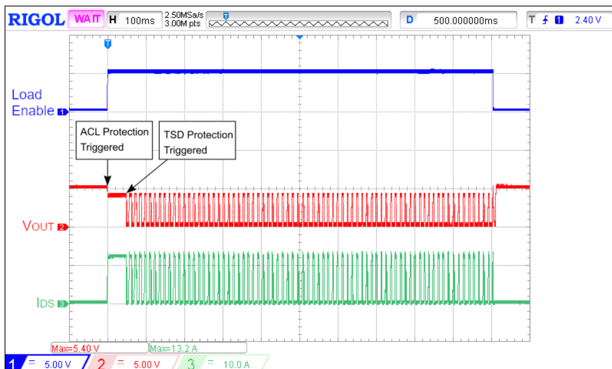
Figure 25: SLG59M1568V ACL with thermal protection operation; V_{DD} = 5\text{ V} , V_{IN} = 5\text{ V} , I_{ACL} = 12\text{ A} , R_{LOAD} = 0.4\text{ }\Omega , C_{LOAD} = 10\text{ }\mu\text{F} , ON = HIGH
