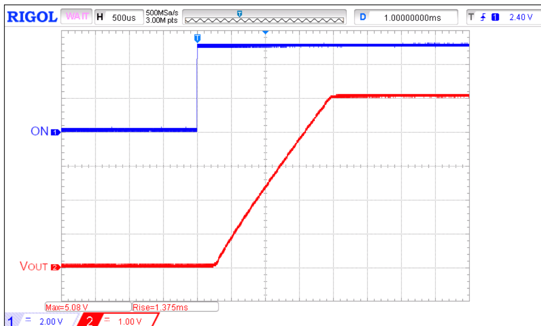
Figure 14: Two SLG59M1714Vs Operating in Parallel: Turn ON Operation; V_{DD} = 5 V, V_{IN} = 5 V, R_{LOAD} = 100 \Omega , C_{LOAD} = 10 \mu F, Load Enable = HIGH
