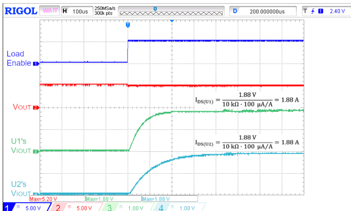
Figure 18: Two SLG59M1714Vs Operating in Parallel: Independent I_{OUT} operation; V_{DD} = 5\text{ V} , V_{IN} = 5\text{ V} , I_{DS} = 4\text{ A} , R_{IOUT\_U1} = 10\text{ k}\Omega , C_{IOUT\_U1} = 10\text{ nF} , R_{IOUT\_U2} = 10\text{ k}\Omega , C_{IOUT\_U2} = 10\text{ nF} , ON = \text{HIGH}
