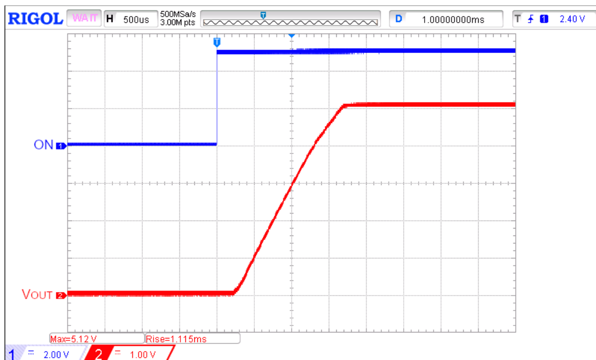
Figure 2: Two SLG59H1006Vs Operating in Parallel: Turn ON Operation; V_{\text{LOGIC}} = 5\text{ V} , V_{\text{IN}} = 5\text{ V} , C_{\text{SLEW}} = 18\text{ nF} , R_{\text{LOAD}} = 100\text{ }\Omega , C_{\text{LOAD}} = 10\text{ }\mu\text{F} , Load Enable = HIGH
