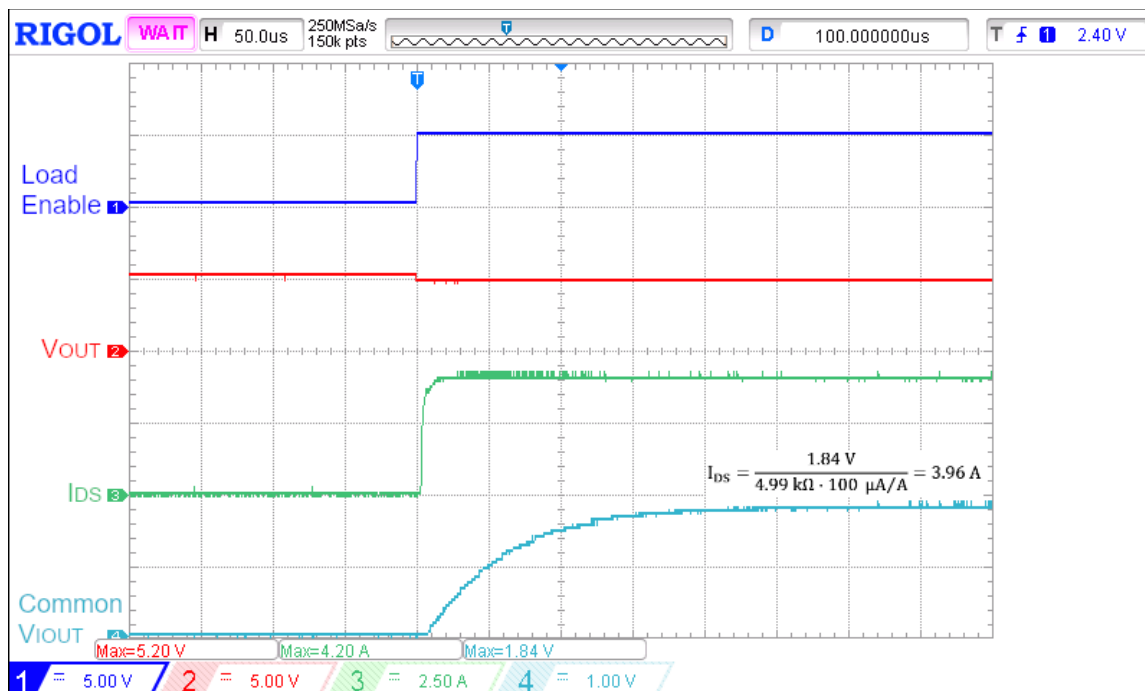
Figure 20: Two SLG59M1714Vs Operating in Parallel: Common IOUT operation; V_{DD} = 5\text{ V} , V_{IN} = 5\text{ V} , I_{DS} = 4\text{ A} , R_{IOUT} = 4.99\text{ k}\Omega , C_{IOUT} = 10\text{ nF} , ON = HIGH
