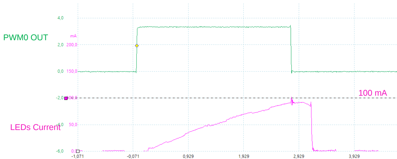
Figure 9: Current Limitation
