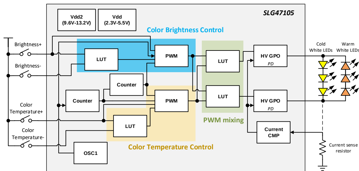
Figure 3: Block Diagram
