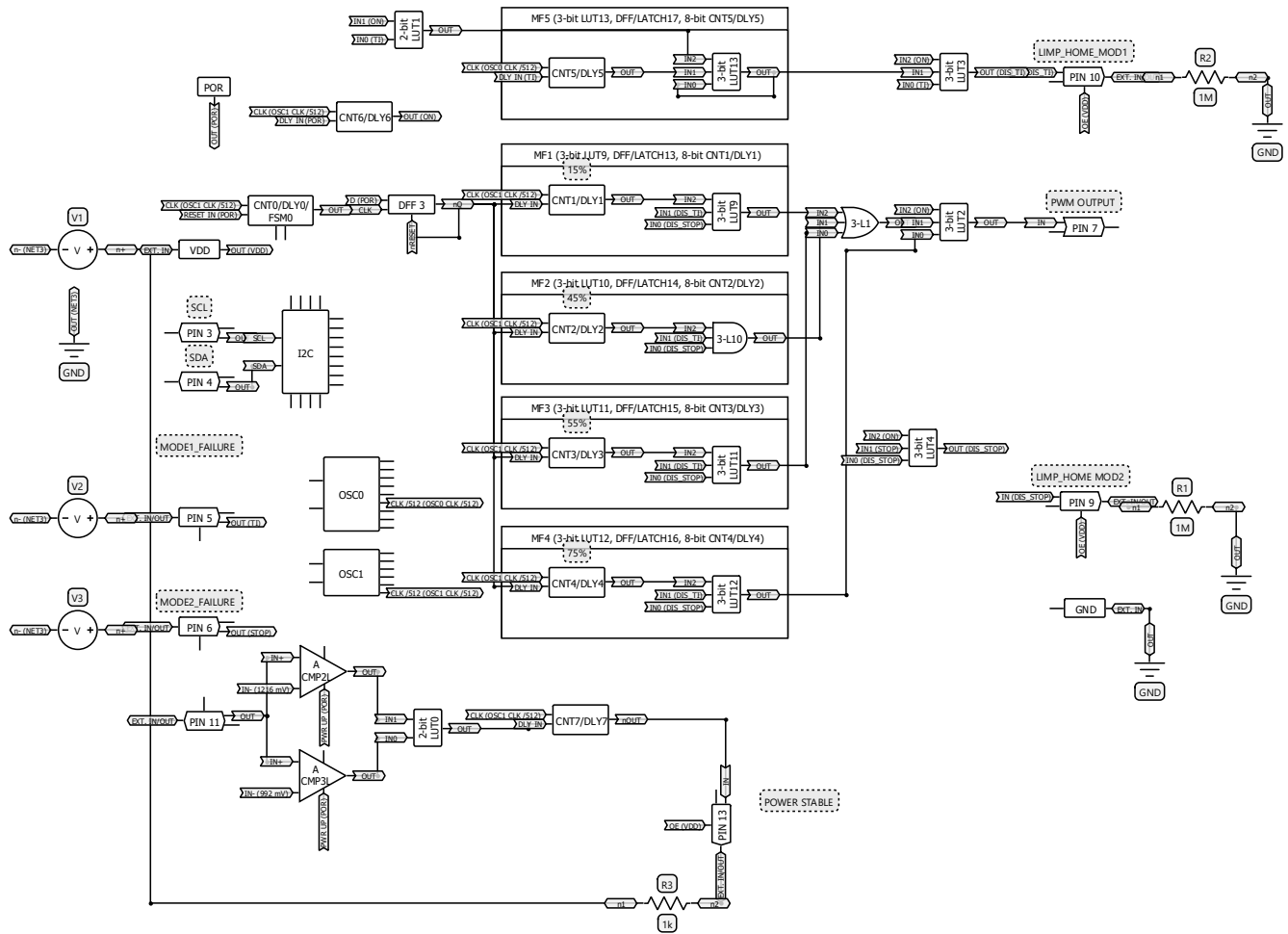
Figure 2: SLG46855-AP Configuration
