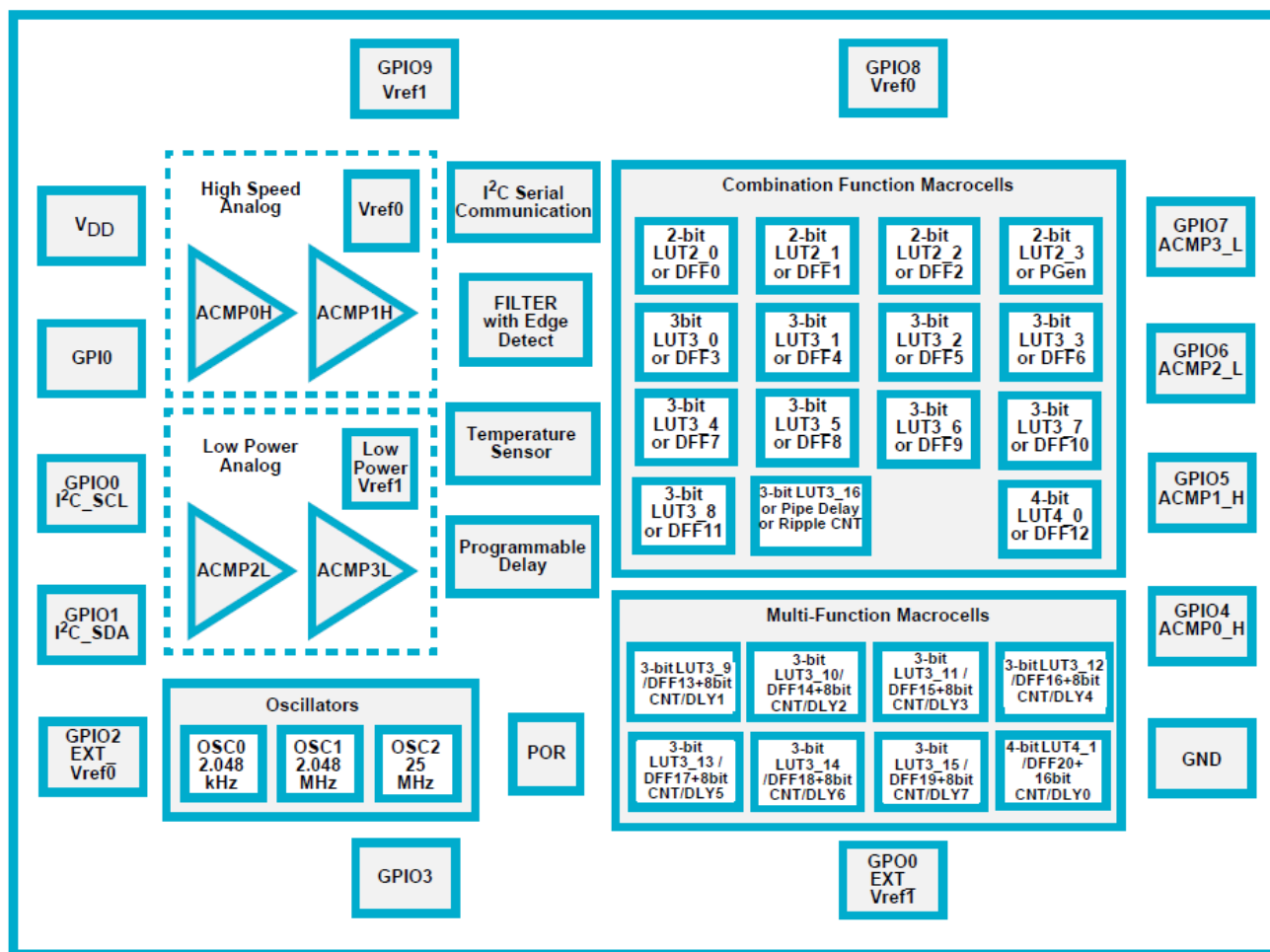
Figure 1: Block Diagram
