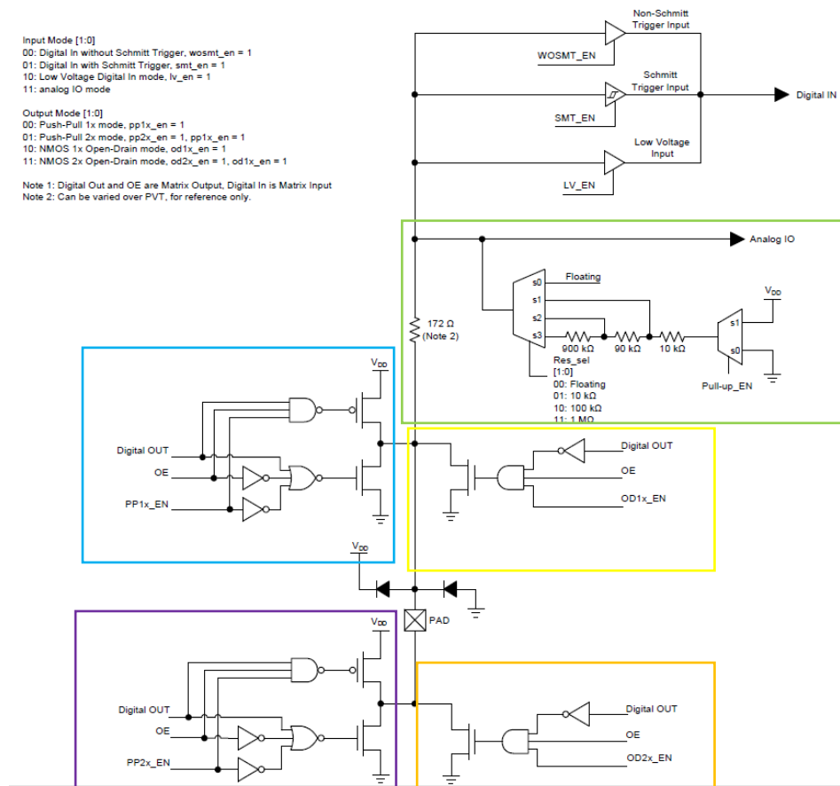
Figure 3: PIN10 (GPIO5)
