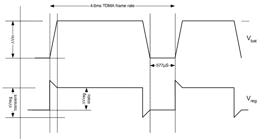
Figure 8: Line Regulation
