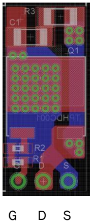
Figure 4. TPHDC001 PCB Layout (GDS output terminal) The PCB specifications for the daughter card are below:
