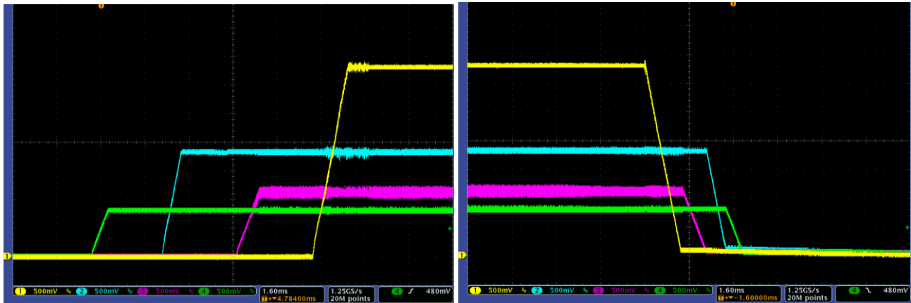
Figure 3. DA9080-66FCBx Power Up/Down
