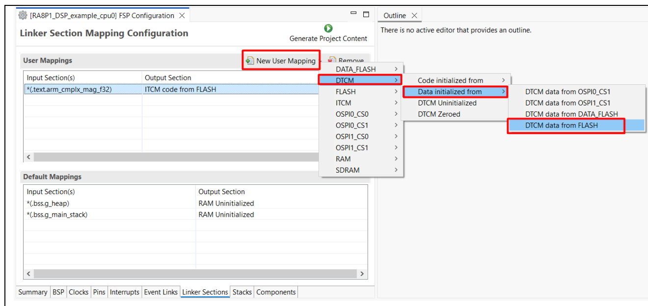
Figure 30. Example of Defining a New Section Mapping for DTCM
