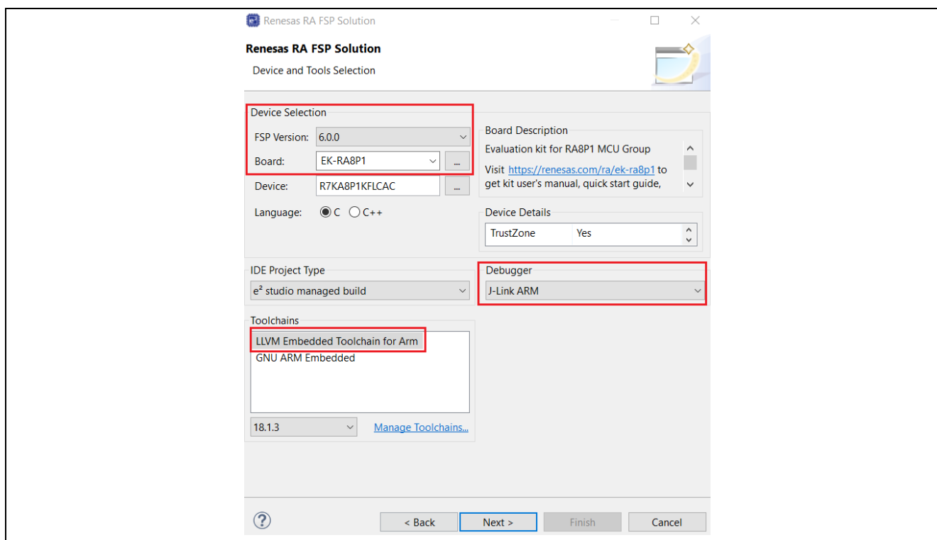
Figure 3. Example of Project Selections
