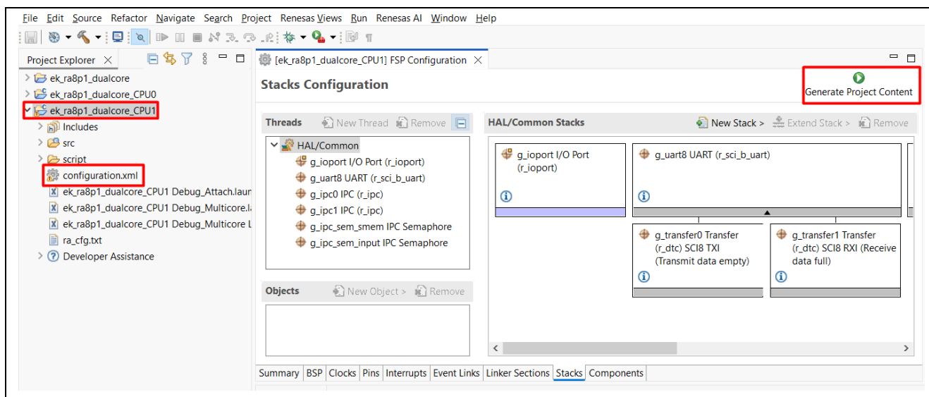
Figure 56. Example of Generate Project Content on CPU1 Project
