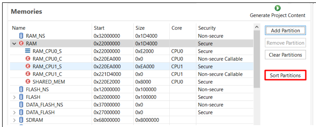
Figure 48. Example of Shortening Partitions in RAM
