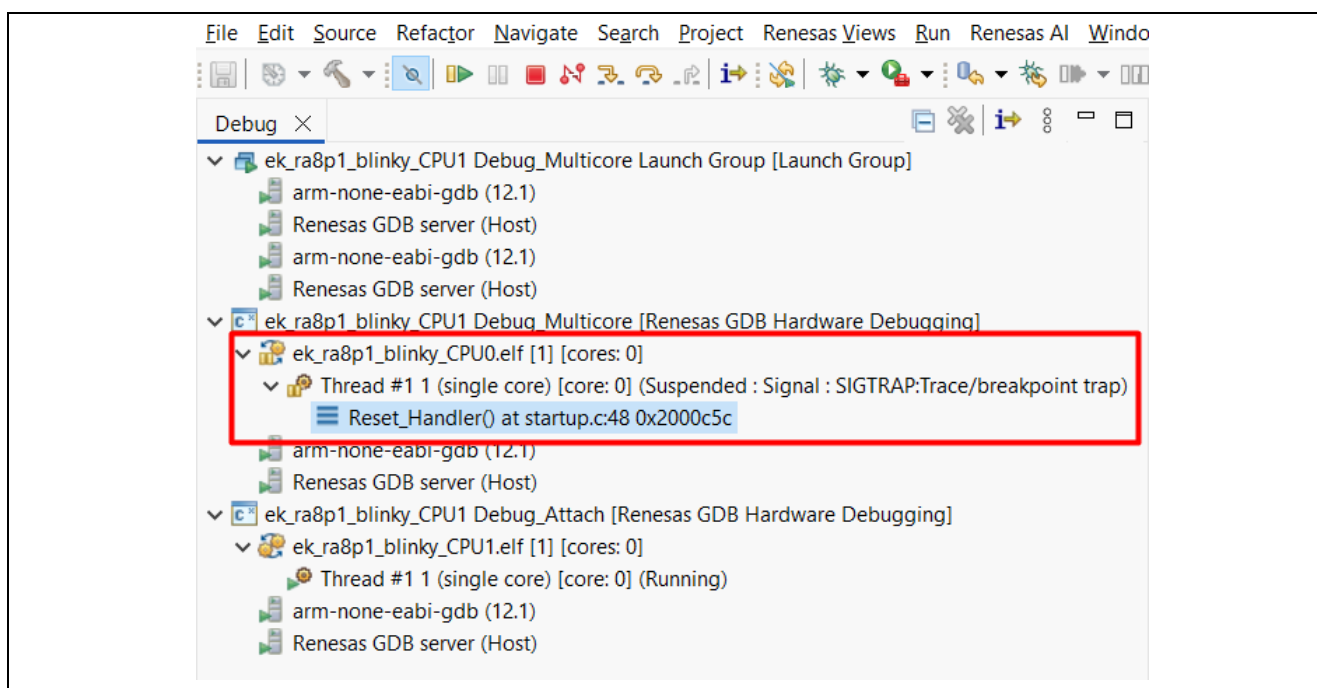
Figure 15. Example of Startup Debug State for Dual-Core Execution.
