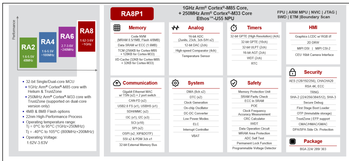
Figure 1. Example of Key Features in RA8P1 MCU
