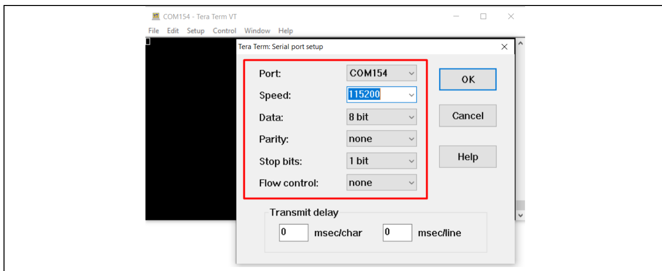
Figure 71. Example of Set Up Tera Term Serial Terminal
