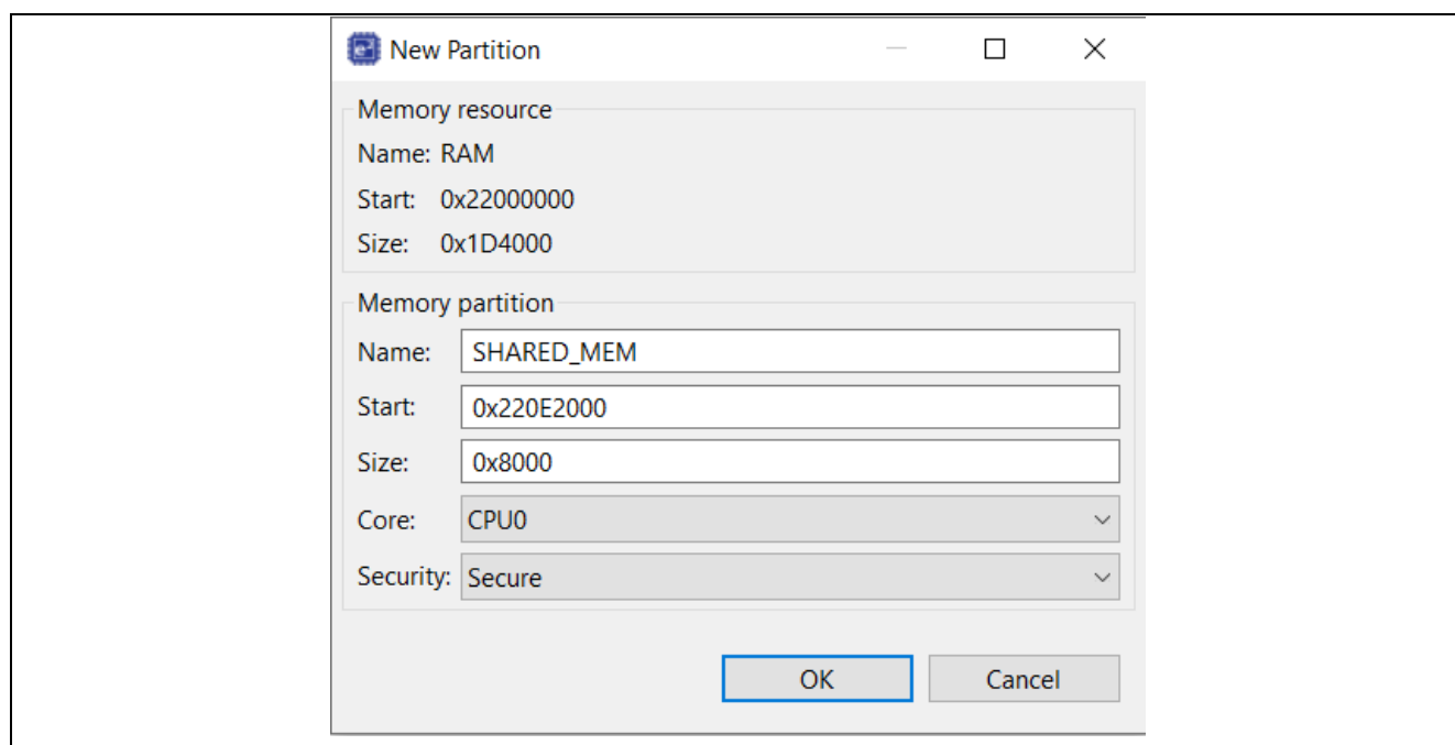
Figure 47. Example of Defining a Shared Memory Partition
