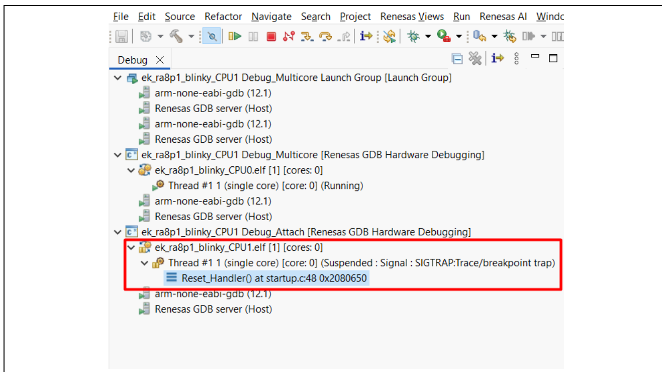
Figure 16. Example of Debug State after R_BSP_SecondaryCoreStart()
