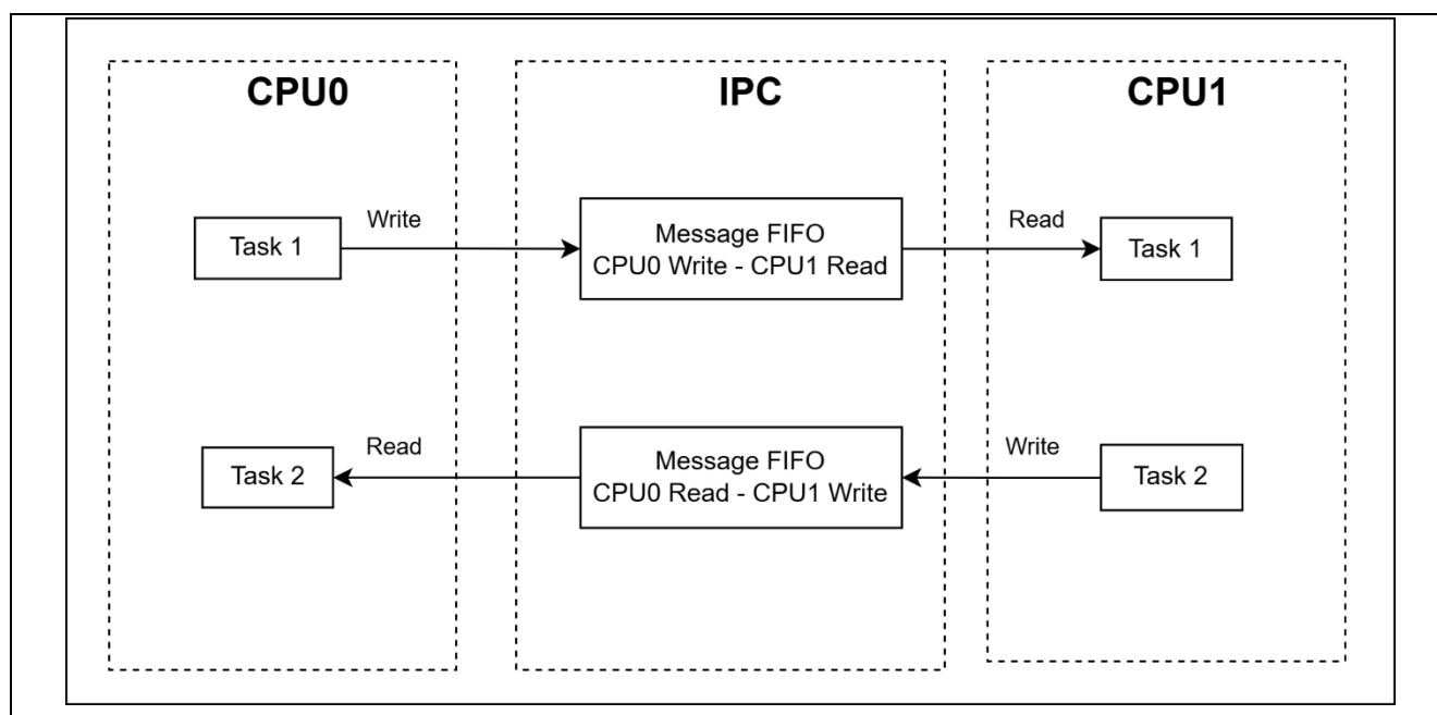
Figure 19. Example of Data Exchange with IPC-Messages FIFO
