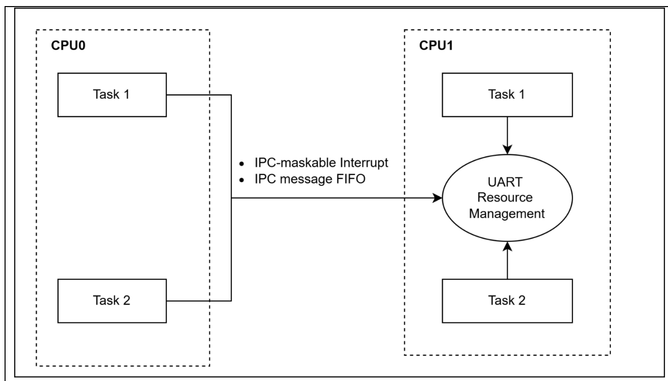
Figure 22. Example of Share Resource - UART diagram
