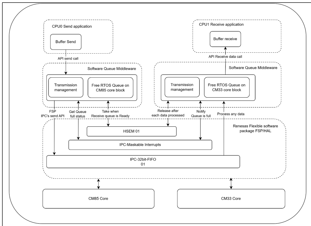
Figure 52. FreeRTOS-based Inter-core Messaging via IPC Hardware
