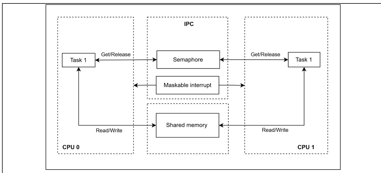
Figure 20. Example of Shared Memory Data Exchange and Synchronization
