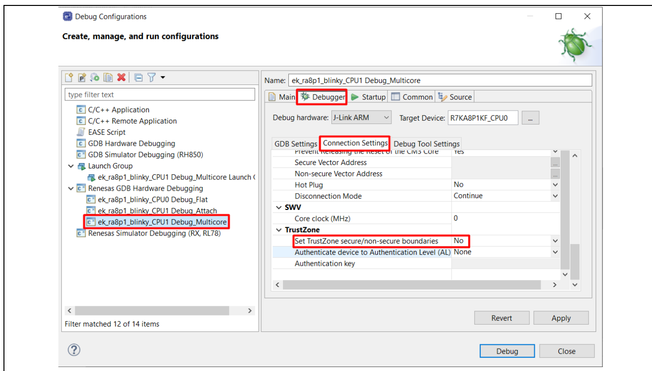
Figure 13. Example of Disabling TrustZone Boundary Setting
