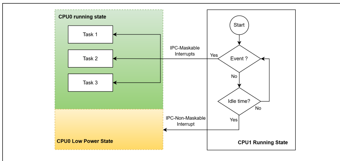
Figure 18. Example of CPU0 Notifications Using IPC Interrupts
