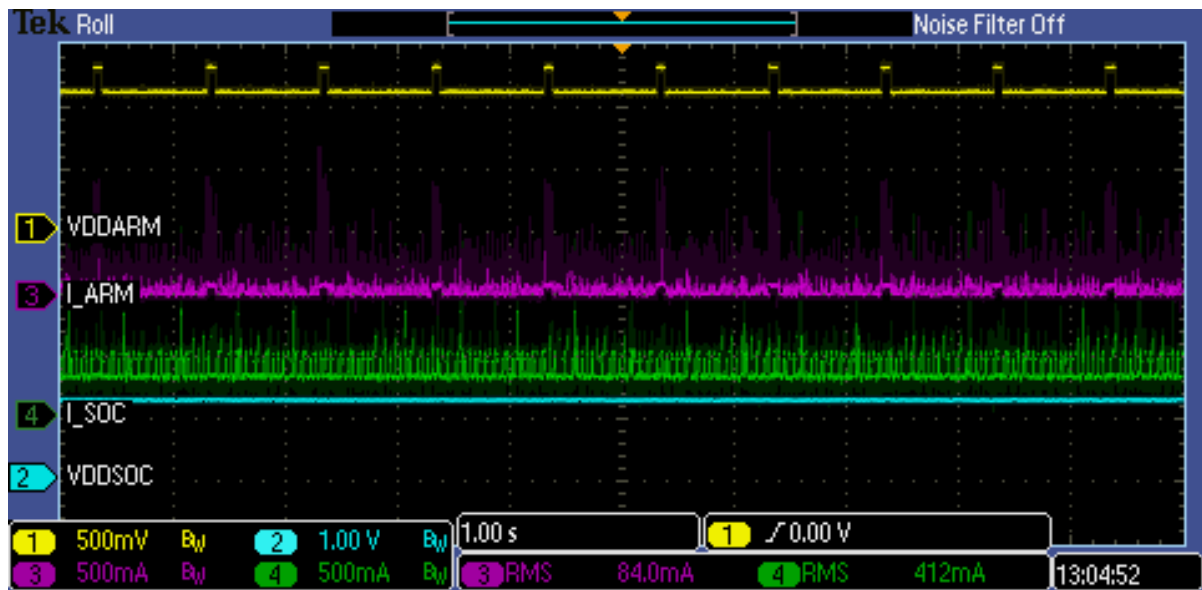
Figure 5: BYPASS MODE (Ido_active=OFF) at 1 GHz
