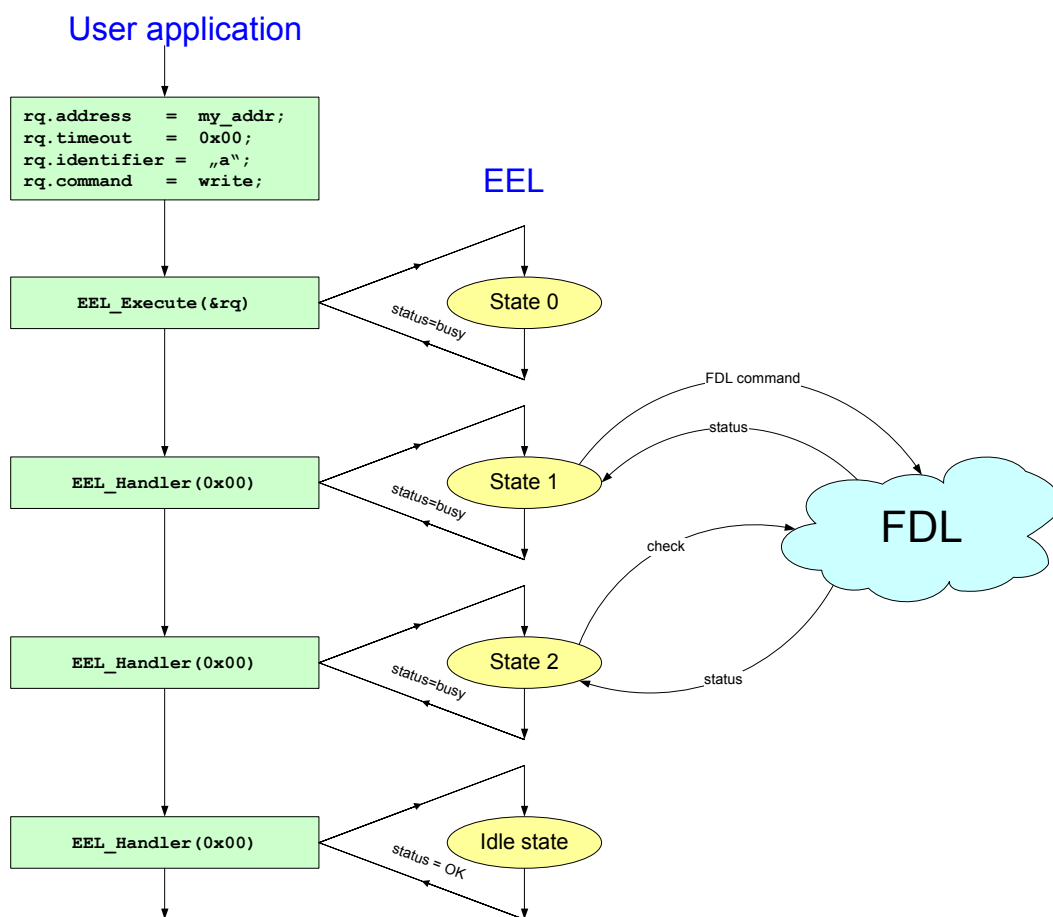
Figure 2-20 Schematic illustration of the polling operation mode
