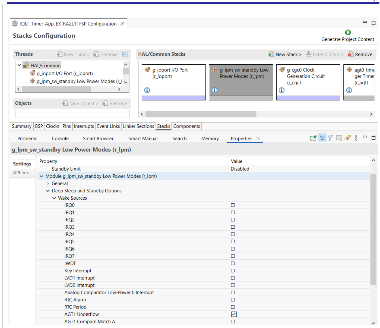
Figure 9. Software Standby Properties Configuration using the Properties Tab
