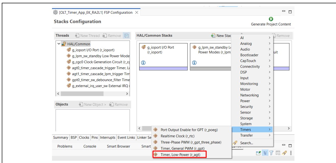
Figure 8. Adding r_agt Module to HAL/Common Thread
