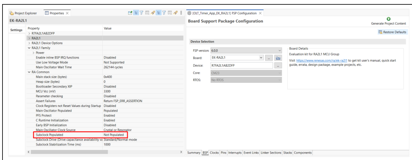
Figure 5. BSP Settings of the Operable Long Timer
