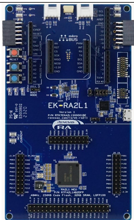
Figure 26. EK-RA2L1 Kit
