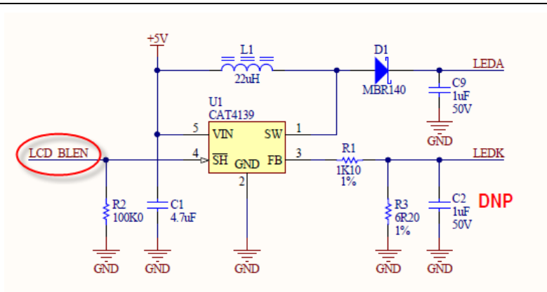
Figure 58. DK-S7G2 Backlight Control Circuit
