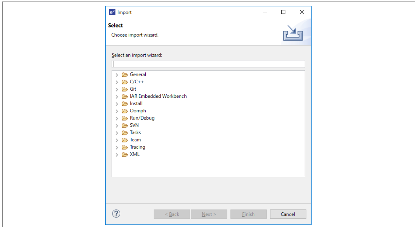
Figure 4 Import dialog
