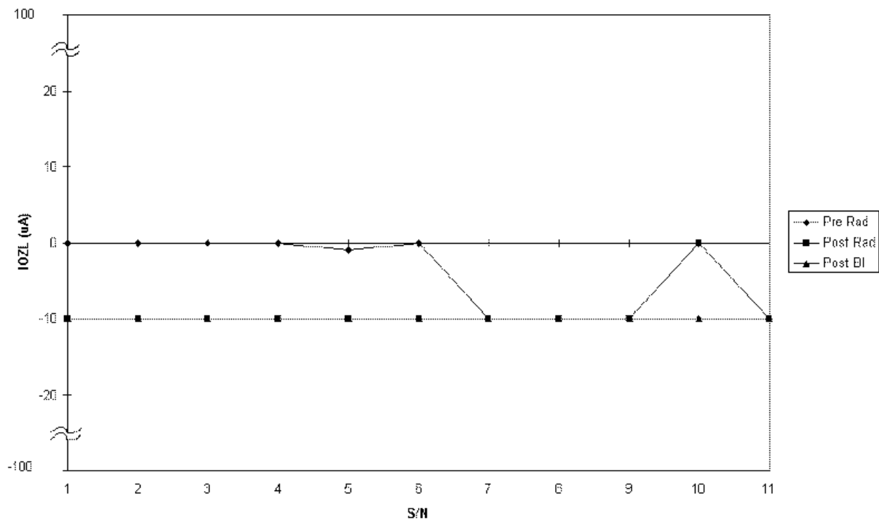
FIGURE 6. COMPARISON OF 64K PROM OUTPUT DRIVE CURRENT LOW ( I_{OZL} )
