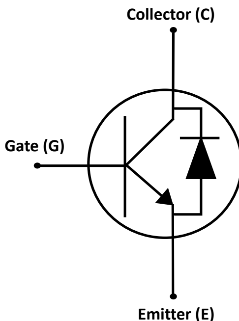
Figure 1-2 RC-IGBT symbol
