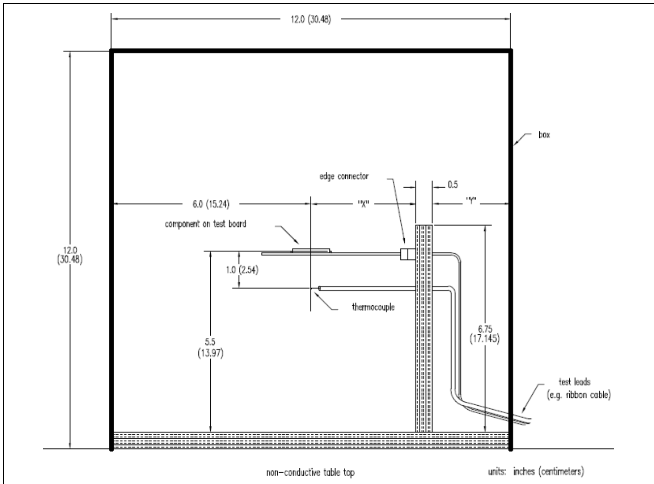
Figure 2-1 T_a measurement position (from the EIA/JEDEC 51-2 Standard)
