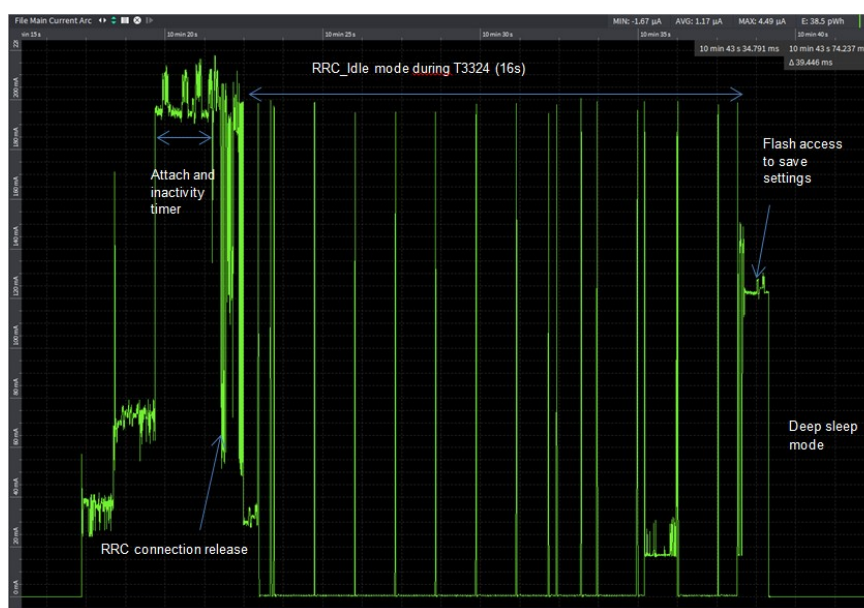
Figure 11. Tracking Area Update Power Consumption Graph
