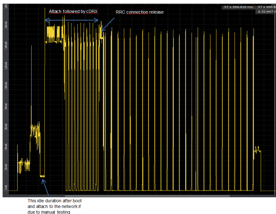
Figure 10. Power Graph in cDRX
