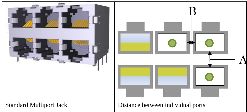
Figure 19-7: Multiport device (from [10])
