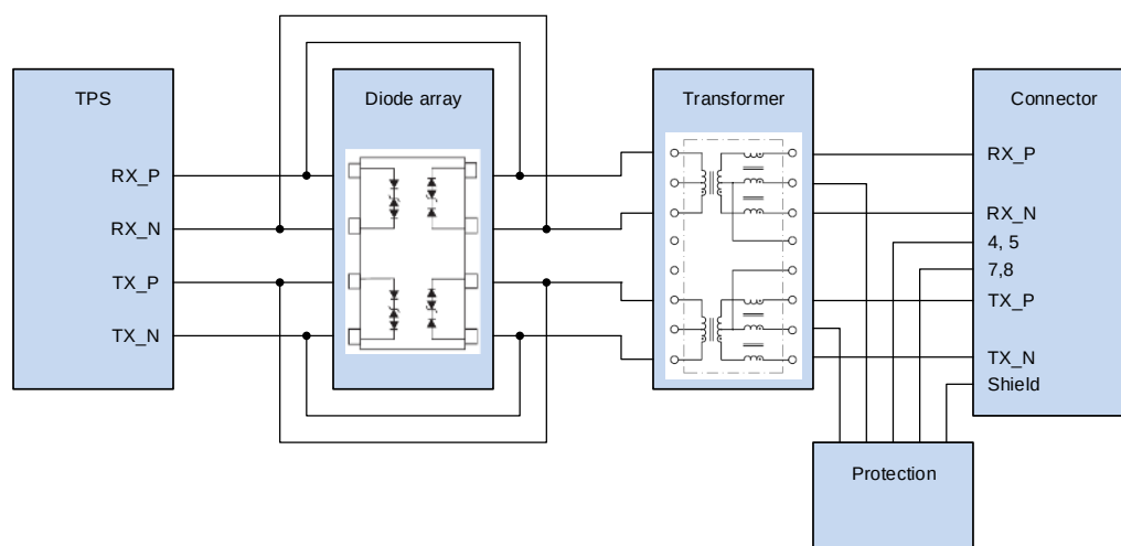
Figure 21-5: Typical ESD protection circuit
