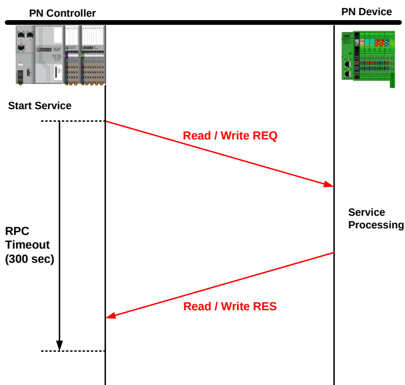
Figure 7-1: Record-Data Request / Response
