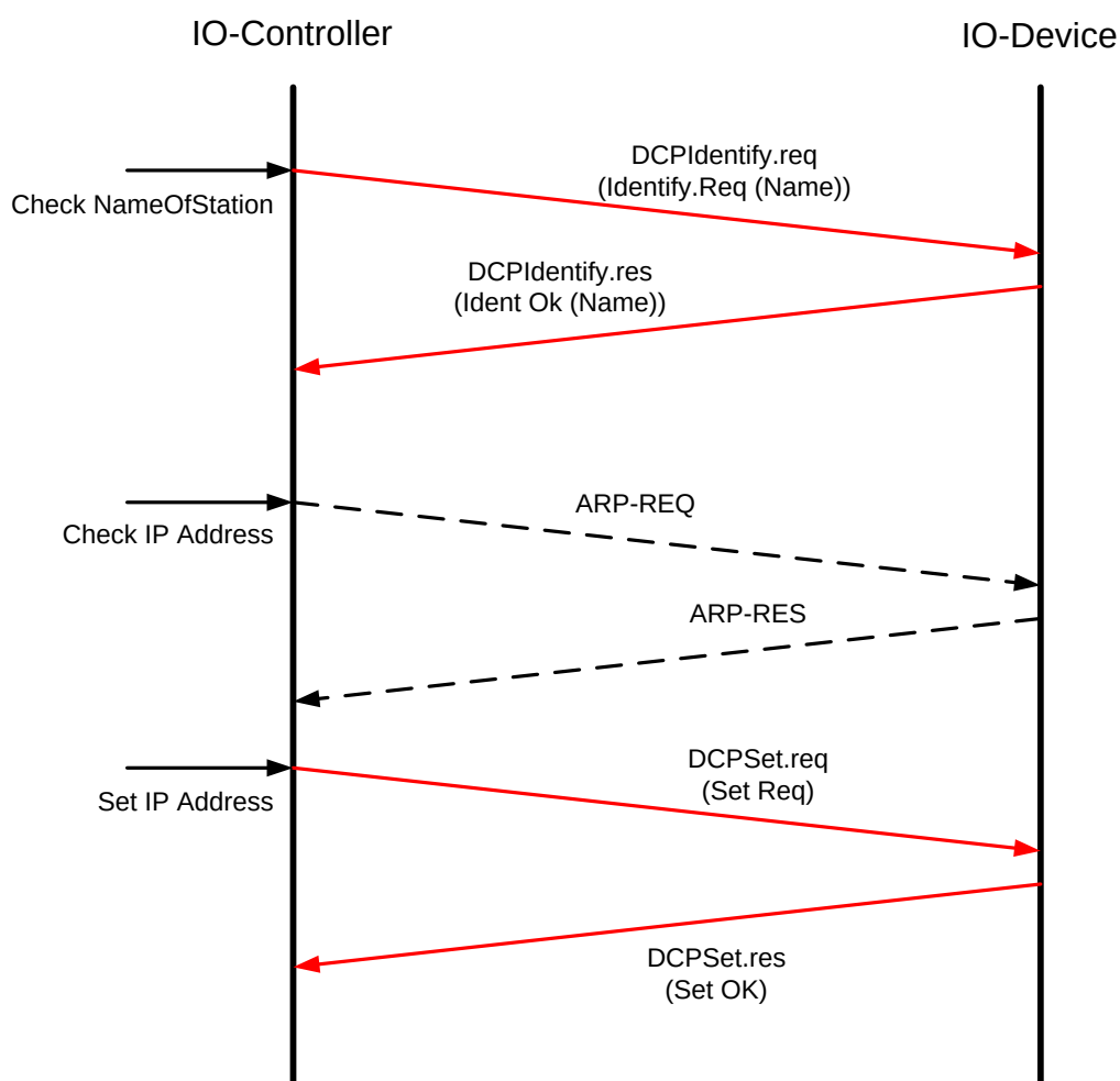
Figure 6-1: Identify Request
