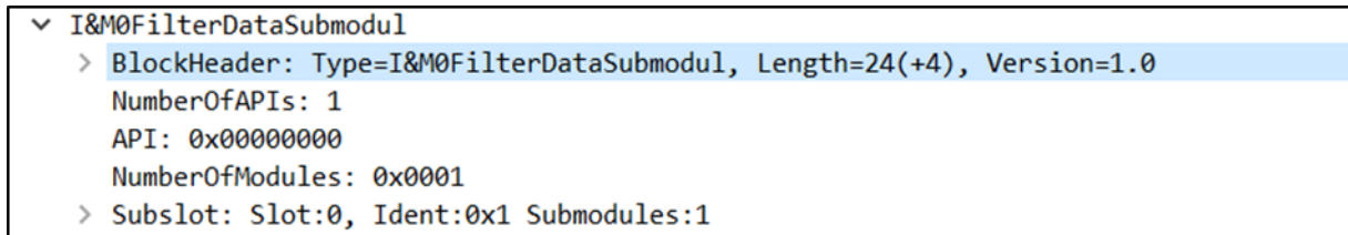
Figure 5-4: I&M0FilterDataSubmodul
