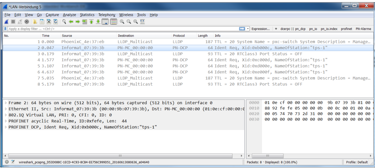
Figure 18-3: Searched station does not respond
