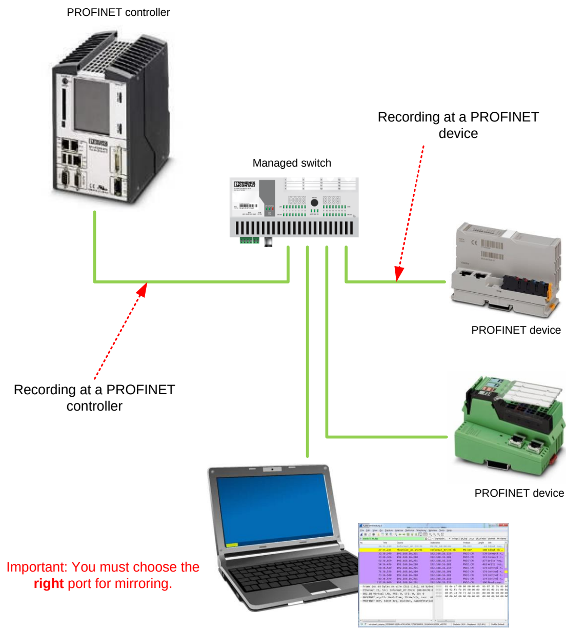
Figure 18-2: Measurements in a network
