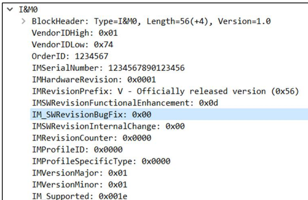
Figure 5-5: I&M0 data with IM_Supported structure
