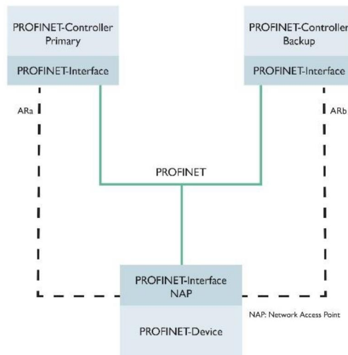
Figure 16-10: S2-Redundancy with the TPS-1
