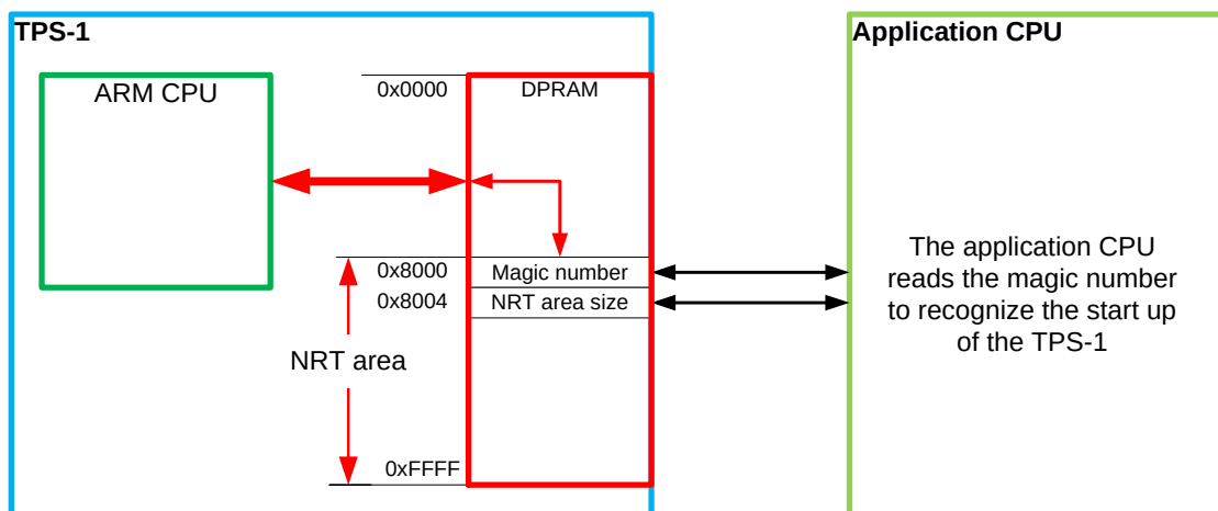
Figure 4-3: Start-synchronisation
