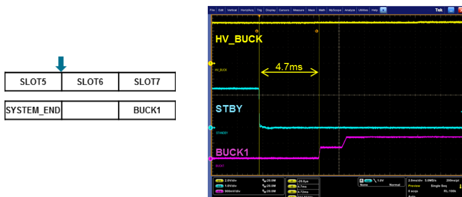
Figure 6: STBY Sequencing Control in Power-Down Mode
