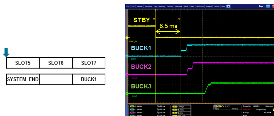
Figure 7: STBY Sequencing Control
