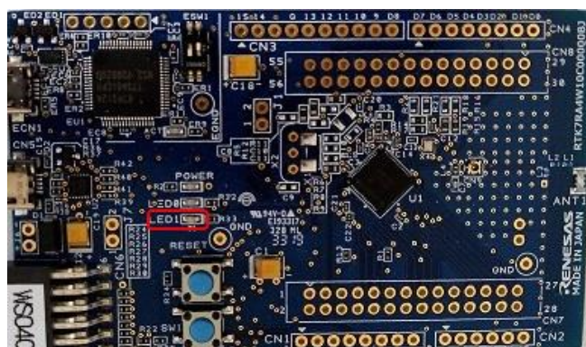
Figure 4-12 Position of the LED that Blinks on Board A(EK Board for RA4W1)
