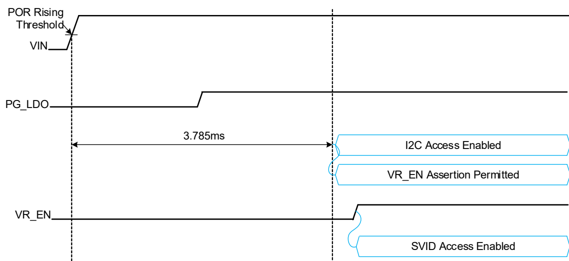
Figure 2. Startup Timing Diagram
