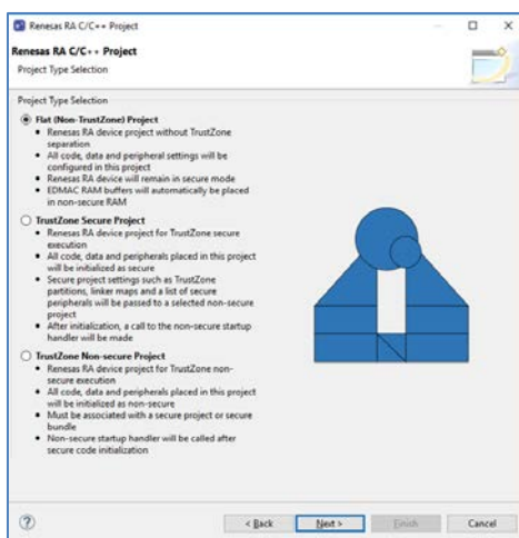
Figure 6. Flat Project
