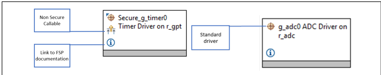
Figure 27. Configurator Icons
