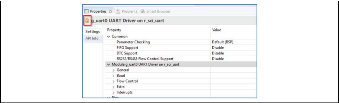
Figure 14. Locked Resources
