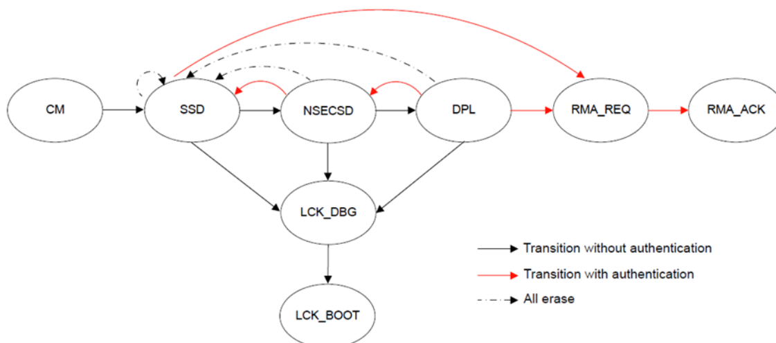
Figure 19. Lifecycle Stages
