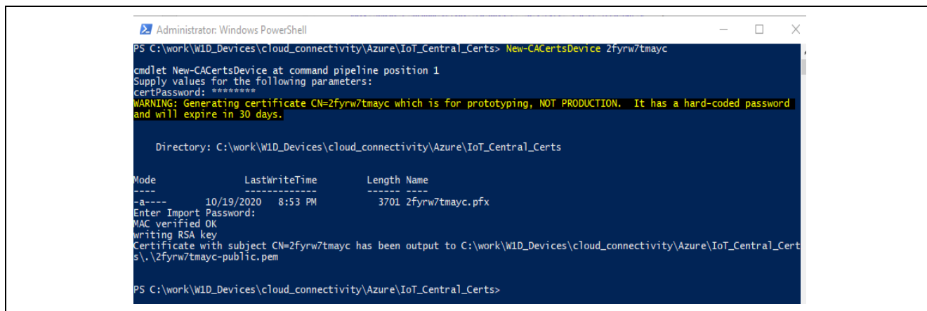
Figure 51. Creating Leaf Certificate
