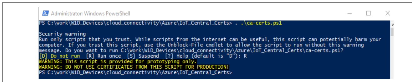
Figure 36. Executing Script with ' .. \ca-certs.ps1 '
