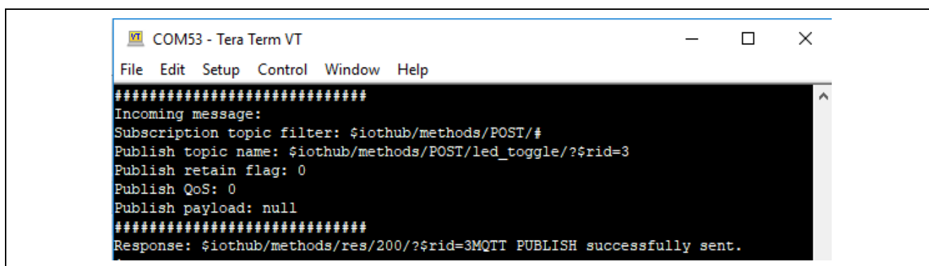
Figure 72. Tera Term Console Display
