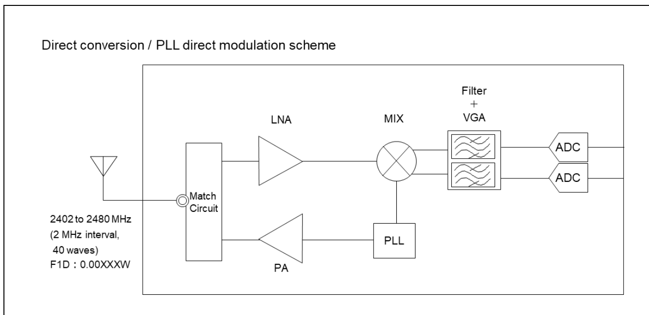
Figure 2-2. Block diagram of radio equipment — RF transceiver details (Example)
