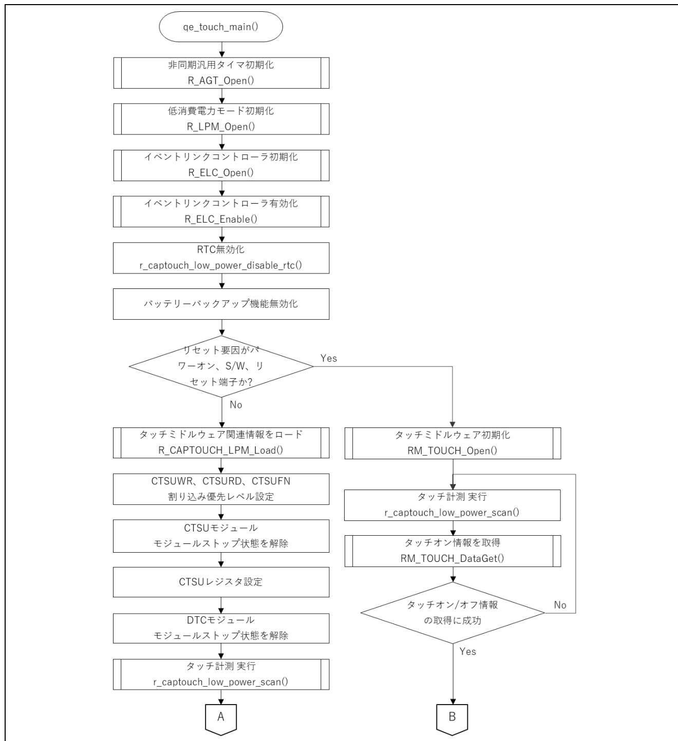
図 4-1 qe_touch_main () (1/2)
