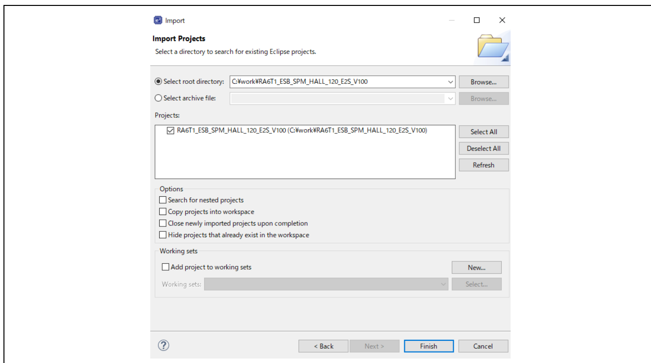
Figure 4-3 Project Import
