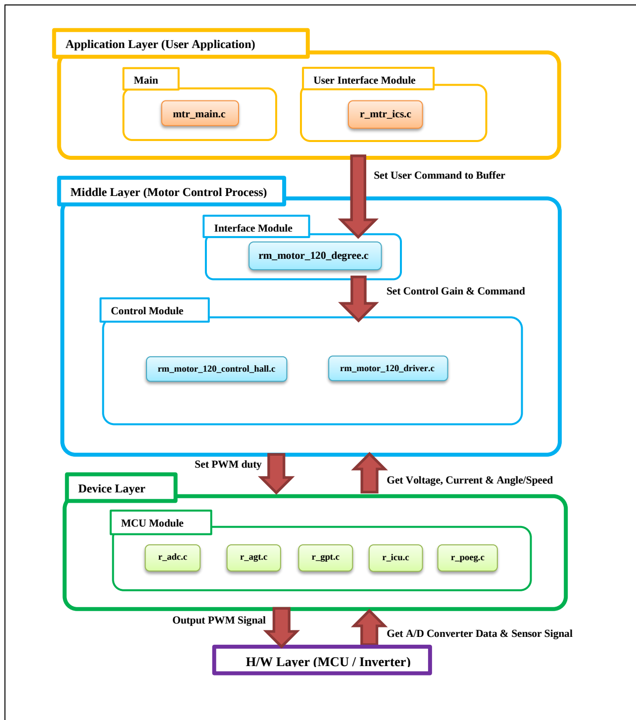
Figure 2-9 Module Configuration
