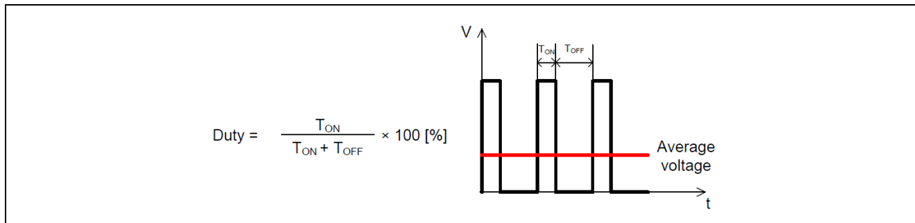
Figure 3-2 PWM Control
