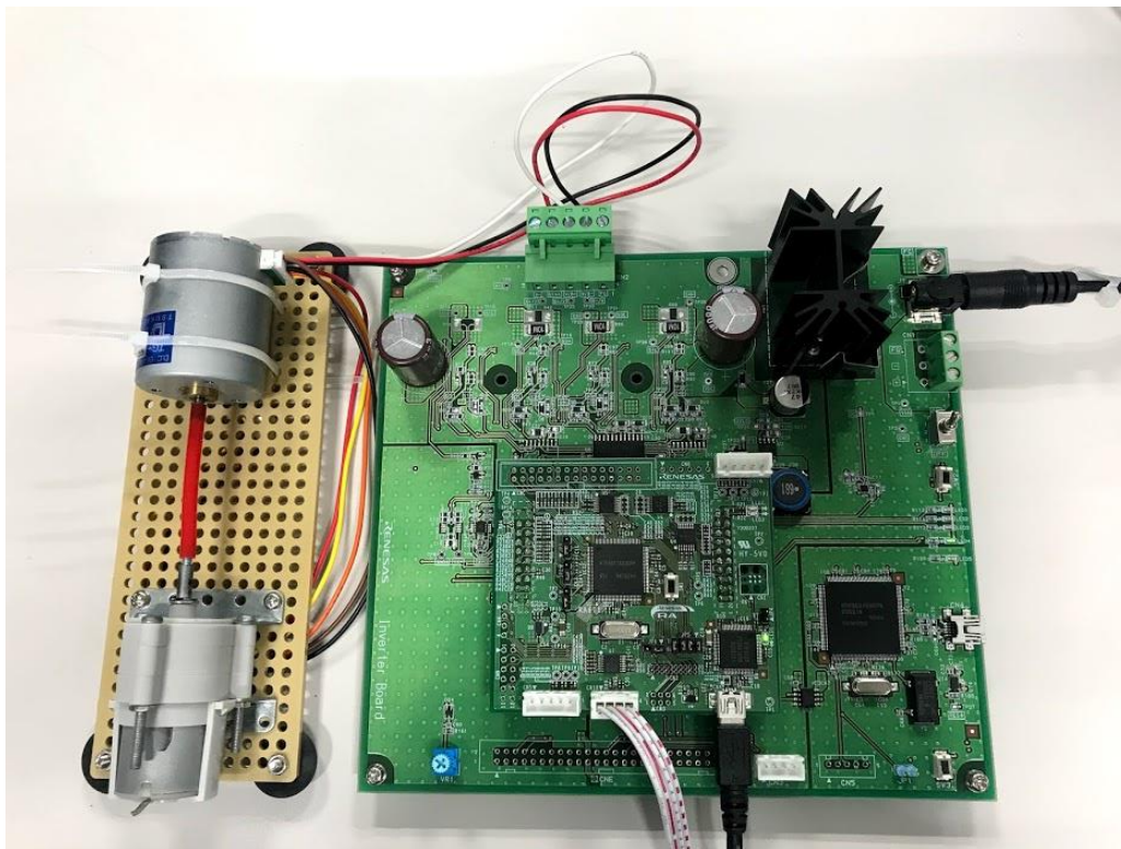
Figure 2-1. RA6T1 RSK with Motor Bench for demonstration
