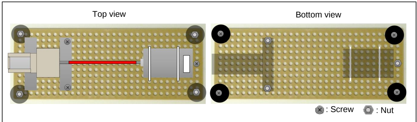
Figure 2-3. Simple motor bench - Parts location
