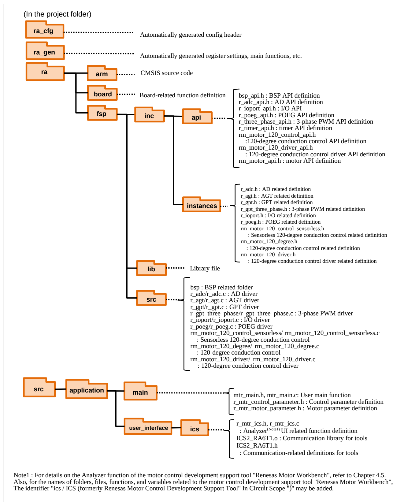
Figure 2-7 Folder and file structure
