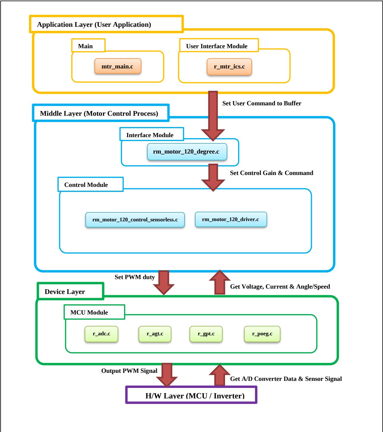
Figure 2-8 Module Configuration
