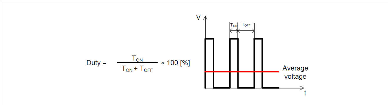
Figure 3-2 PWM Control
