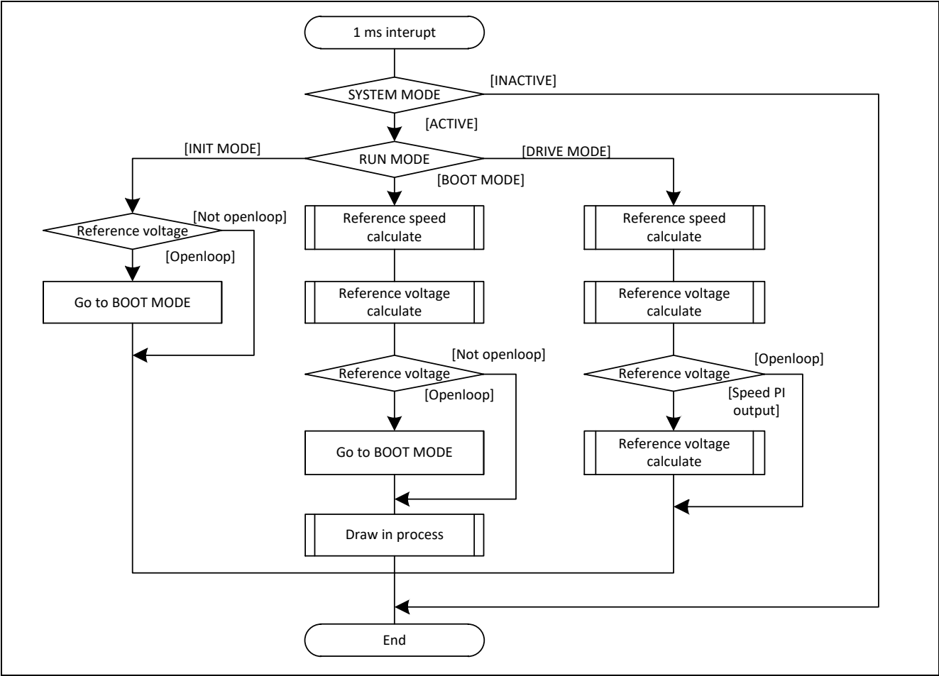
Figure 3-12 1 [ms] Periodic Interrupt Handling
