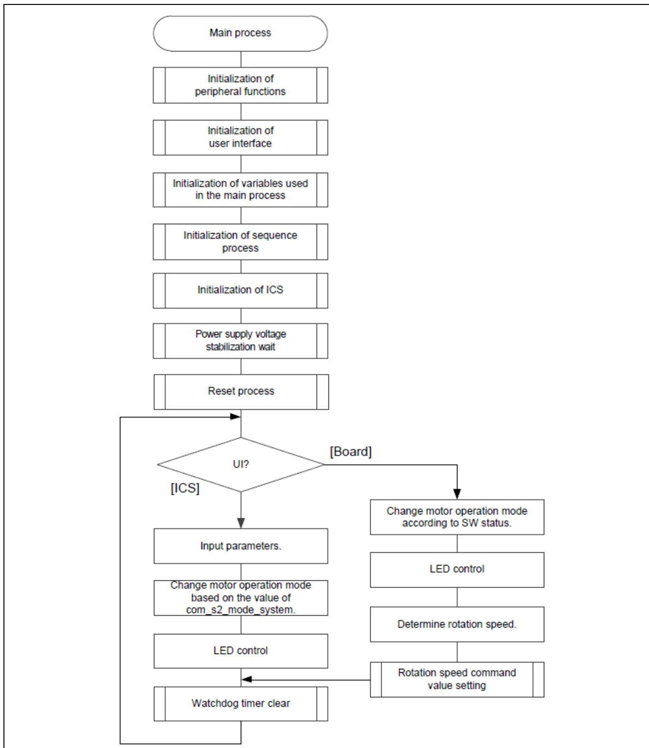
Figure 3-10 Main Process Flowchart
