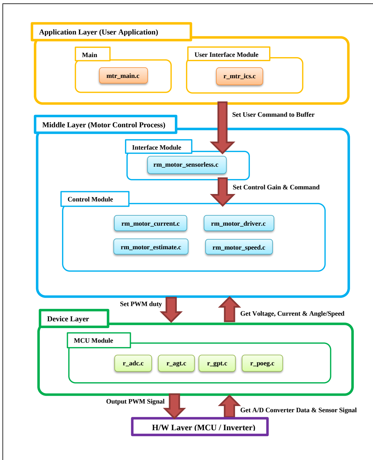
Figure 2-8 Module Configuration
