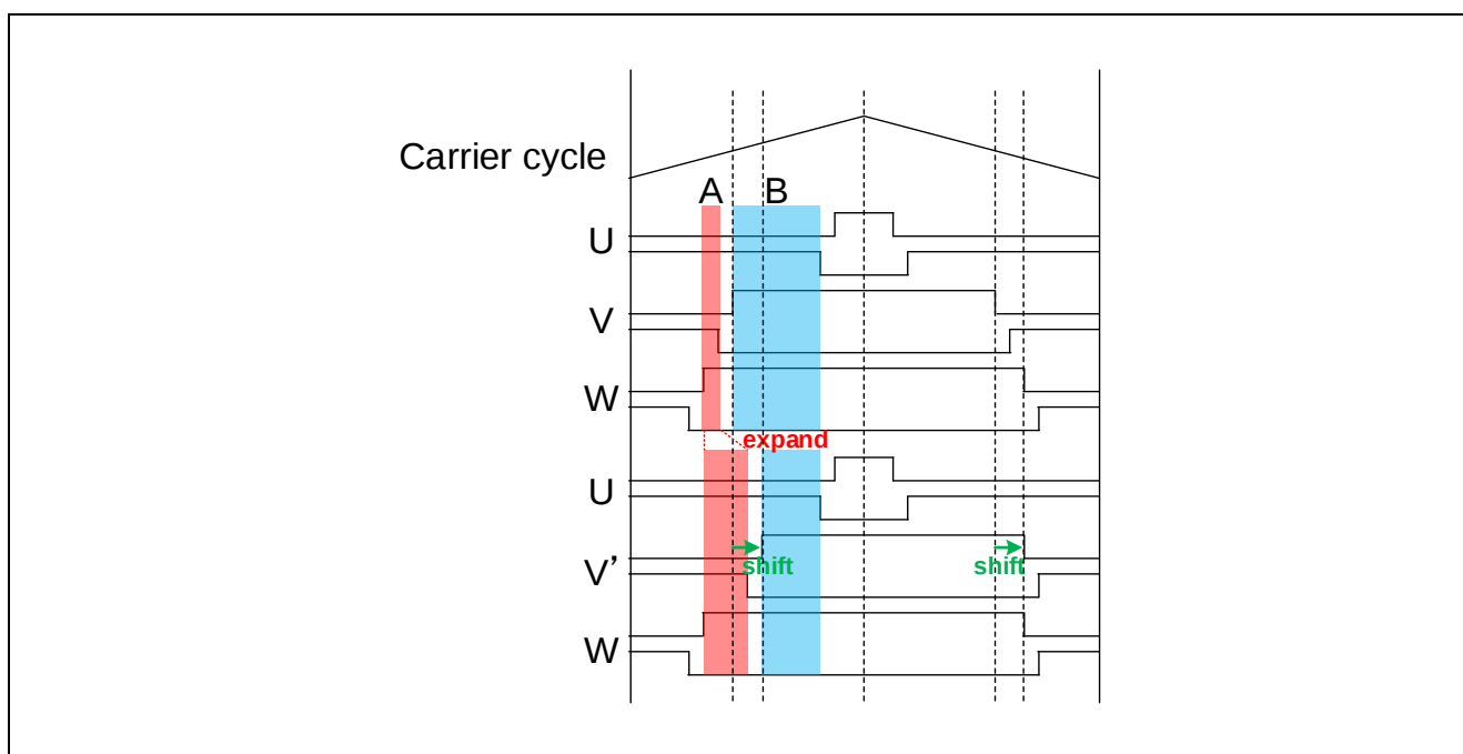
Figure 3-7 Duty adjustment
