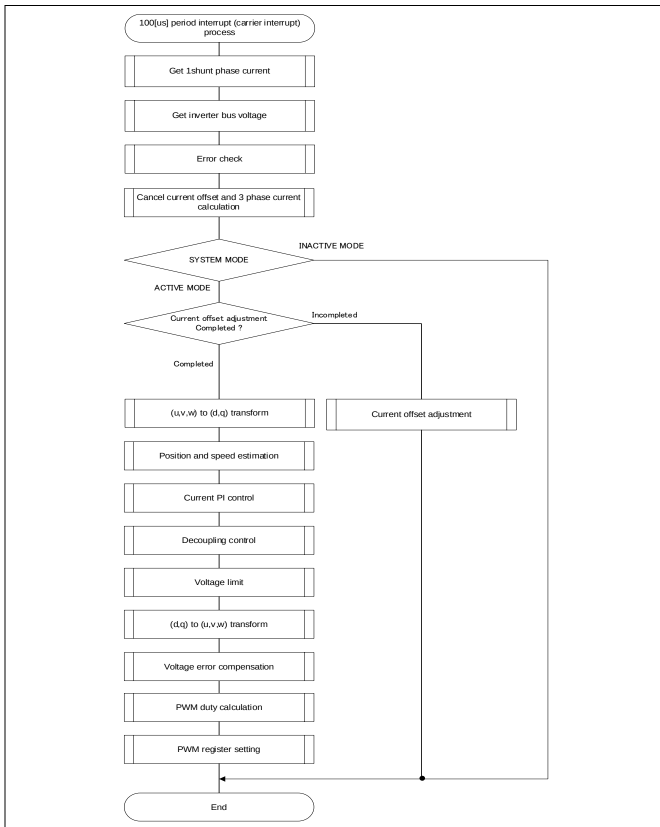
Figure 3-17 100[μs] Period Interrupt (Carrier Interrupt) Process Flowchart
