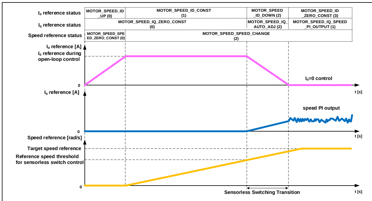
Figure 3-4 Startup Control of Sensorless Vector Control Software
