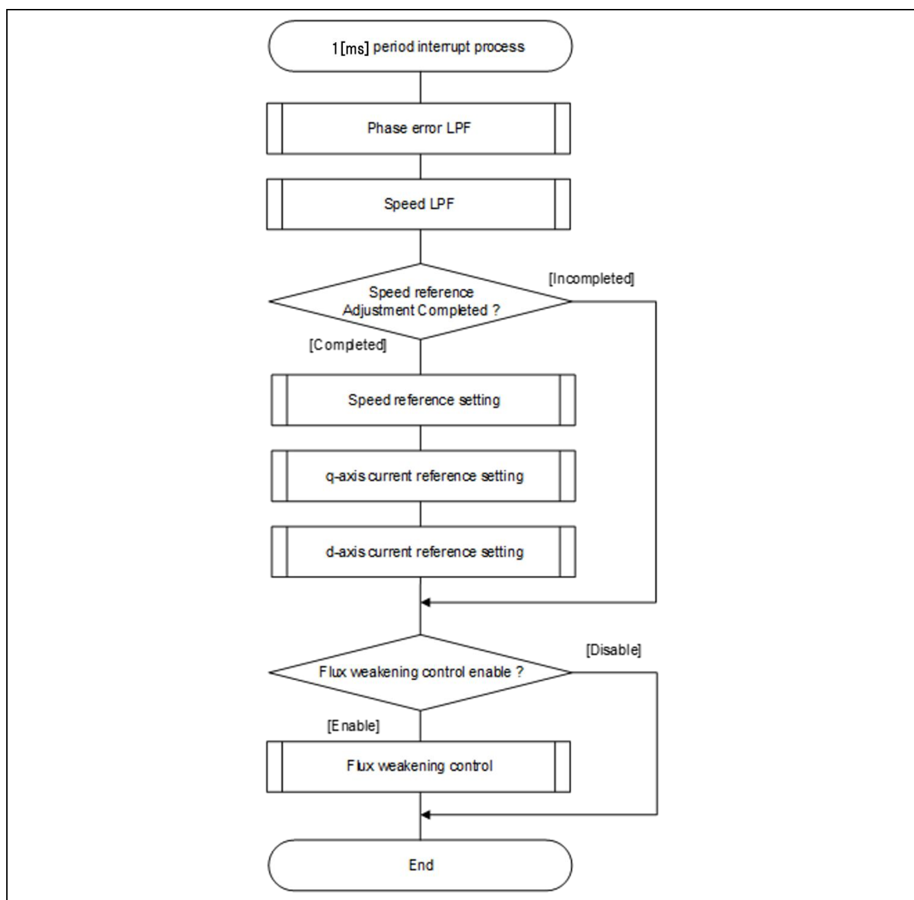
Figure 3-18 1 [ms] Period Interrupt Process Flowchart
