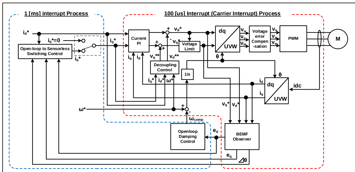
Figure 3-9 Block Diagram of Sensorless Vector Control (Openloop Control)
