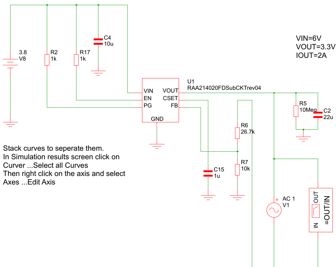
Figure 2. Gain Phase Test Setup with Sub-Circuit RAA214020FDSBCKTrev04
