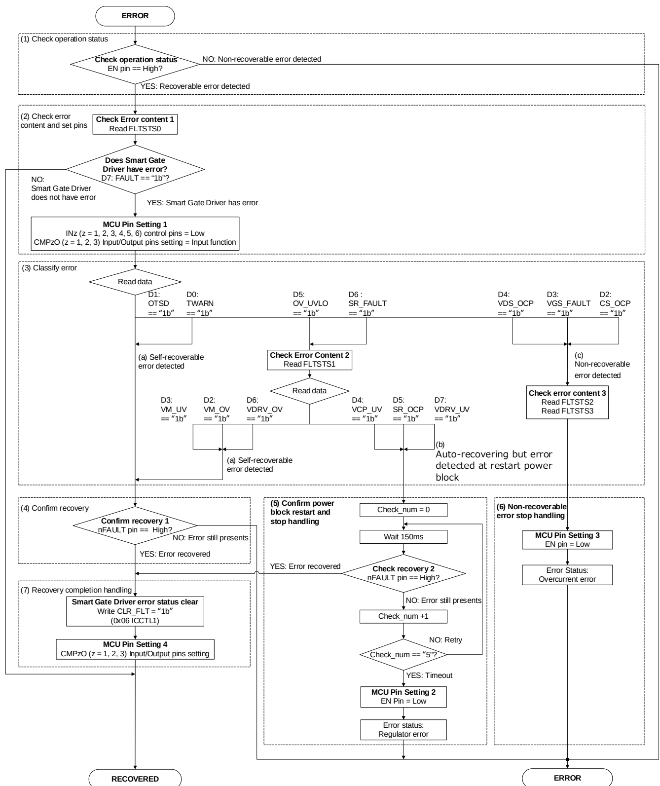
Figure 3-2 Smart Gate Driver Error Recovery Sequence Example
