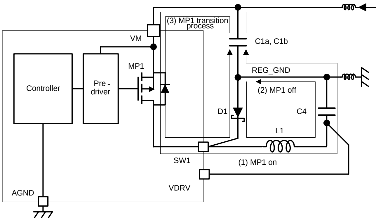
Figure 4-8 Current Path of the Buck Switching Regulator
