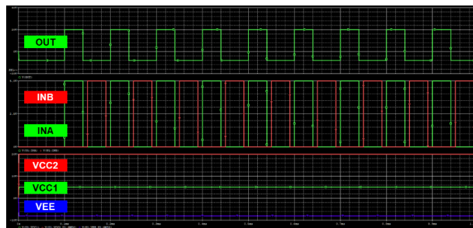
Figure.8 Simulation result (Basic characteristics)
