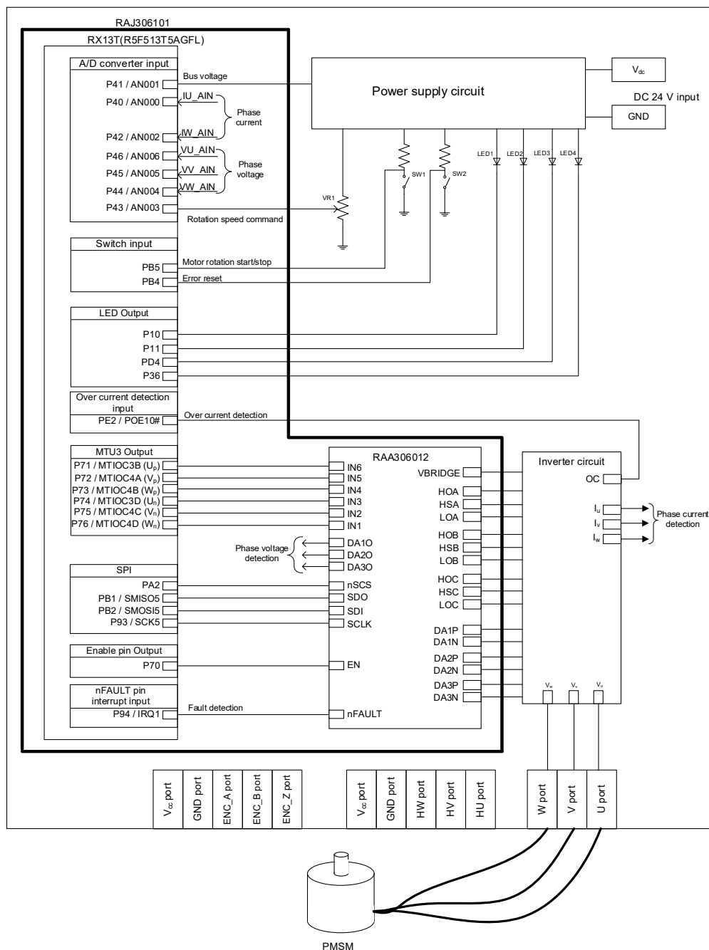
Figure 2-1 Hardware Configuration Diagram
