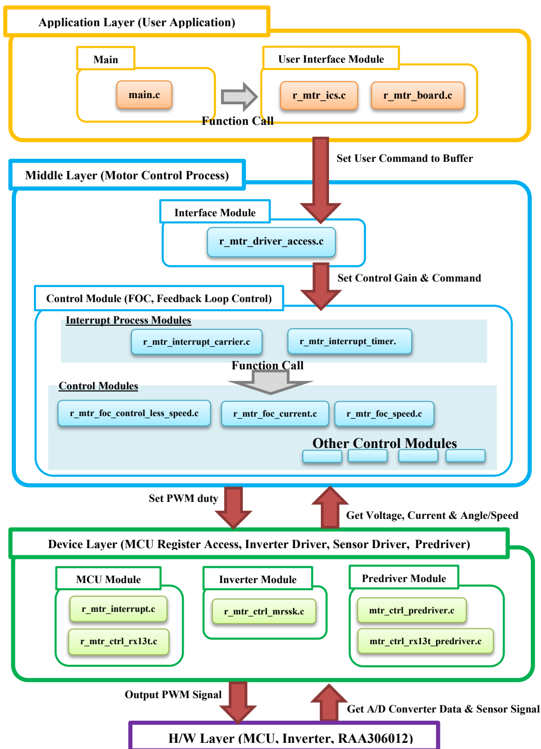
Figure 2-3 Module Configuration
