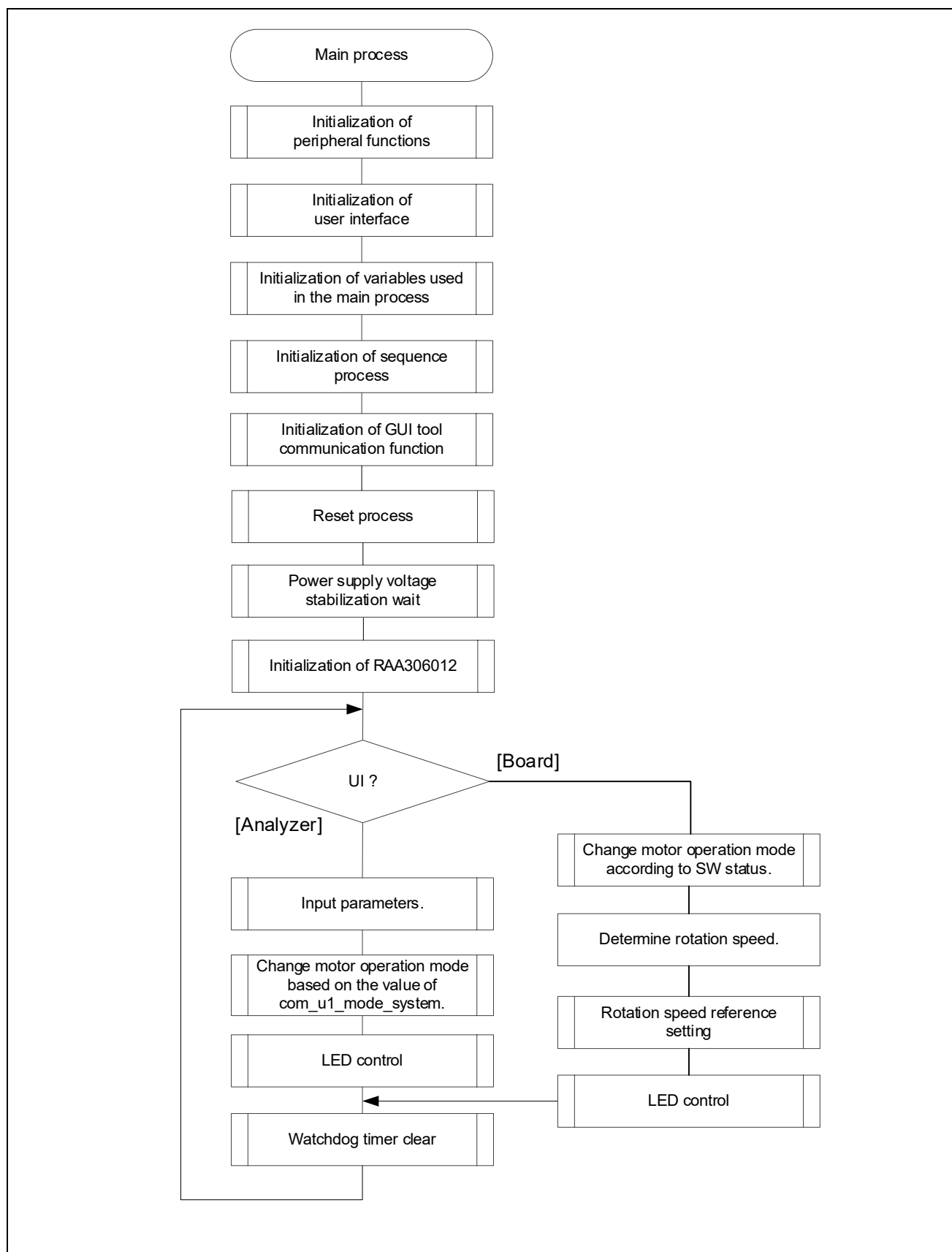
Figure 3-7 Main Process Flowchart
