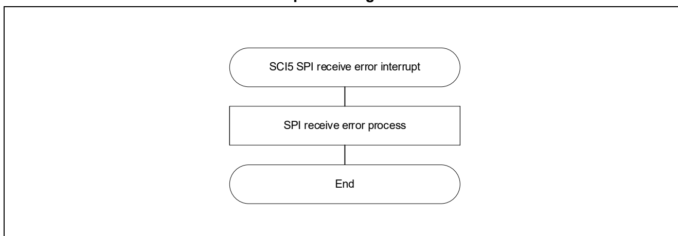
Figure 3-14 SCI5 SPI receive error interrupt Handling
