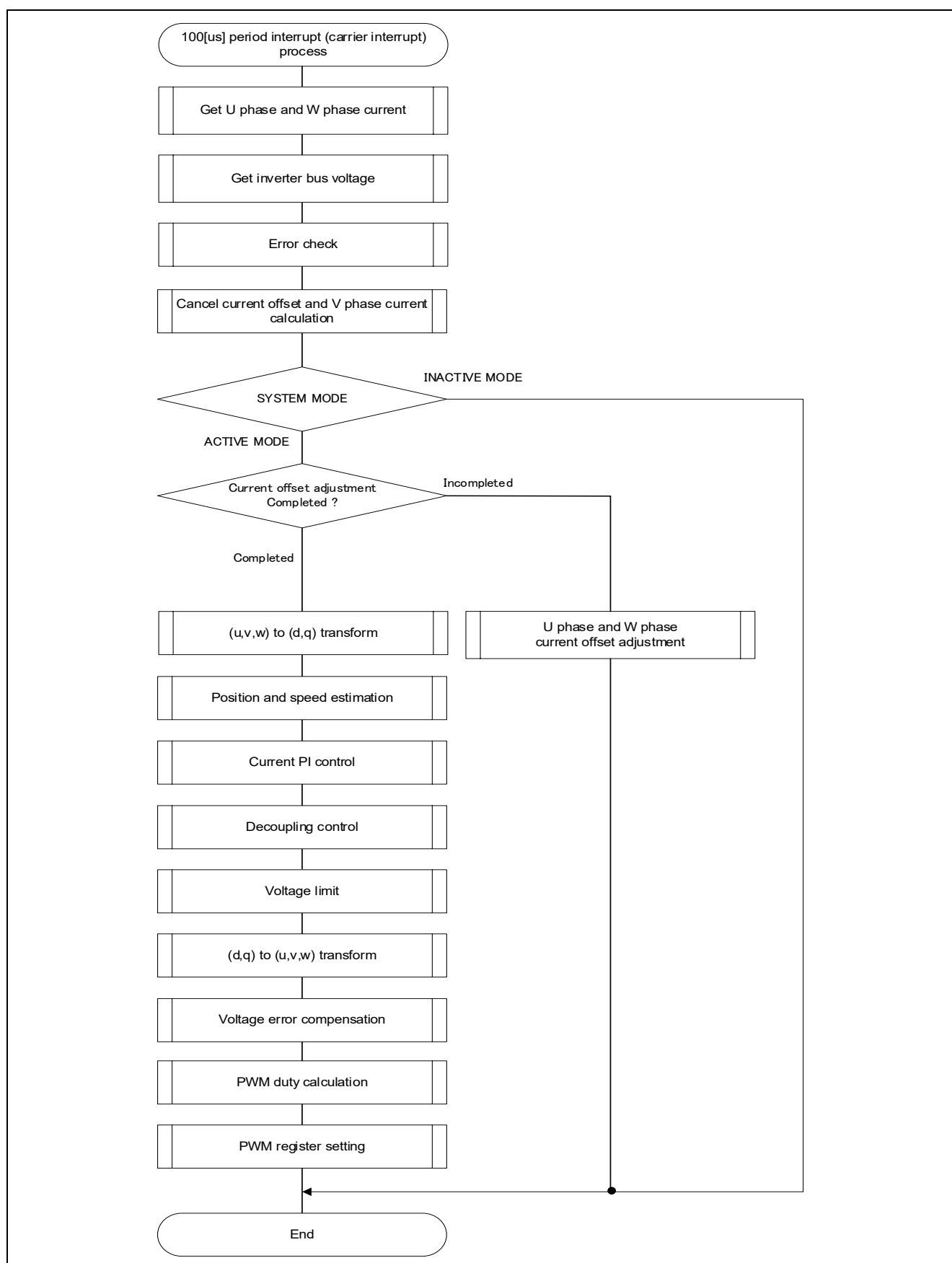
Figure 3-8 100[μs] Period Interrupt (Carrier Interrupt) Process Flowchart
