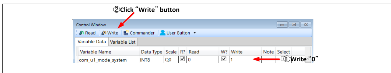
Figure 4-3 Procedure - Stop the Motor
