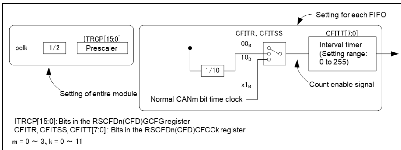
Figure 2-4 Block Diagram of the Interval Timer
