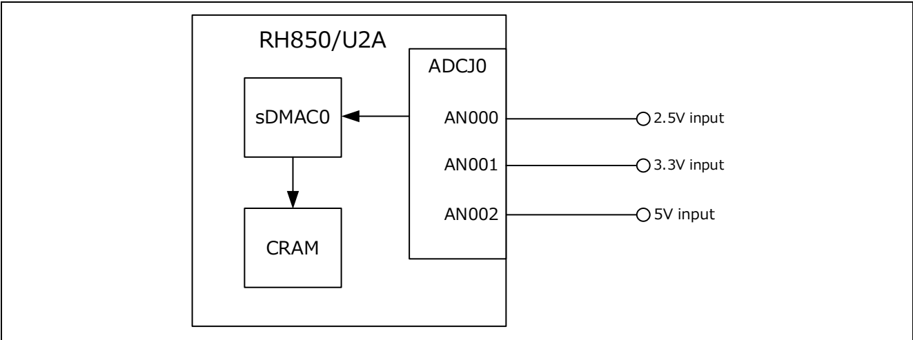
Figure 3.8.2 System Configuration
