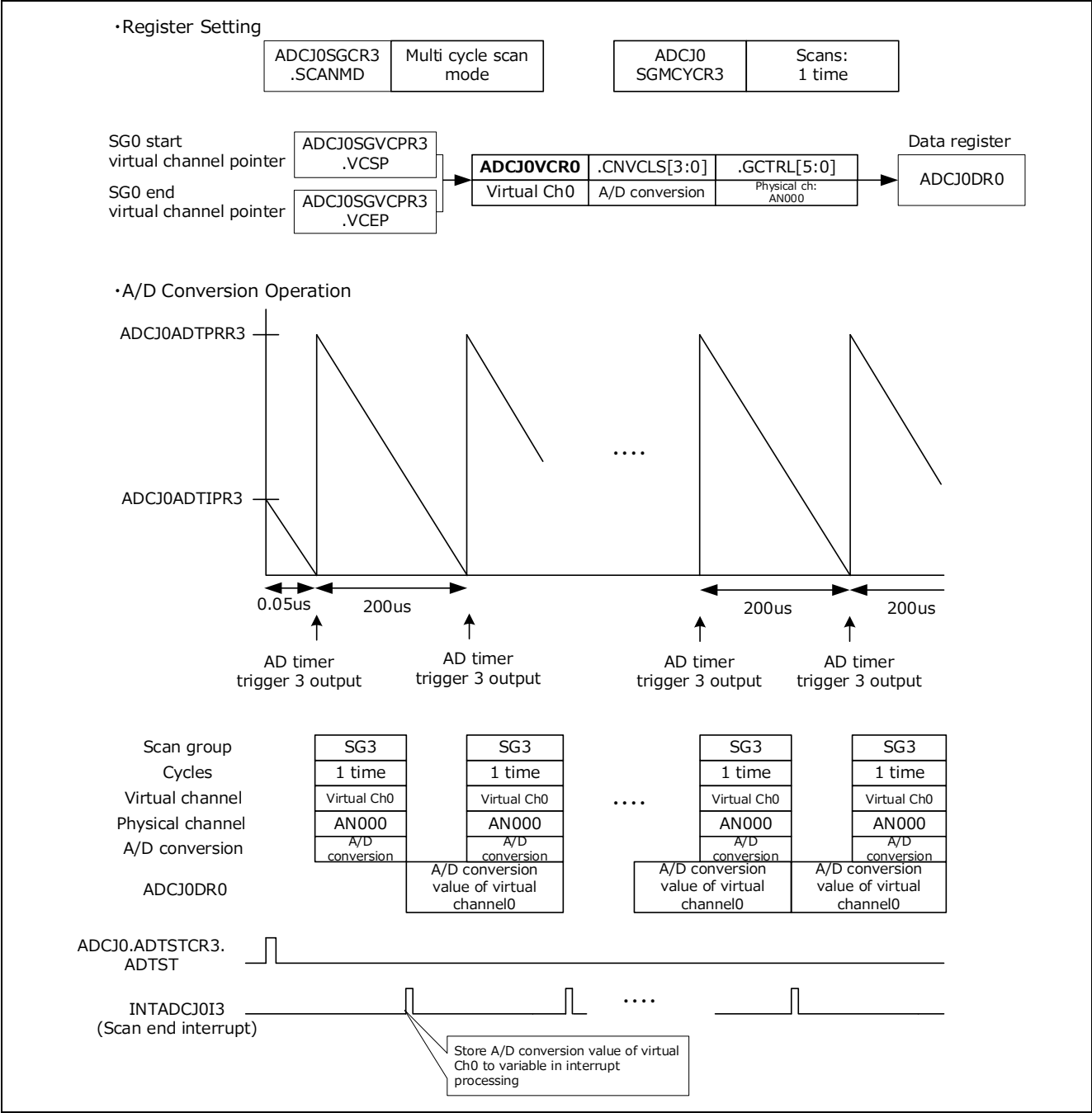
Figure 3-3 A/D timer Operation Value
