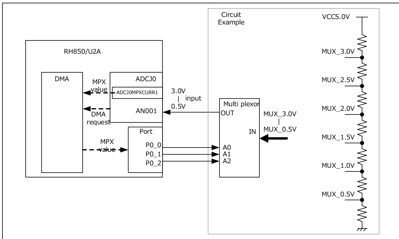
Figure 3-10 System Configuration
