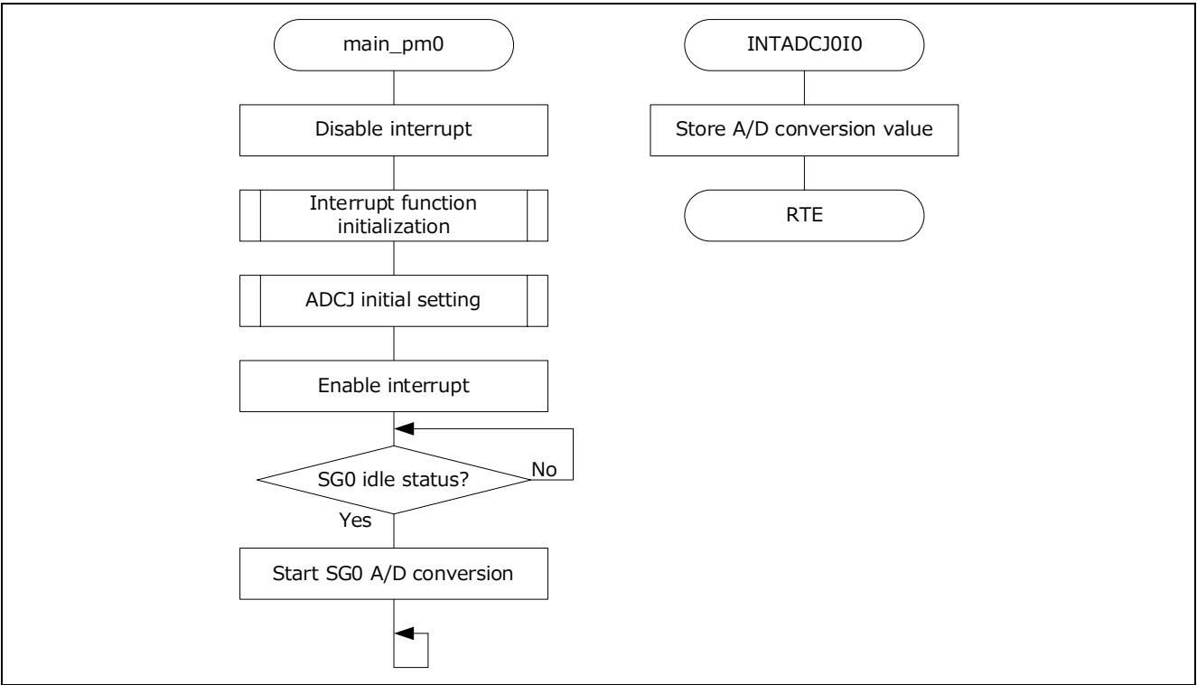
Figure 3.1.4 Flowchart
