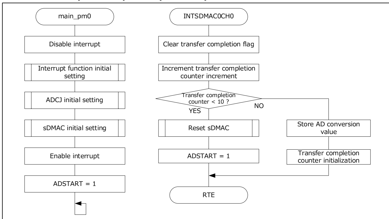
Figure 3.7.5 Flowchart
