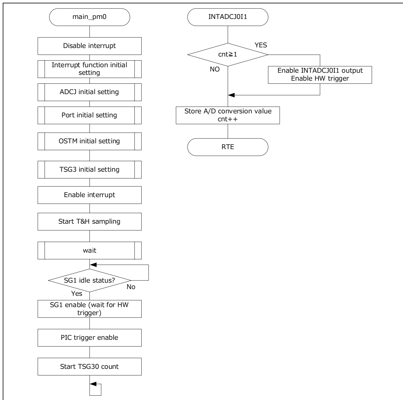
Figure 3-16 Flow Chart
