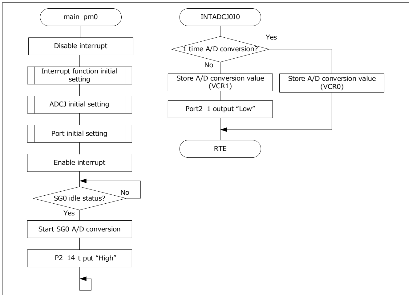
Figure 3.9.4 Flowchart
