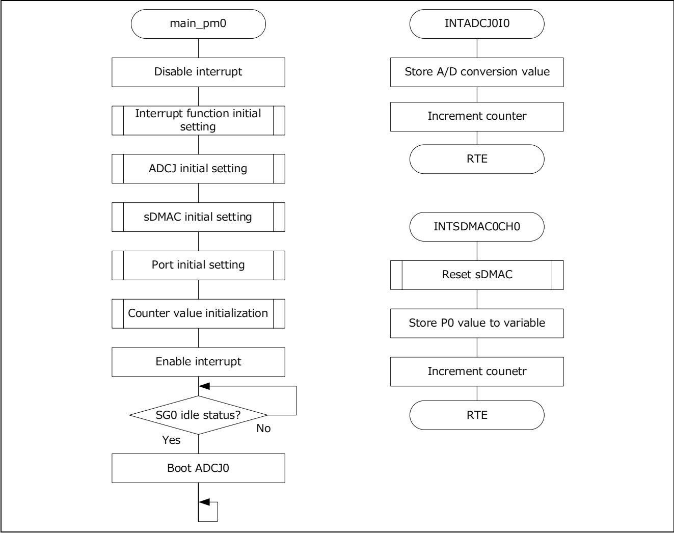
Figure 3-12 Flowchart
