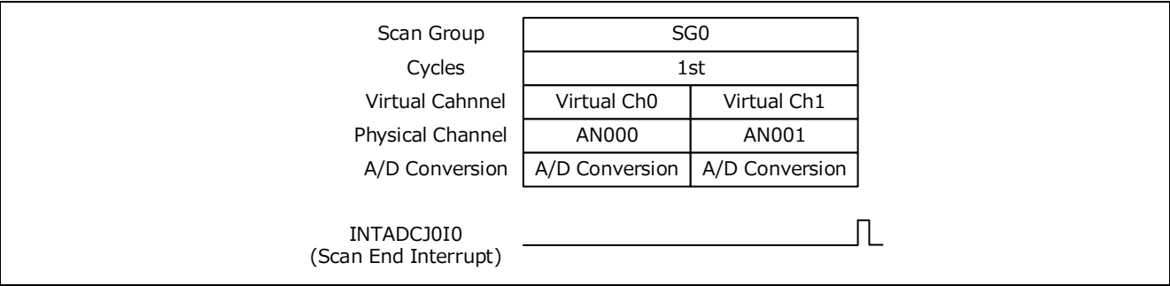
Figure 3.1.1 Normal A/D Conversion (Multicycle scan Operation)
