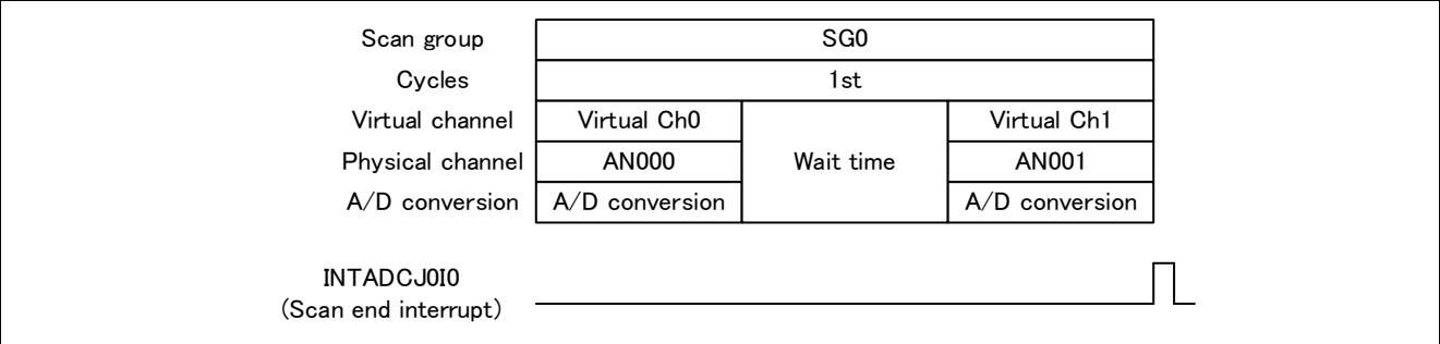
Figure 3.9.1 Normal A/D Conversion (Multicycle scan) Operation
