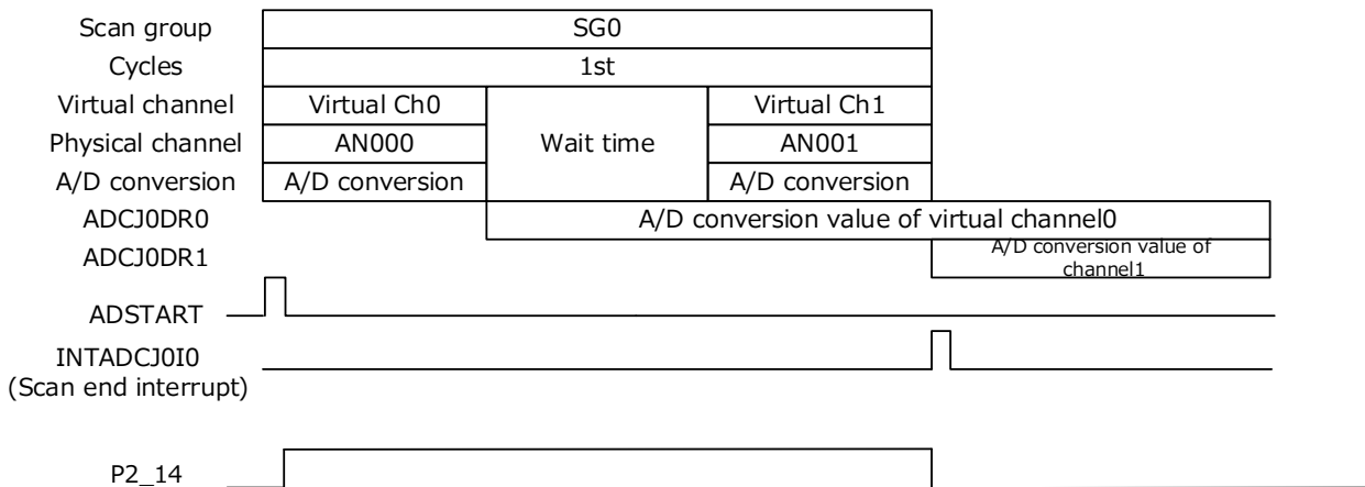
Figure 3.9.3 Normal A/D Conversion (Wait Insert between Virtual Channels) Operation Example
