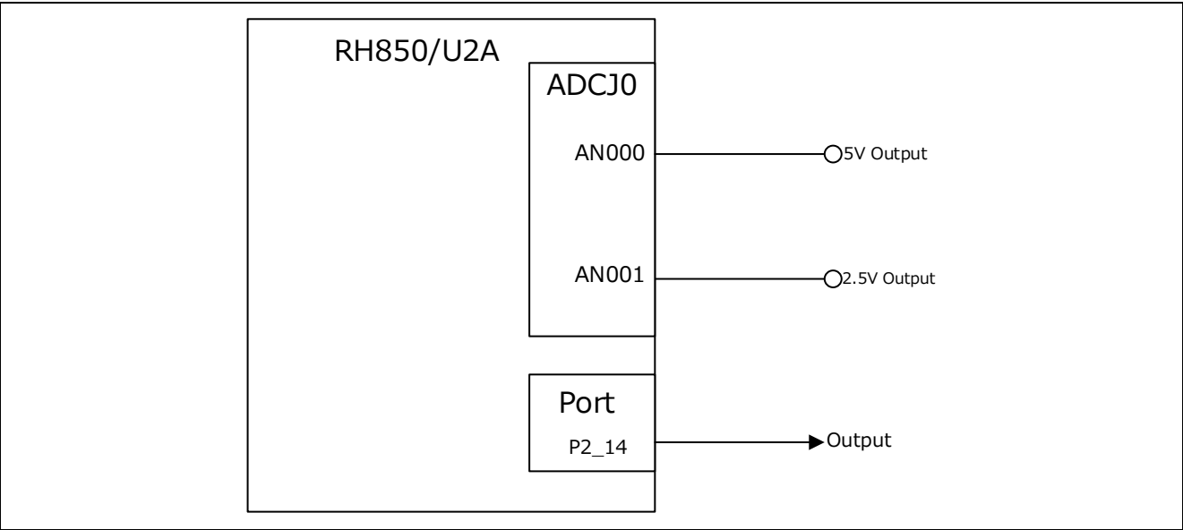
Figure 3.9.2 System Configuration
