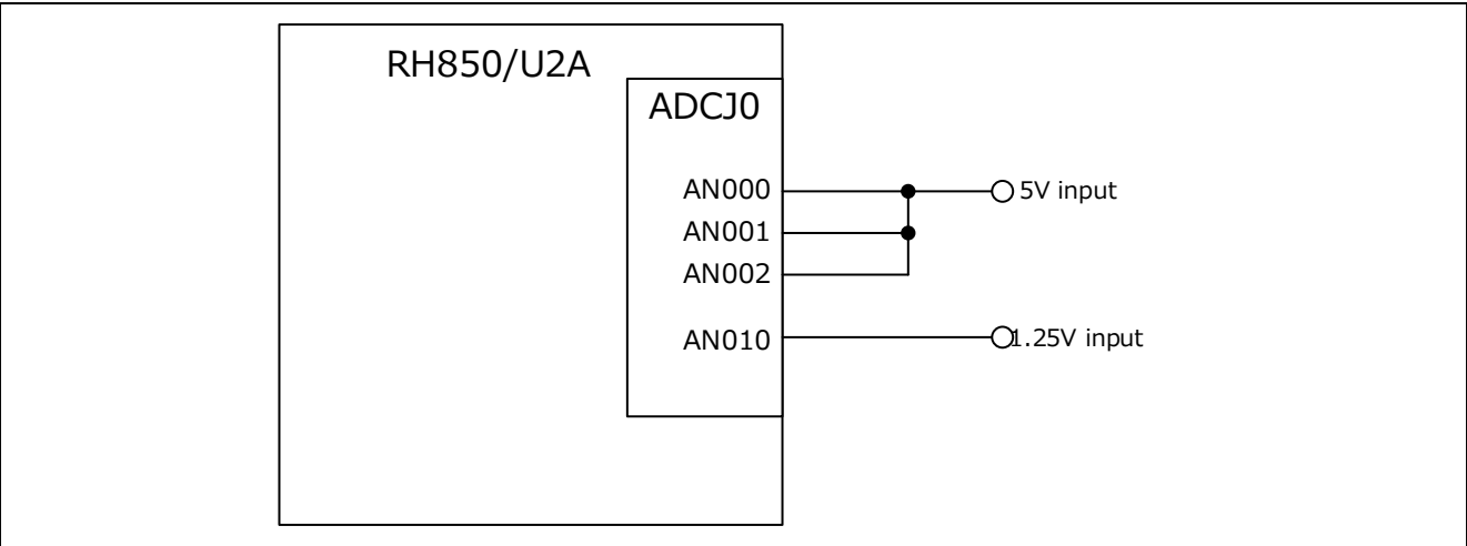
Figure 3.2.2 System Configuration
