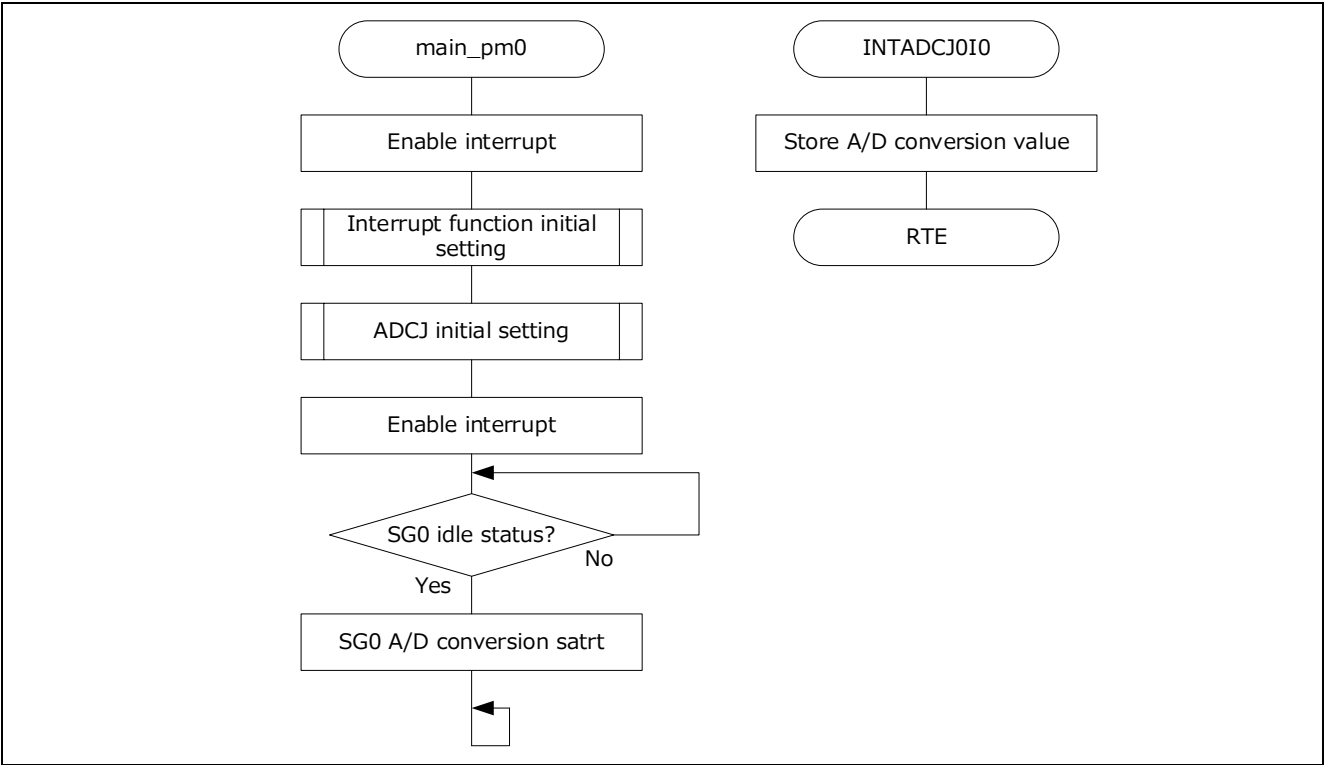
Figure 3-8 Flowchart
