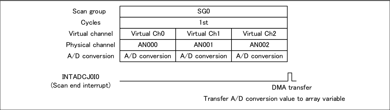
Figure 3.7.1 Operation Example using DMA Transfer
