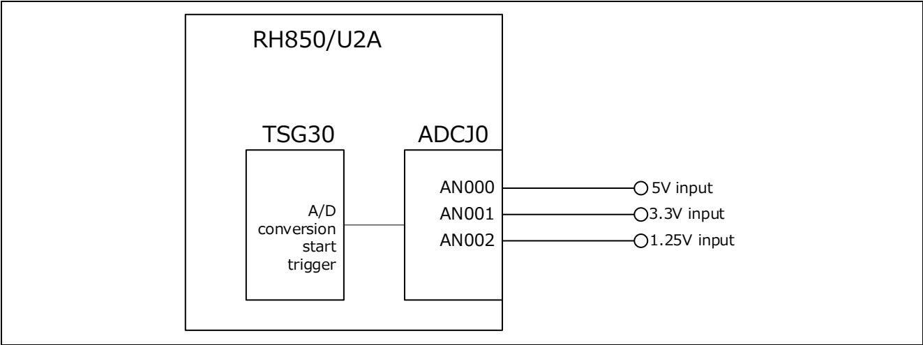
Figure 3-14 System Configuration
