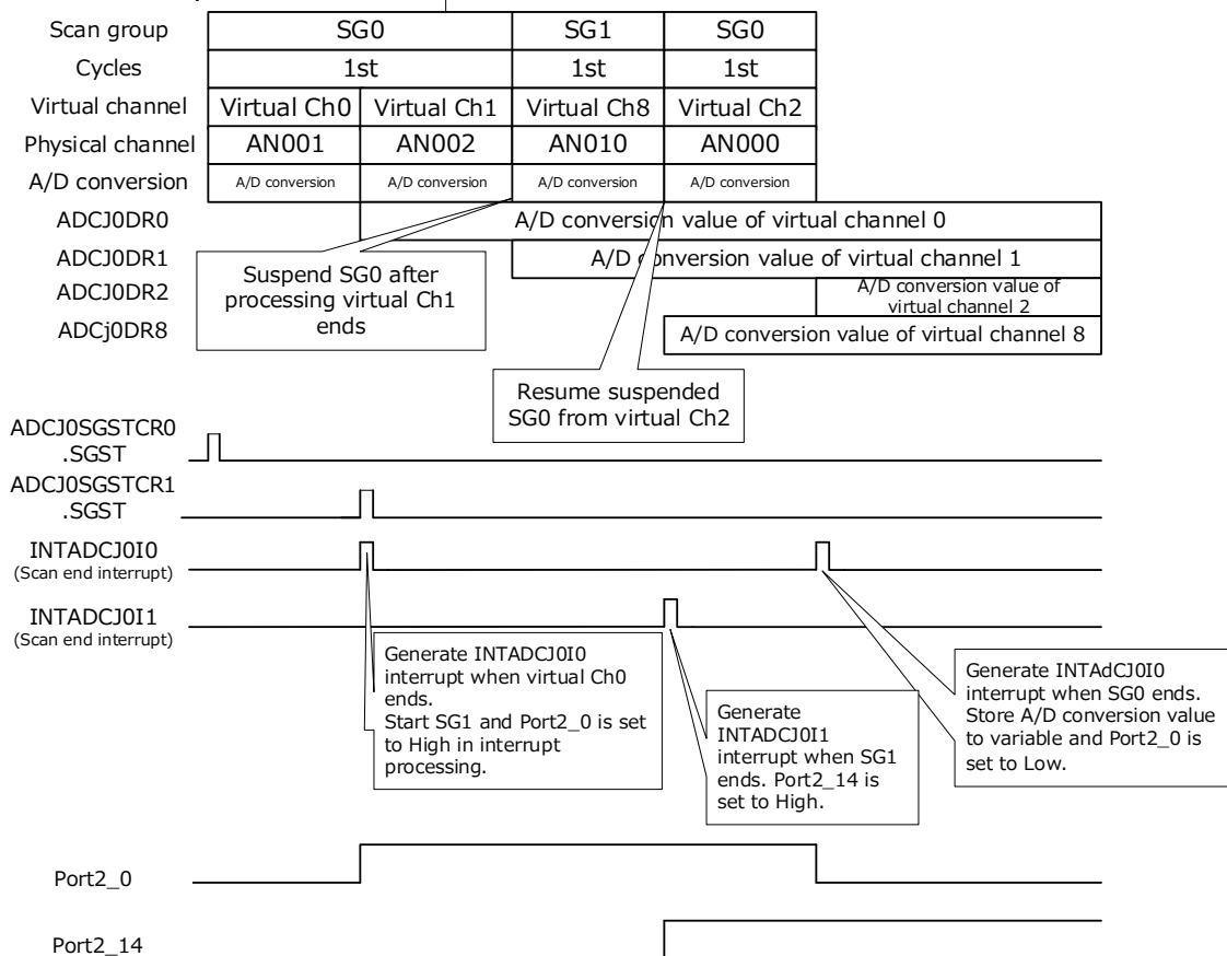
Figure 3.2.3 Operation Example of Synchronous Suspend &amp; Resume
