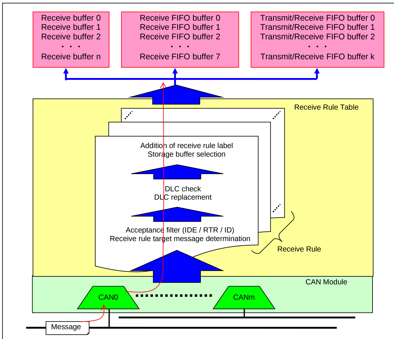
Figure 7-1 Filtering Image by receive rule table
