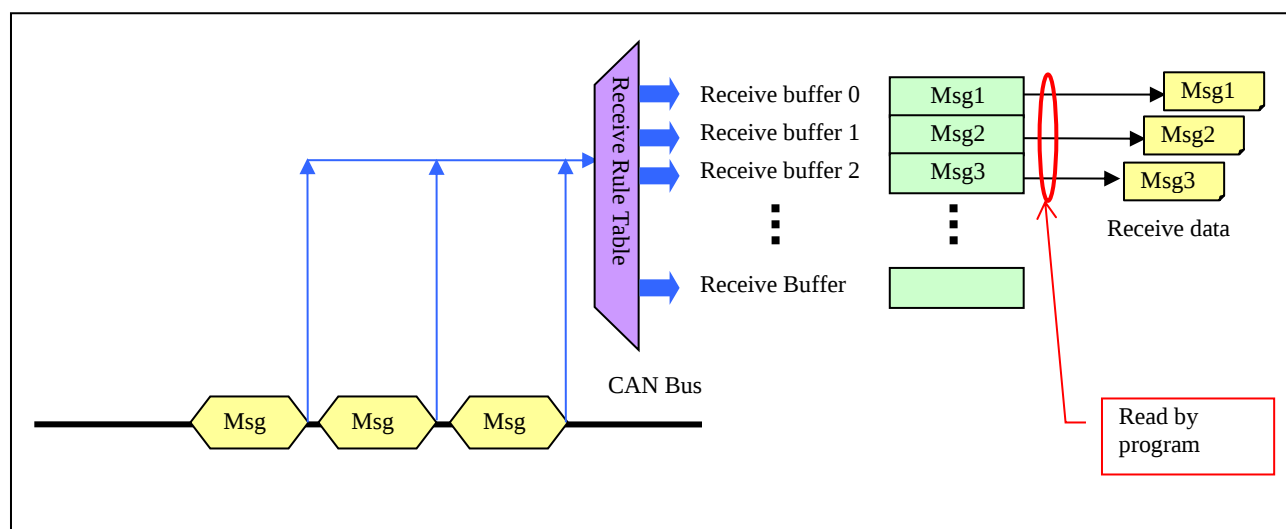
Figure 2-1 Receive Buffer Operation
