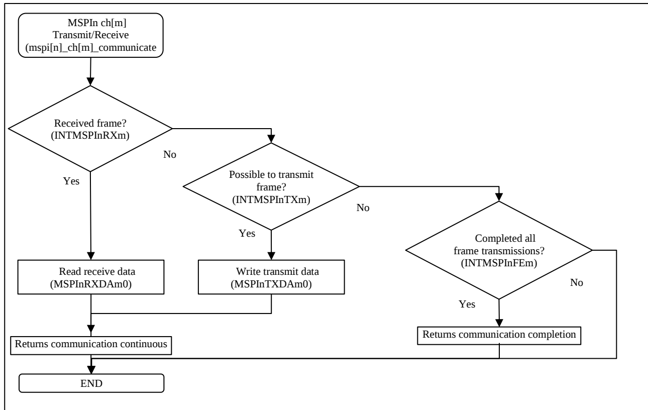
Figure 3-10 Operation Flow (2/2)
