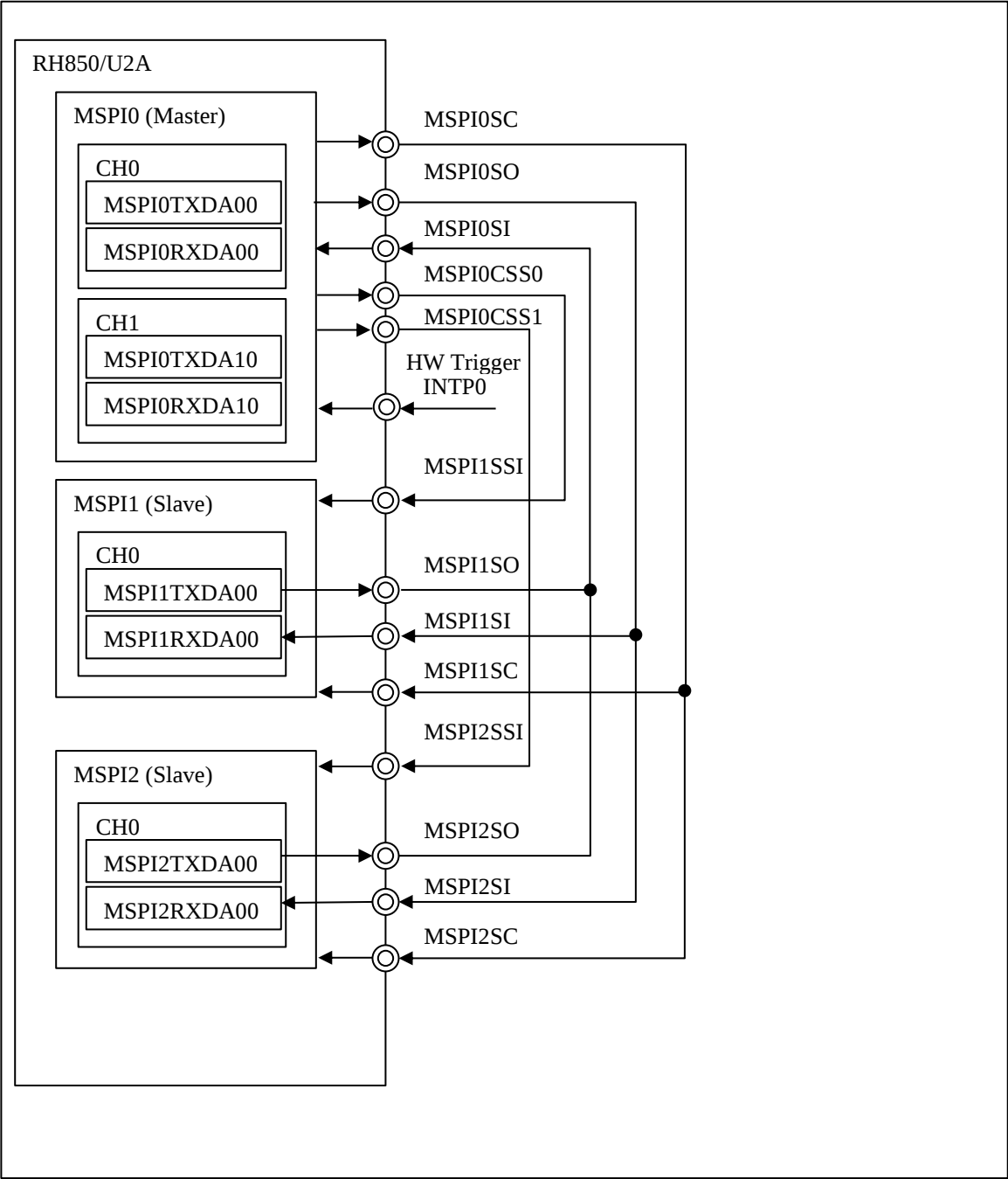
Figure 3-6 System Configuration
