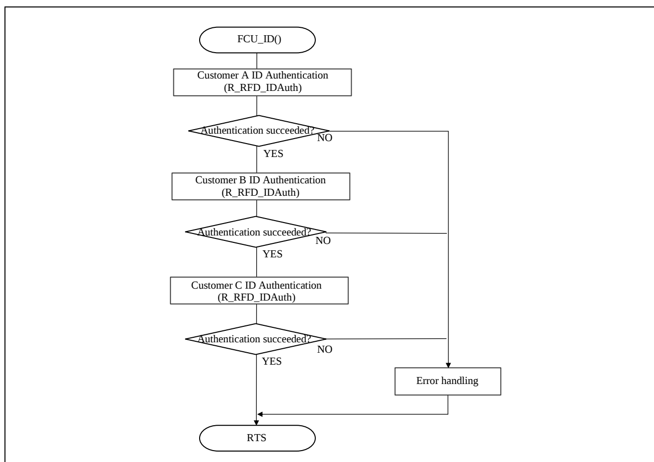
Figure 6-10 Flowchart of “FCU_ID()” function “Operation procedure (3)”
