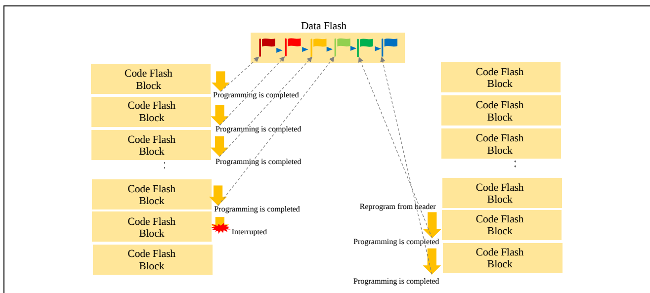
Figure 7-1 Diagram of managing progress with user flag
