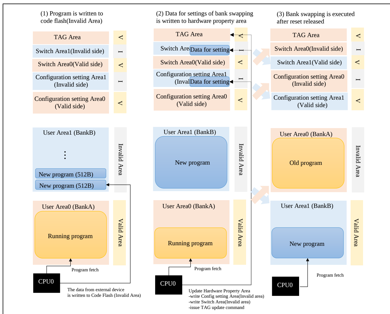
Figure 6-1 Overview of software update operation
