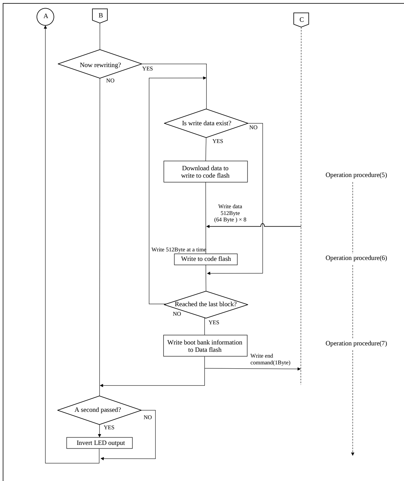
Figure 5-4 Overall sequence(2)
