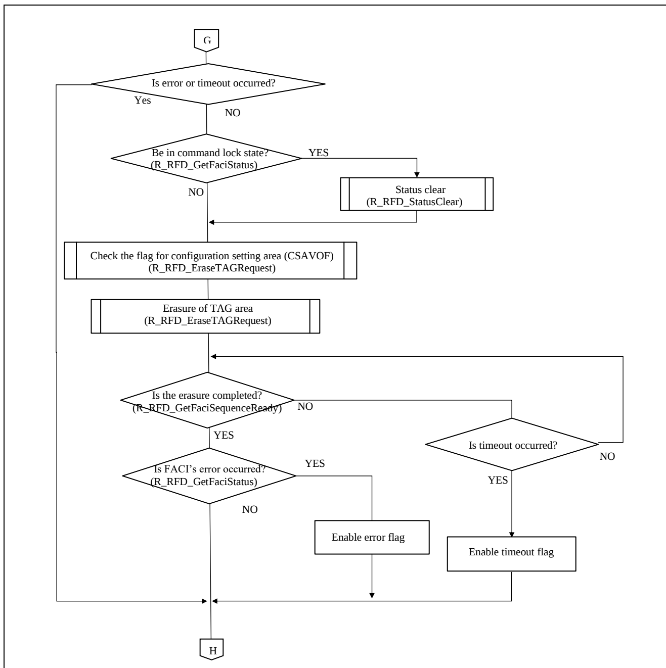
Figure 6-21 Flowchart of erasure the contents of TAG Area
