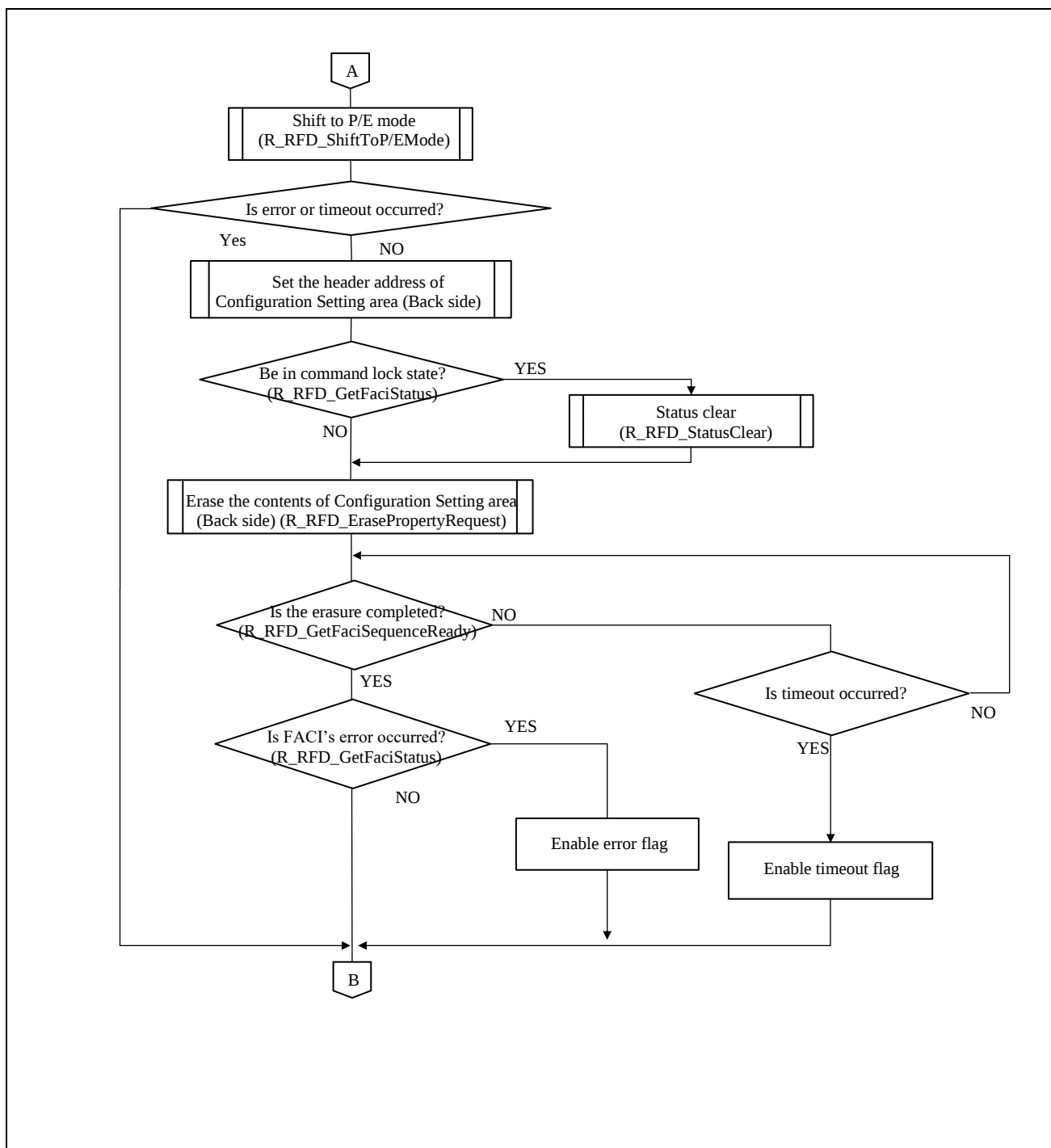
Figure 6-15 Flowchart of erasure the contents of Configuration Setting Area (Back side)
