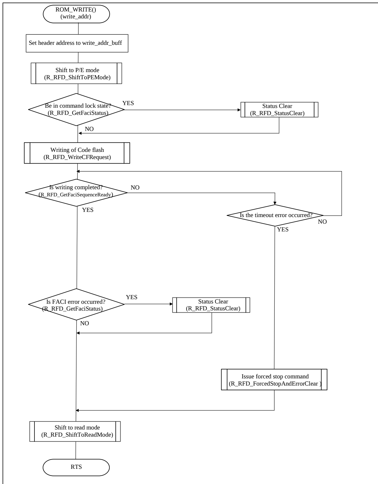
Figure 5-14 Flowchart of “ROM_WRITE()” function “Operation procedure (6)”
