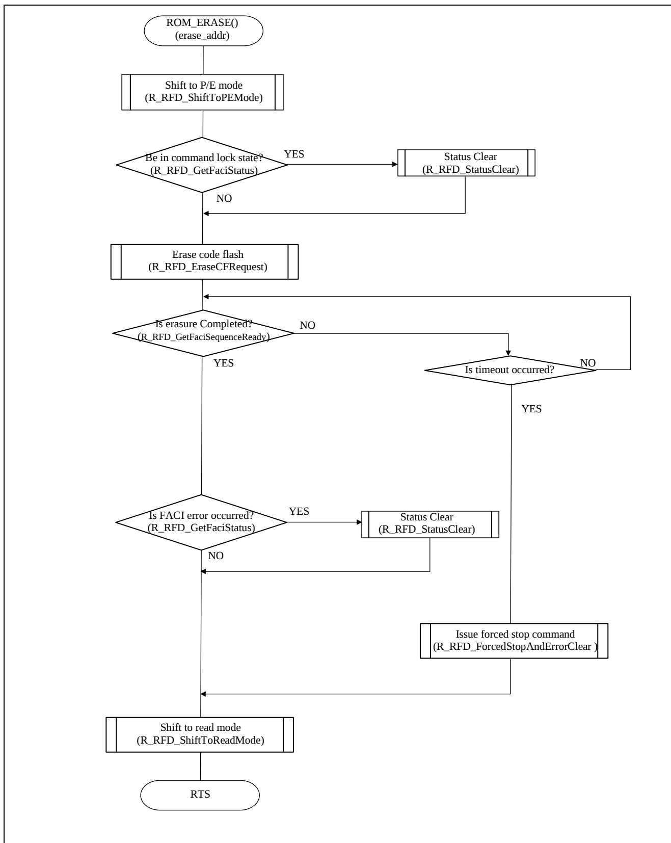
Figure 5-12 Flowchart of “ROM_ERASE()” function
