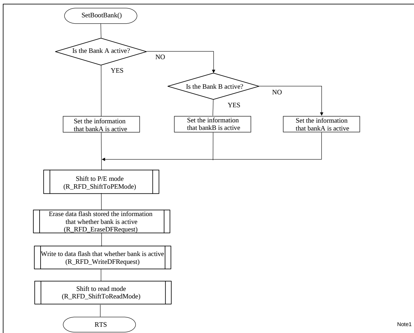
Figure 5-15 Flowchart of SetBootBank () function
