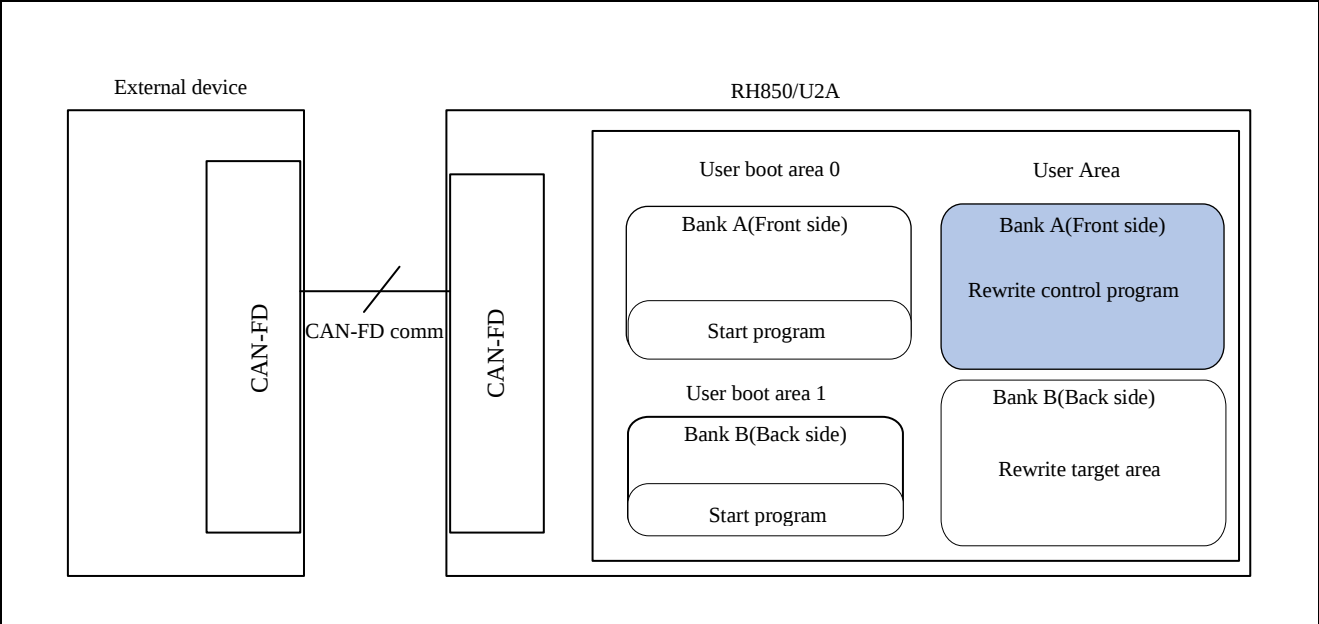
Figure 6-7 Program location of each Bank
