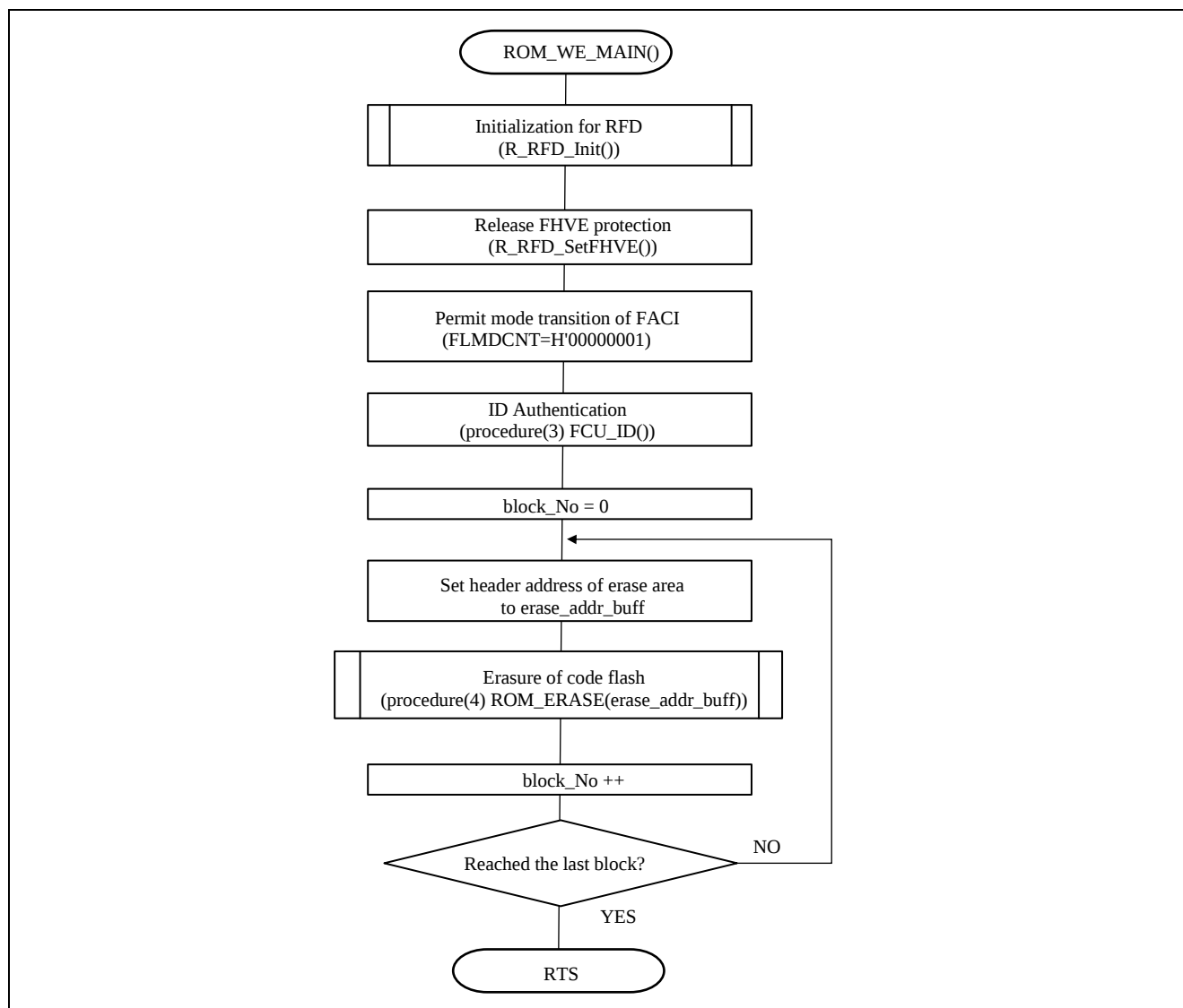
Figure 6-9 Flowchart of "ROM_WE_MAIN()" function
