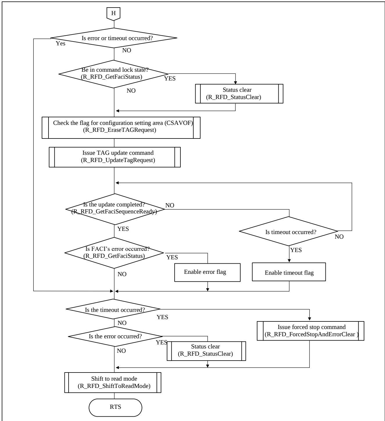
Figure 6-22 Flowchart of update the contents of Tag Area
