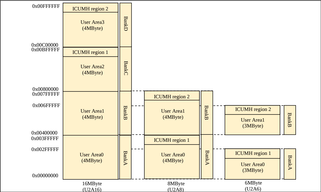
Figure 2-2 Code flash(User area) structure of single map mode Note1 .
