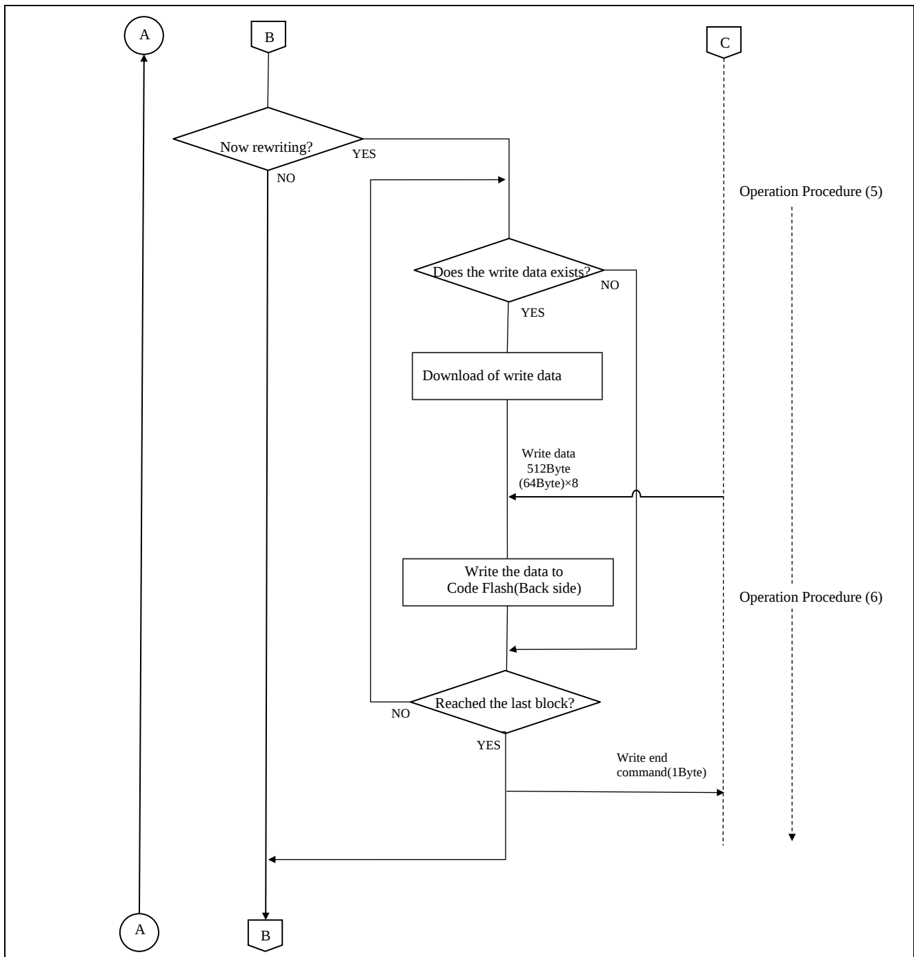
Figure 6-3 Overall sequence (2)
