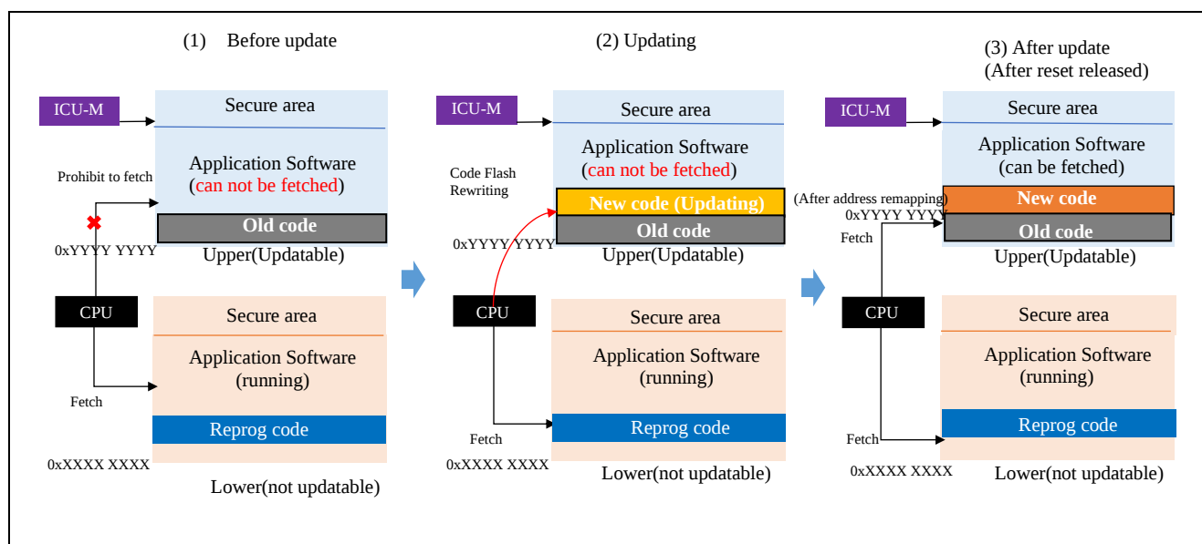
Figure 3-1 Method for reprogram diff code
