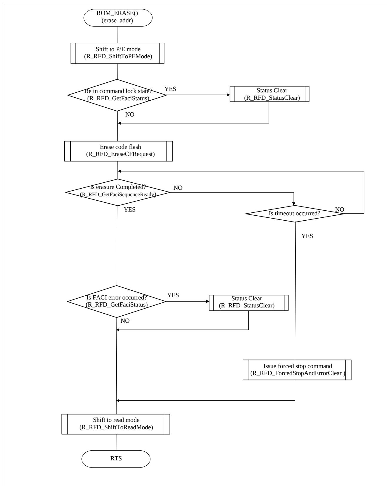
Figure 6-11 Flowchart of “ROM_ERASE()” function
