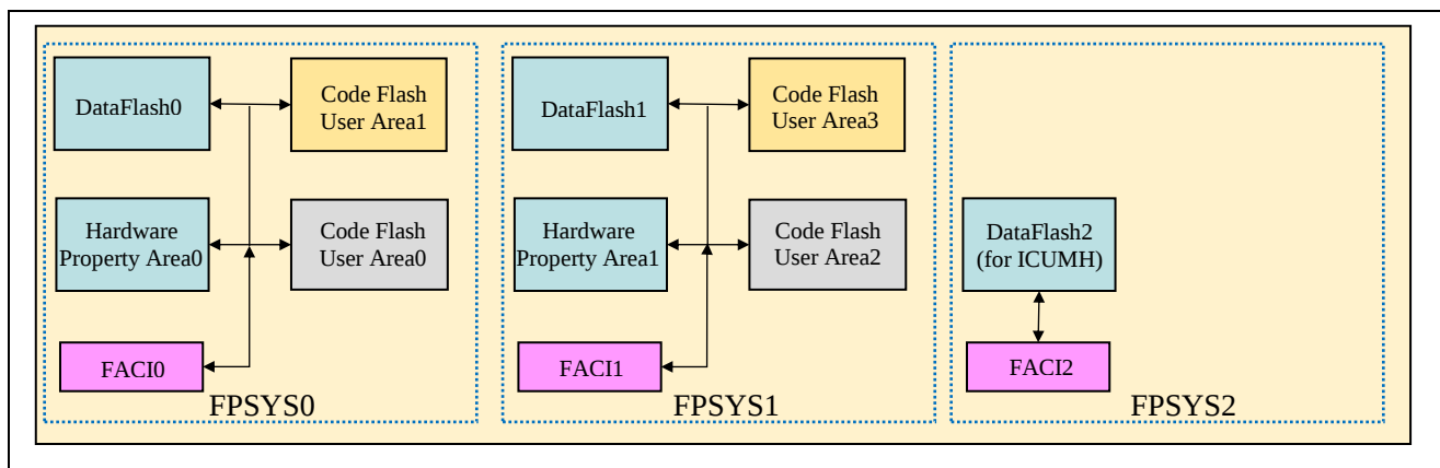
Figure 2-1 Block diagram of U2A16 Flash Programming System structure
