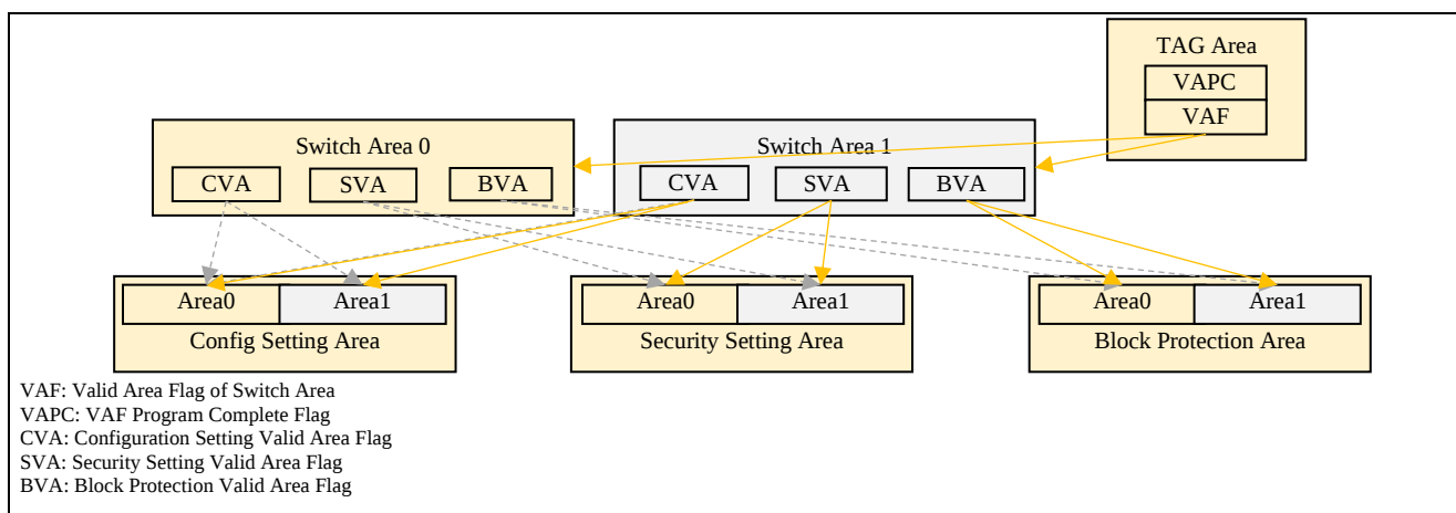
Figure 2-7 Details of Config Setting, Security Setting, Block Protection, Switch and TAG Area structure.
