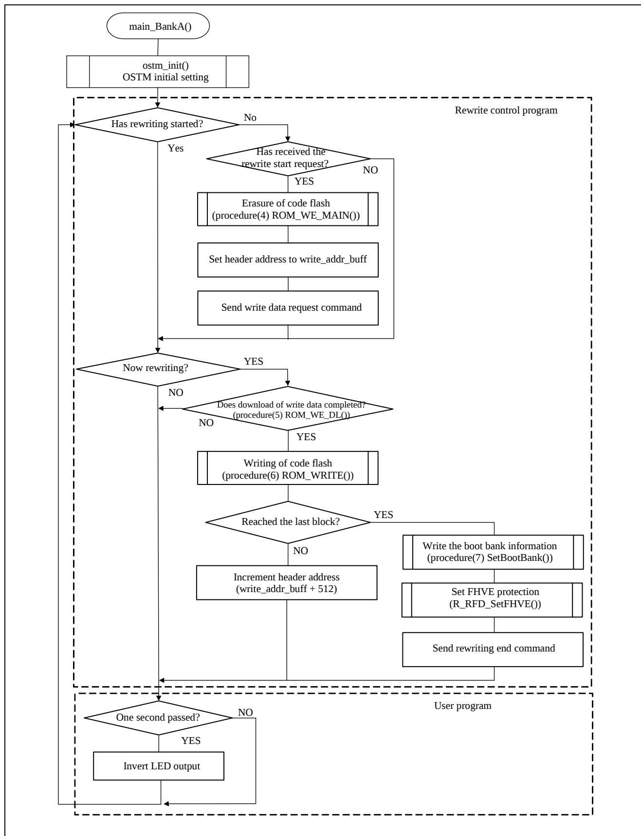
Figure 5-9 Flowchart of “main_BankA()” function
