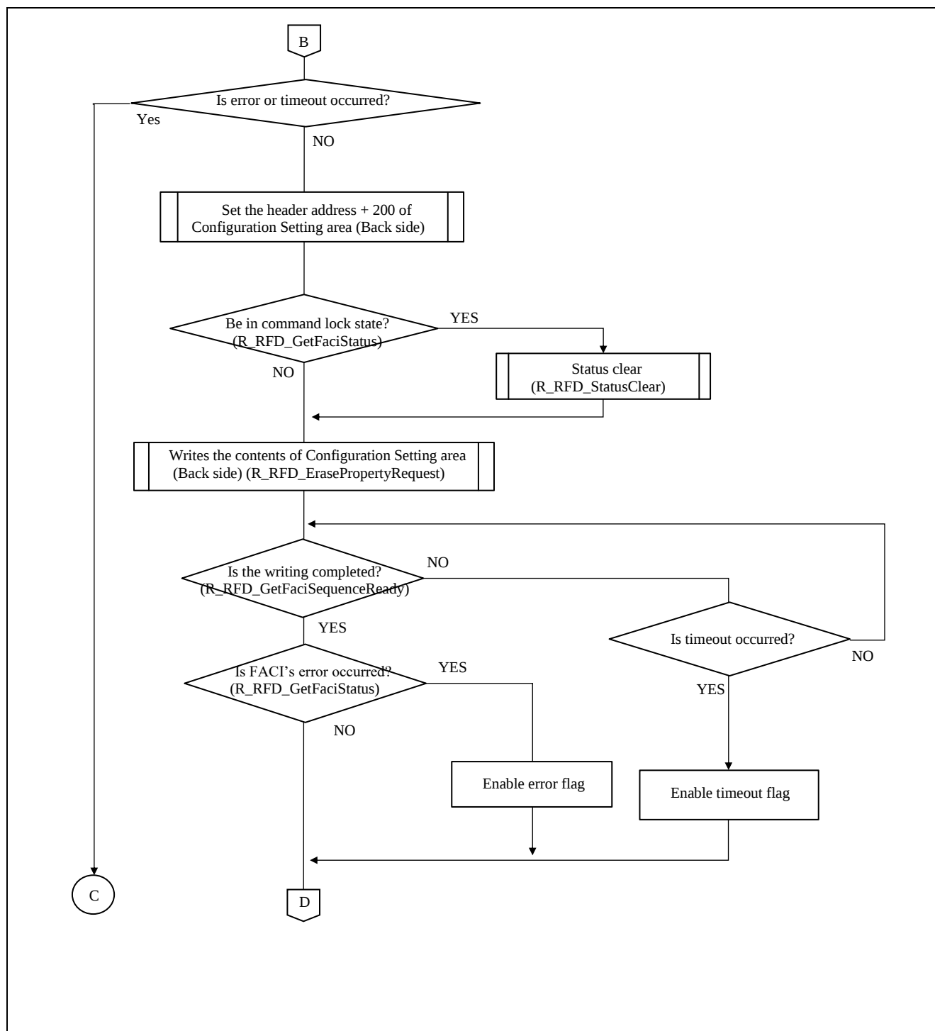
Figure 6-16 Flowchart of writing the data to Configuration Setting Area (Back side) (1)
