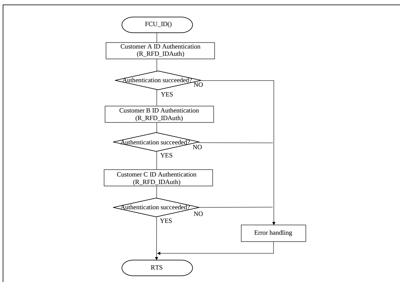
Figure 5-11 Flowchart of “FCU_ID()” function “Operation procedure (3)”
