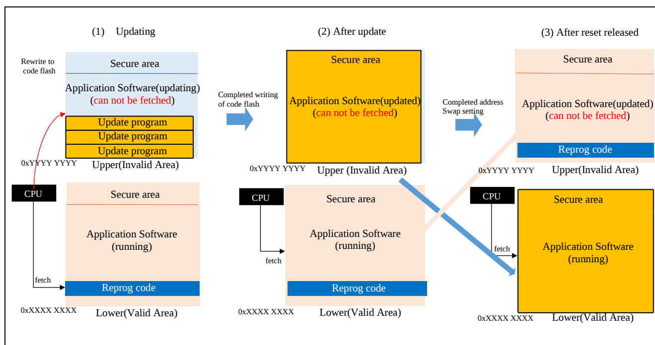
Figure 3-2 Method for bank swapping
