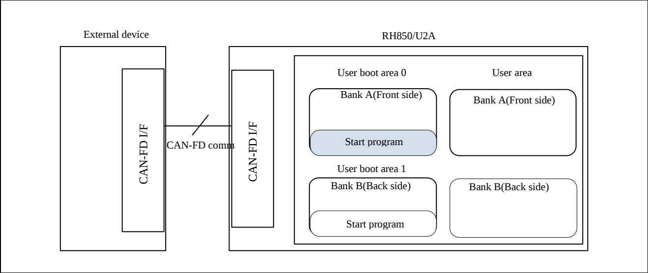
Figure 6-5 Startup program location
