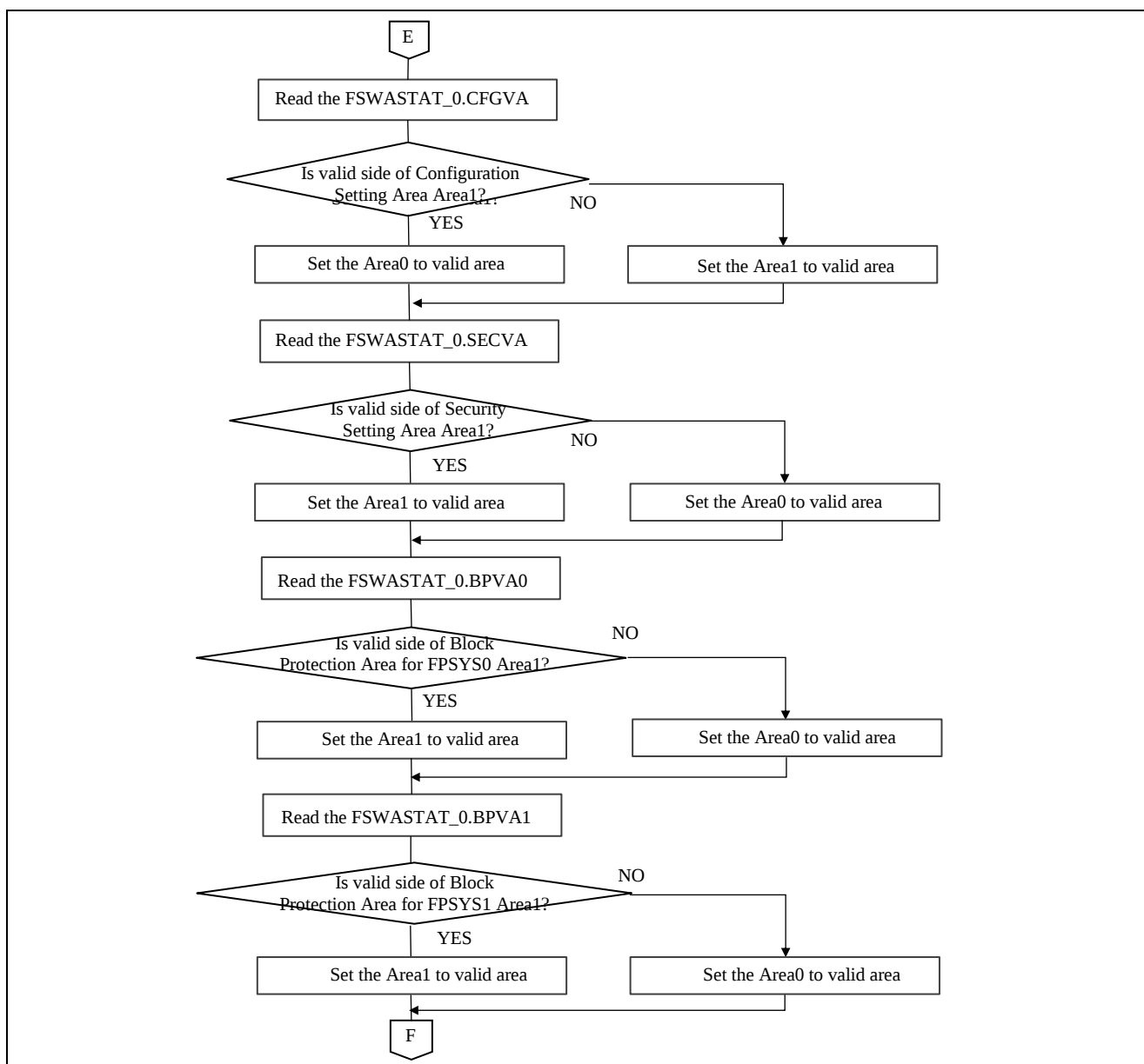
Figure 6-18 Flowchart of Setting the value for Switch Area (To Back side)
