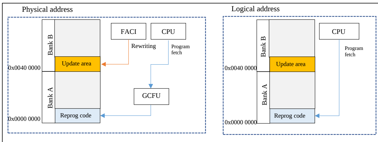
Figure 5-1 Rewriting operation in the case of Bank A is active
