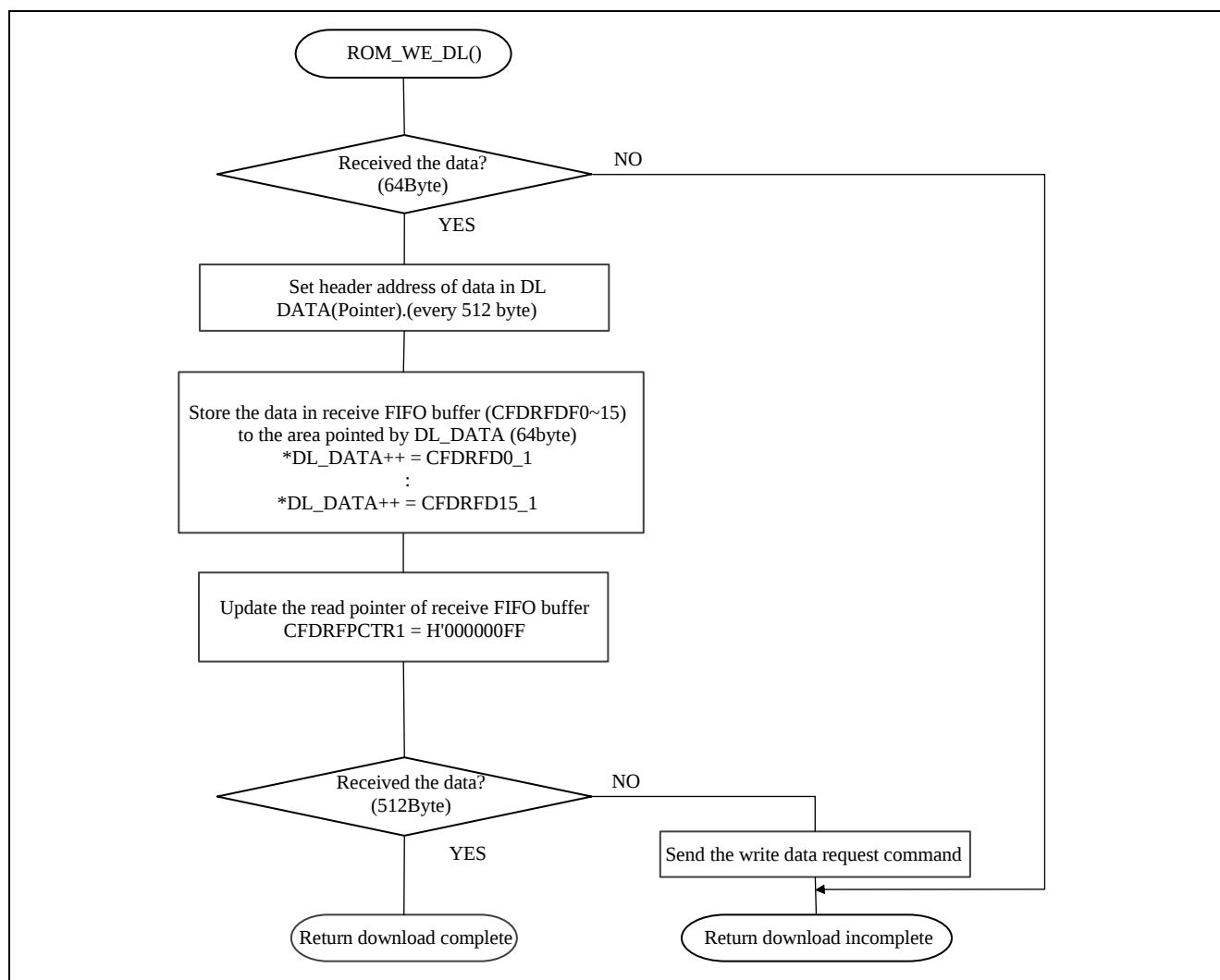
Figure 6-12 Flowchart of "ROM_WE_DL()" function
