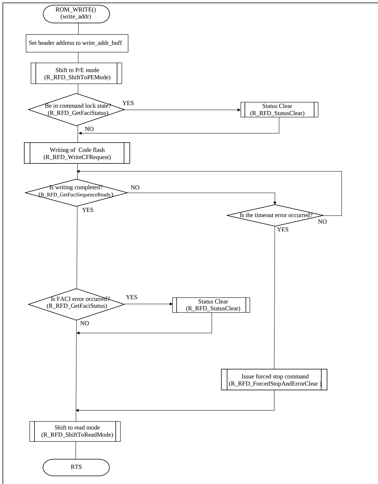
Figure 6-13 Flowchart of “ROM_WRITE()” function “Operation procedure (6)”
