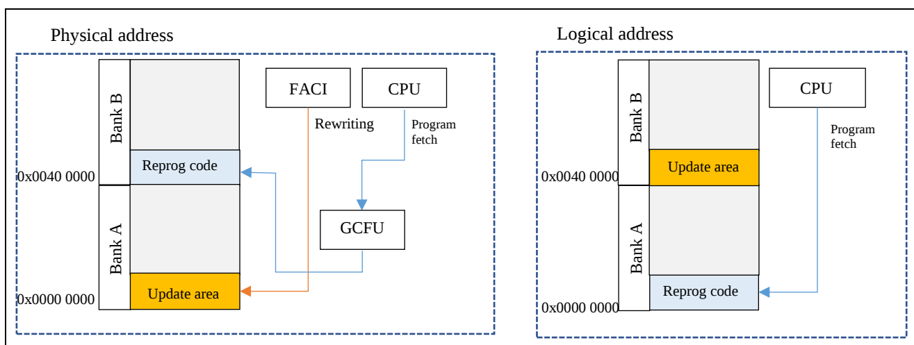
Figure 5-2 Rewriting operation in the case of Bank B is active
