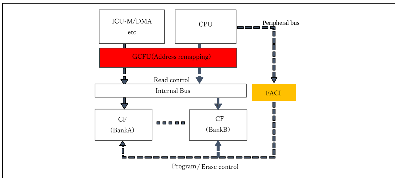
Figure 2-5 Bus structure related flash memory accesses.
