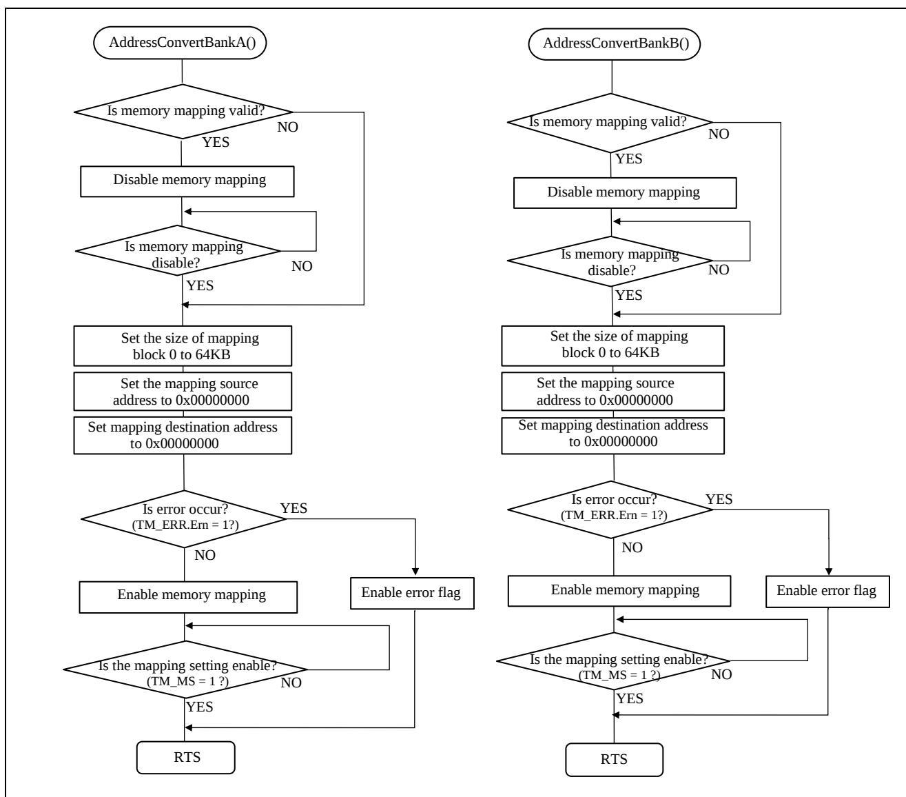
Figure 5-7 Flowchart of “Bank switching function”
