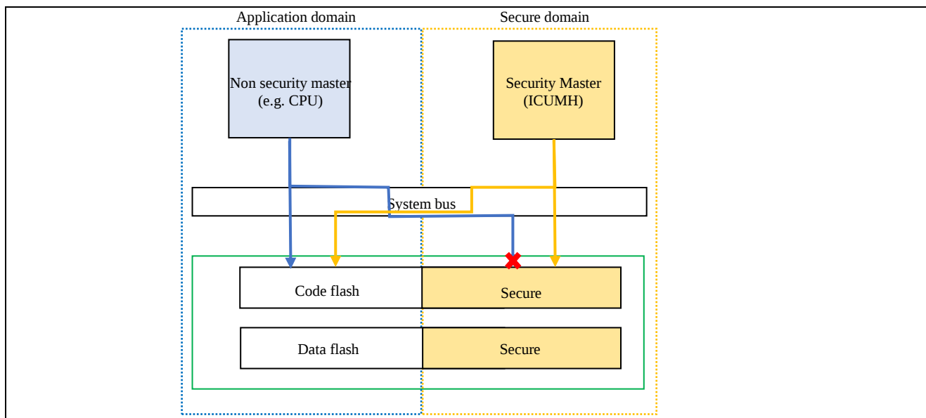
Figure 3-3 Diagram of access master.
