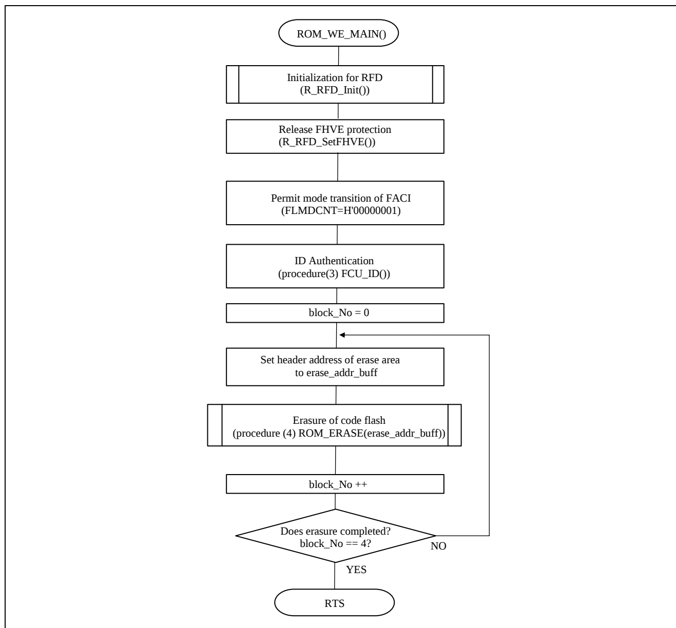
Figure 5-10 Flowchart of “ROM_WE_MAIN()” function Included operation procedure (3) and (4).
