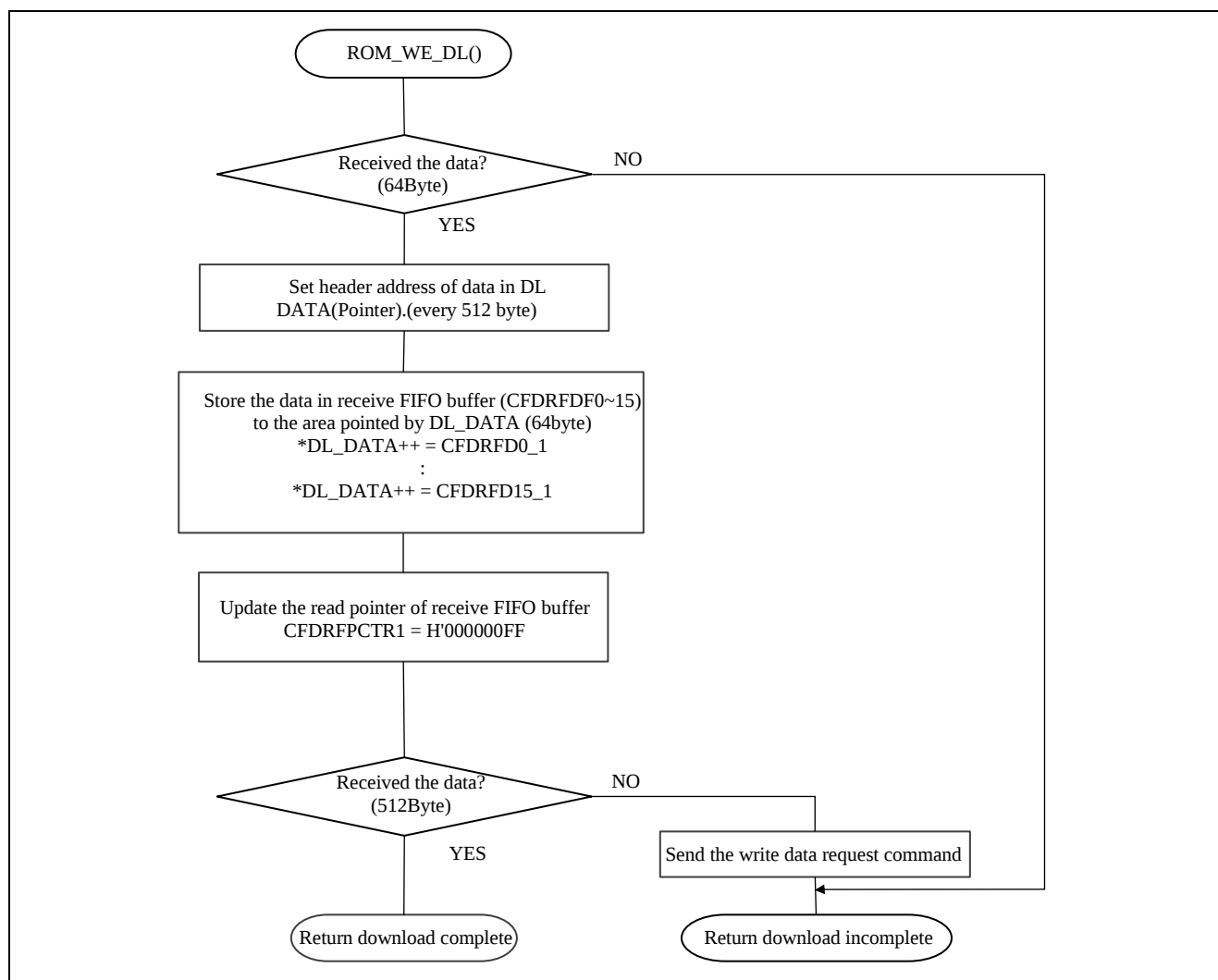
Figure 5-13 Flowchart of "ROM_WE_DL()" function
