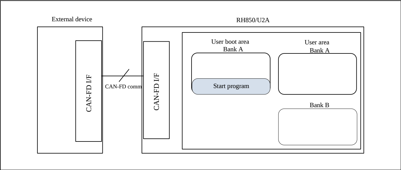
Figure 5-5 Startup program location
