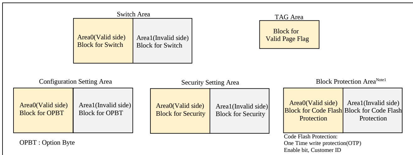
Figure 2-6 Overview of the hardware property area (shipping value)
