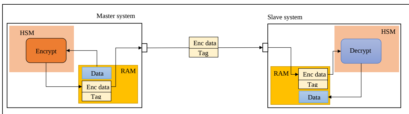
Figure 3-4 Diagram of communication with encryption
