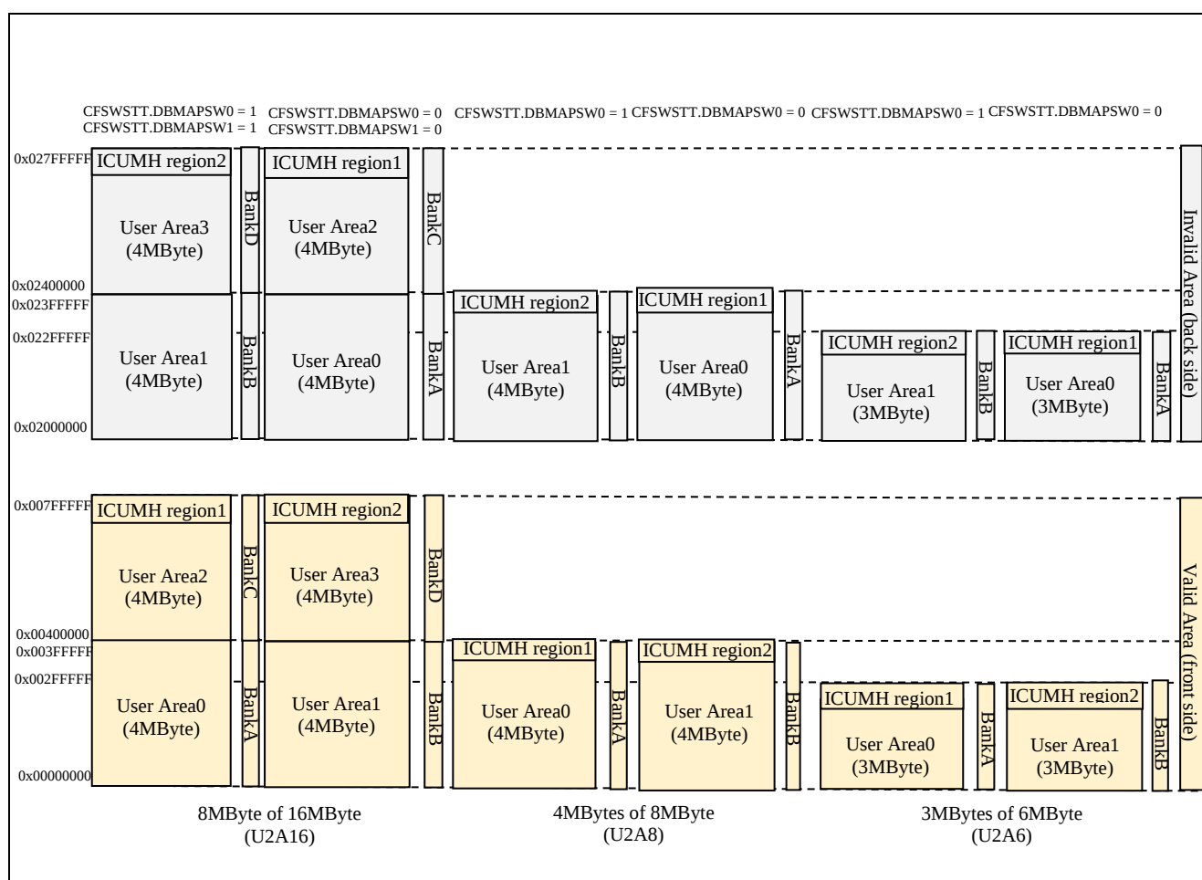
Figure 2-3 Code flash (User area) structure of double map mode Note1 .
