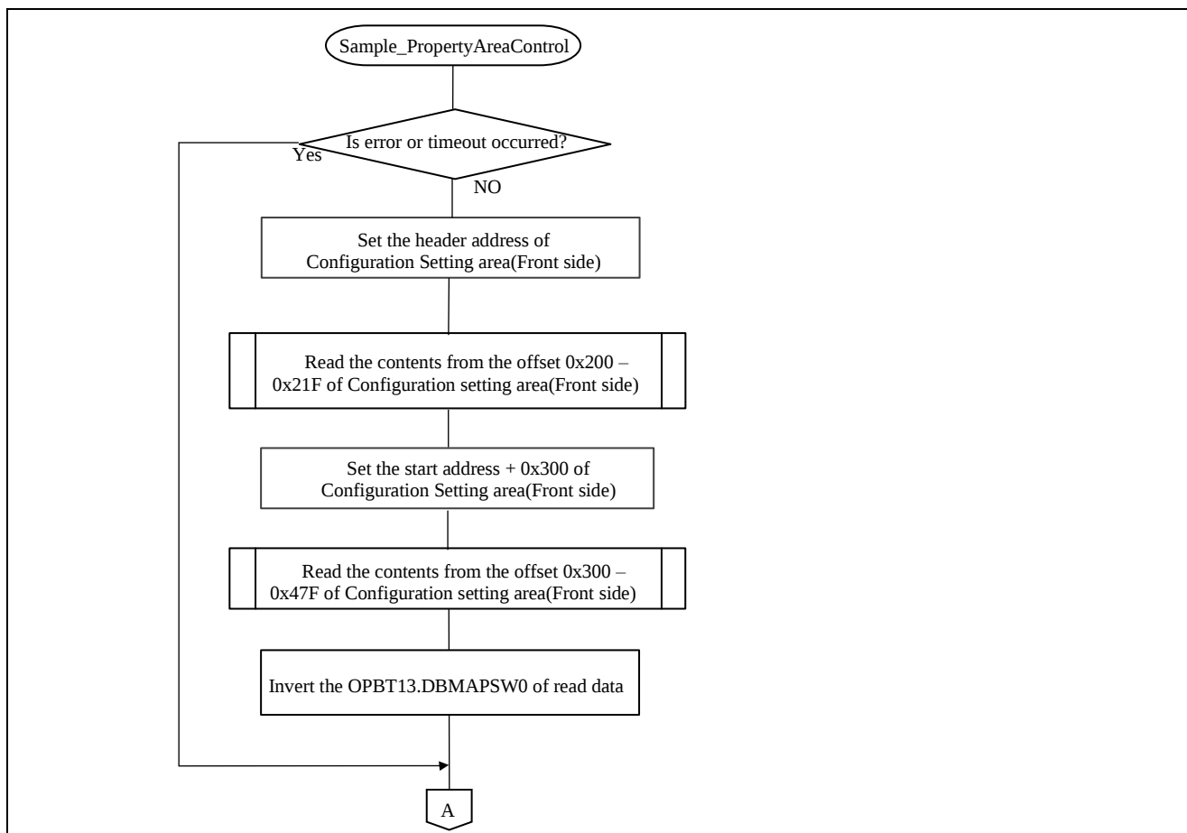
Figure 6-14 Flowchart of reading the contents of Configuration Setting Area (Front side)
