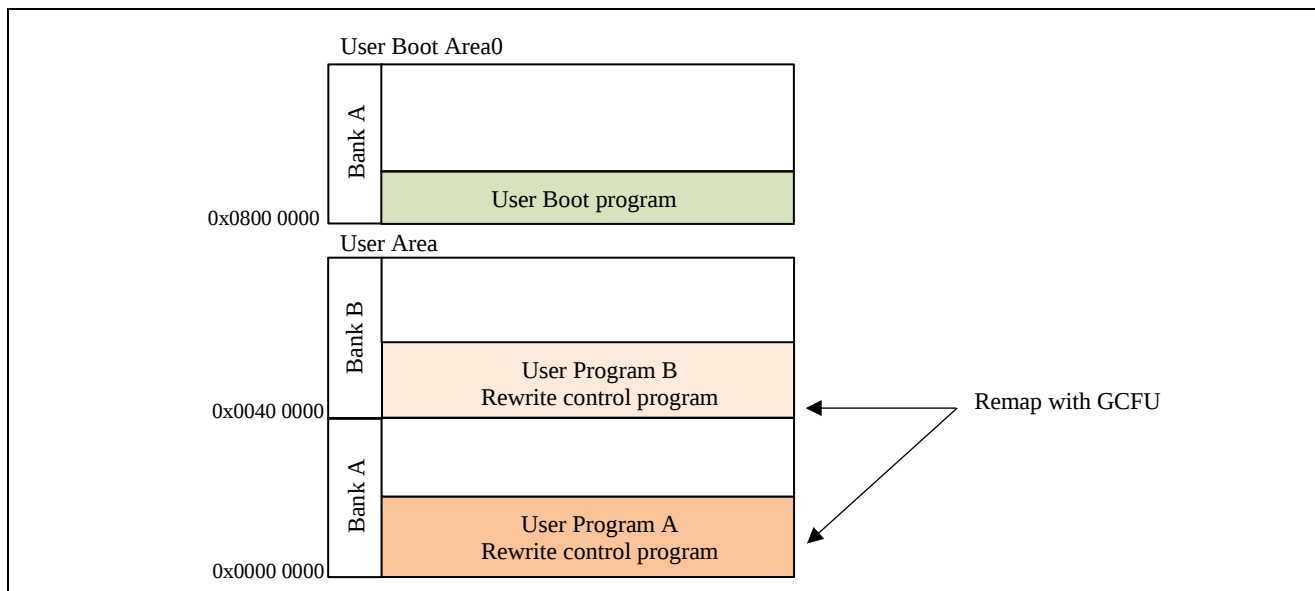
Figure 2-4 Flash access remapped by GCFU
