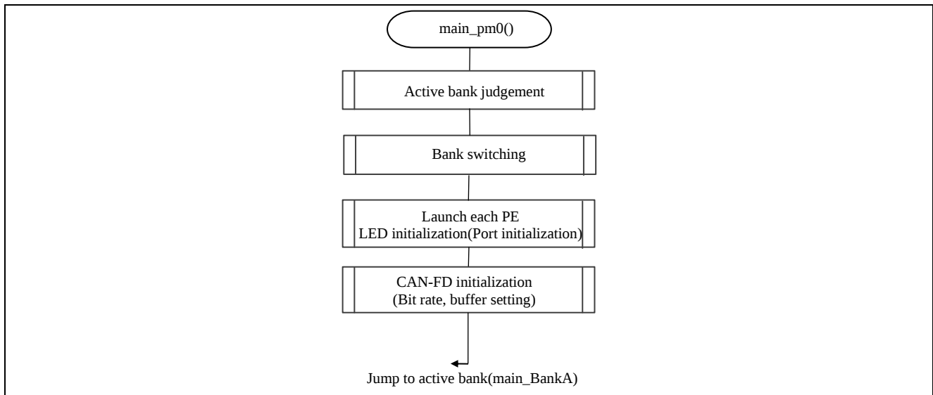
Figure 5-6 Flowchart of main_pm0()
