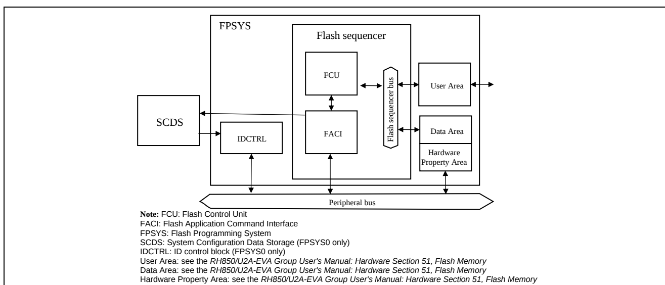
Figure 2-8 Structure of Flash Programming System
