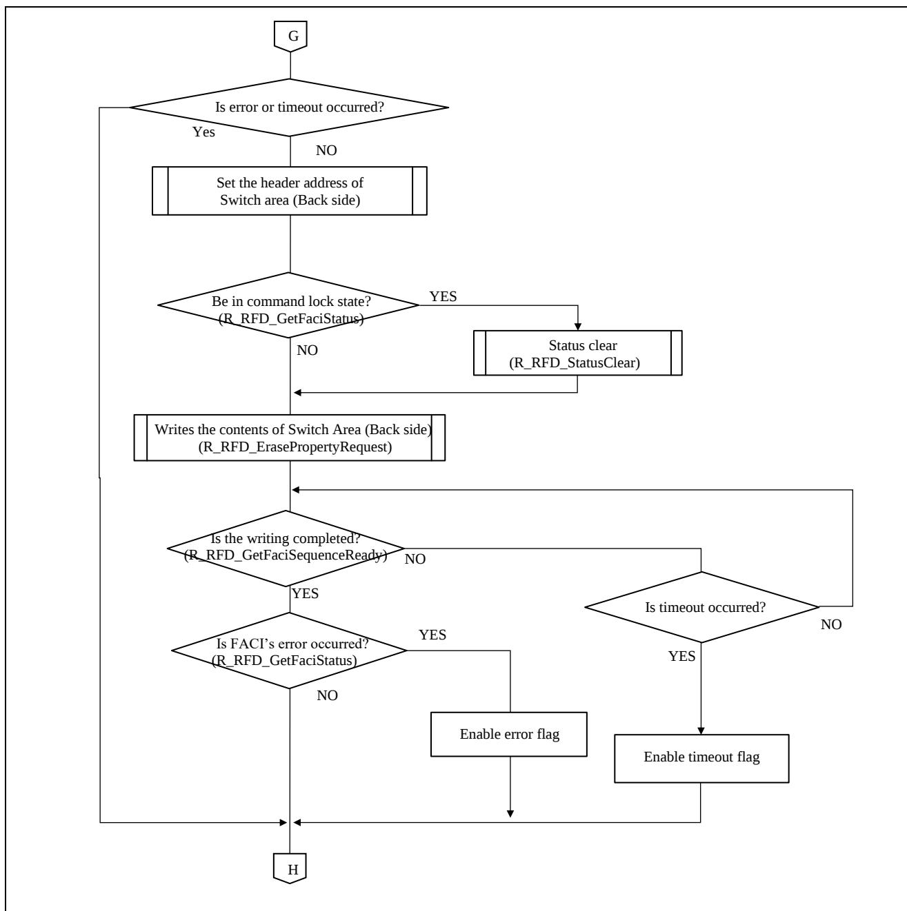
Figure 6-20 Flowchart of writing the contents of Switch Area (Back side)
