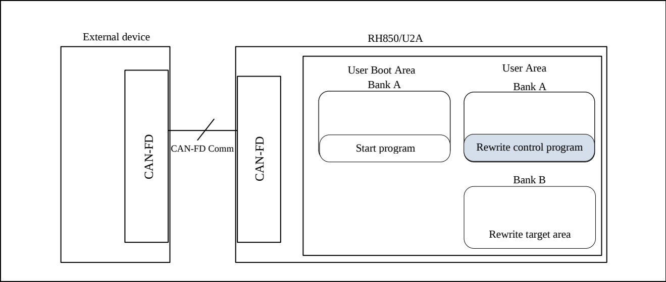
Figure 5-8 Program location of each Bank
