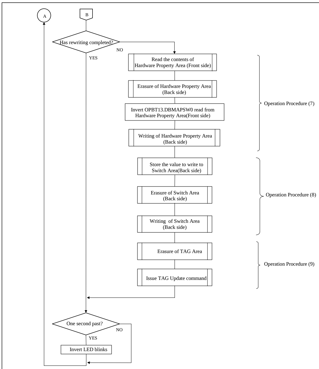
Figure 6-4 Overall sequence (3)
