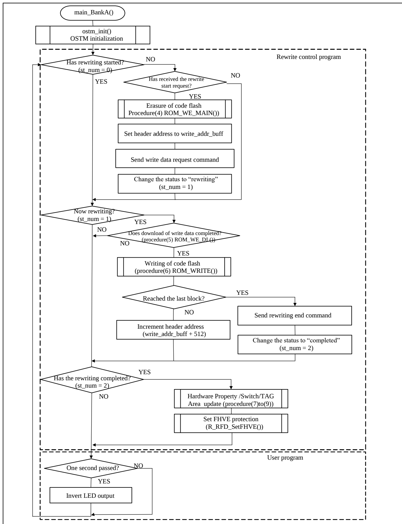
Figure 6-8 Flowchart of “main_BankA()” function “Operation procedure (2)”
