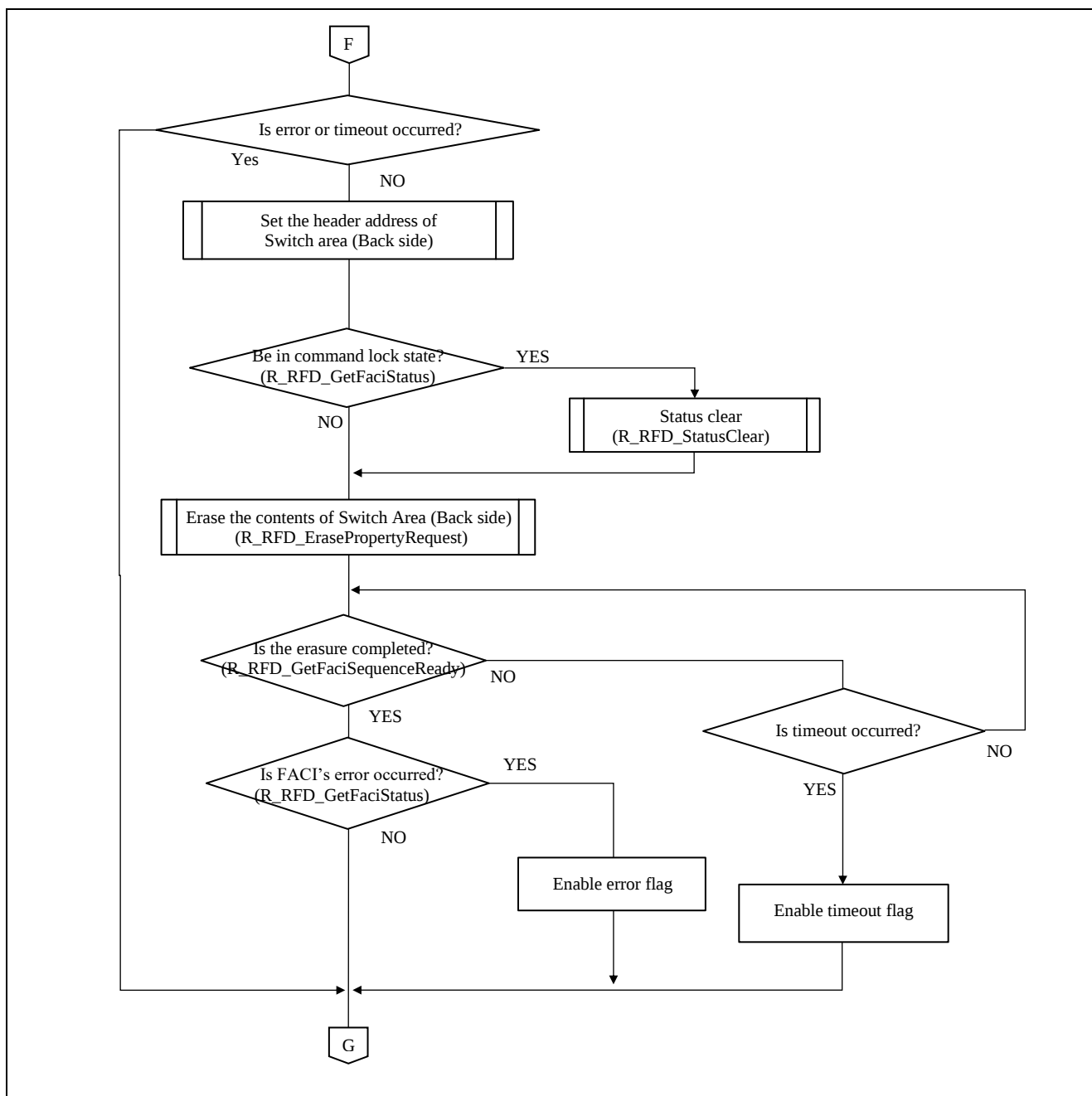
Figure 6-19 Flowchart of erasure the contents of Switch Area (Back side)
