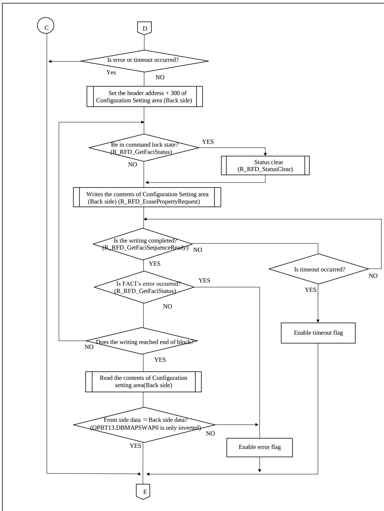
Figure 6-17 Flowchart of writing the data to Configuration Setting Area (Back side) (2)
