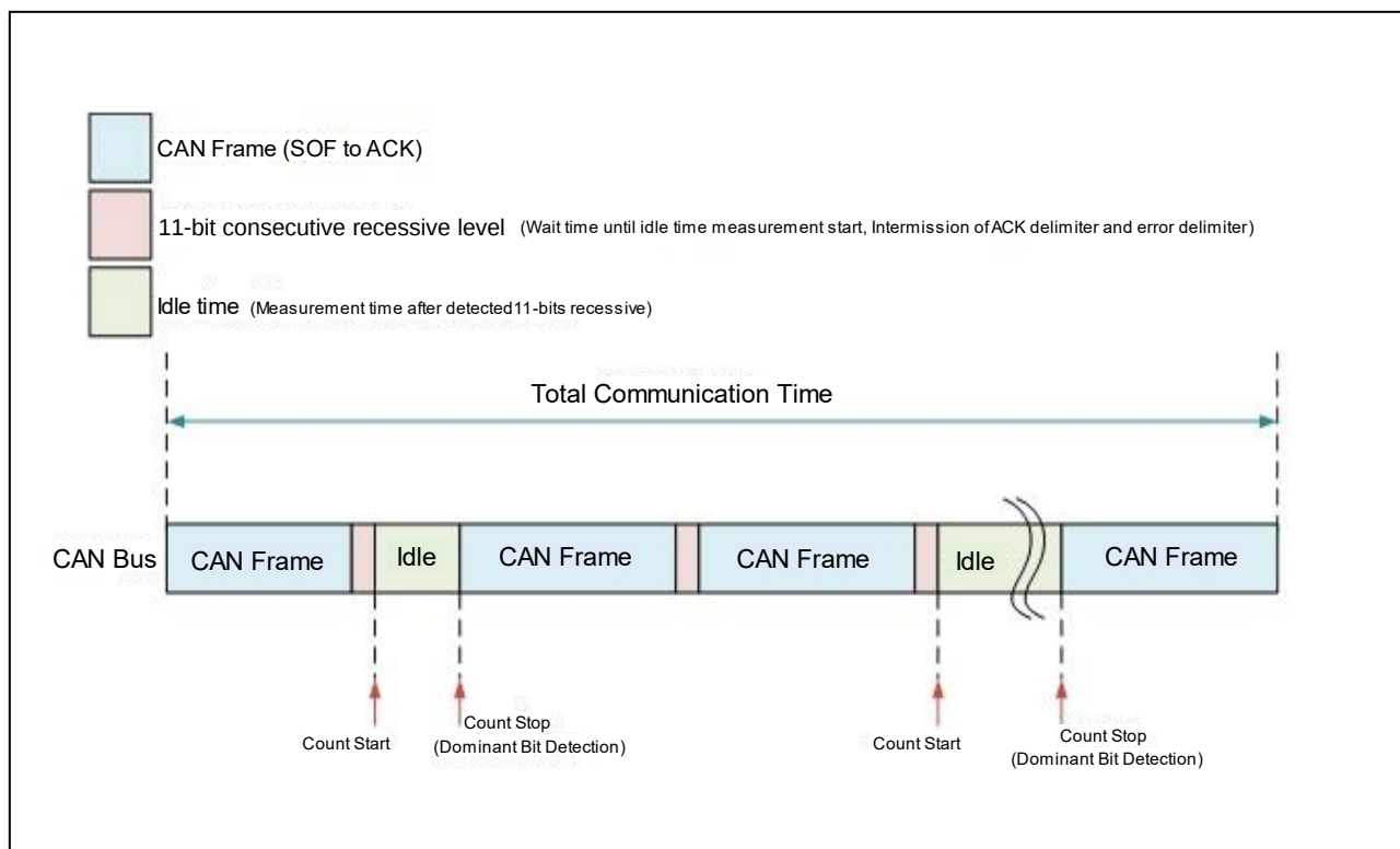
Figure 4-1 Bus Traffic Measurement Function Overview
