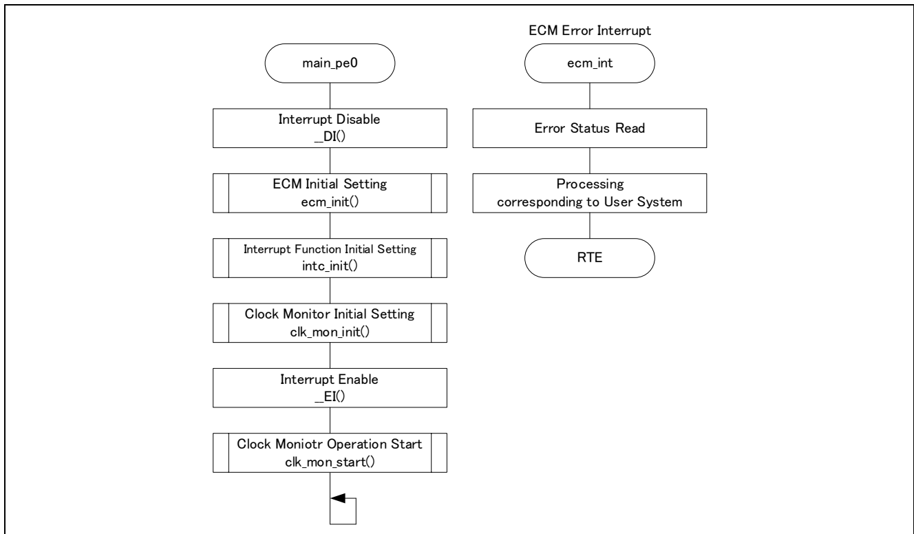
Figure 2-3 Flowchart
