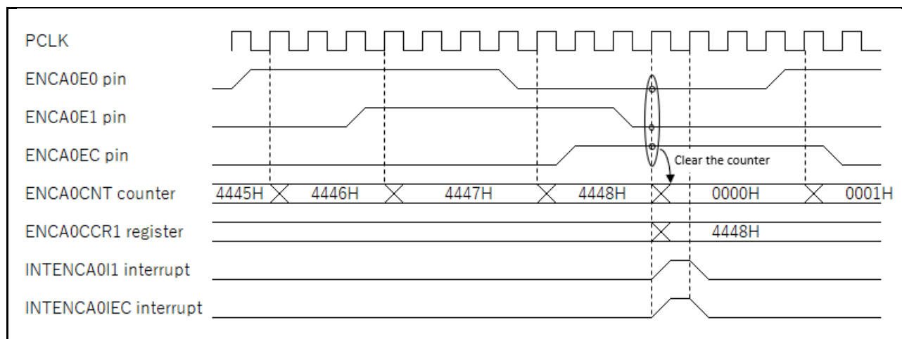
Figure 2-1 ENCA0 operation overview
