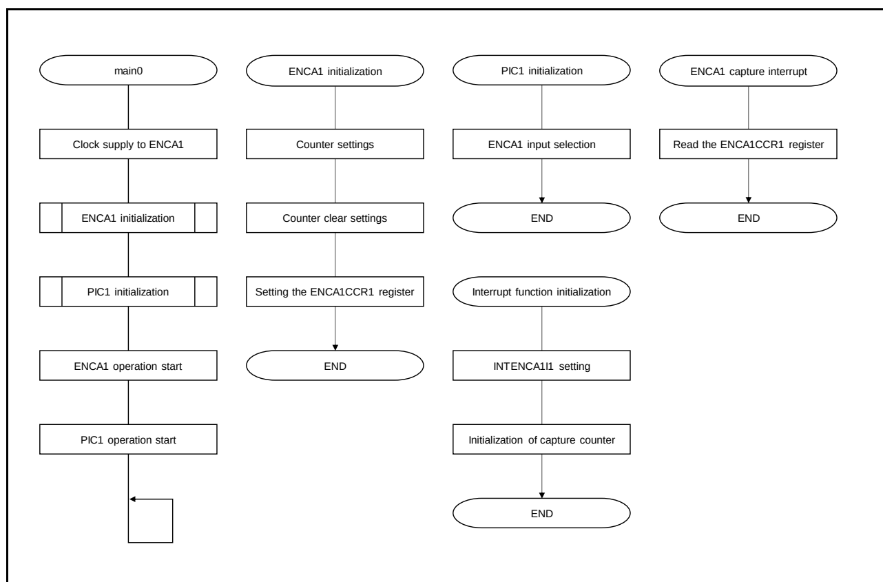
Figure 3-2 ENCA1, PIC1 operation flowchart
