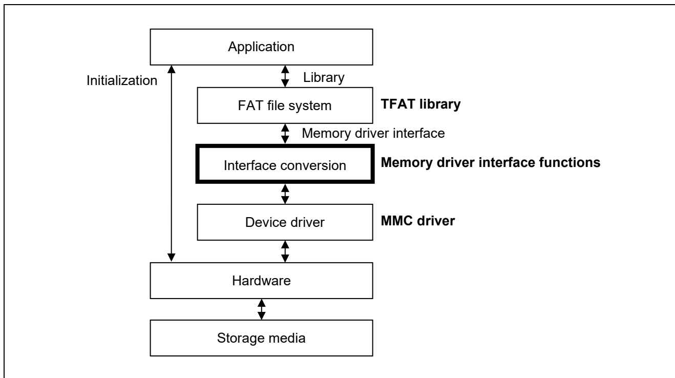
Figure 4.1 Configuration of TFAT Library and MMC Driver
