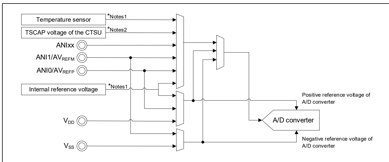
Figure 2-4 Configuration of Testing of the A/D converter (RL78/G13, G14, G22, G23)
