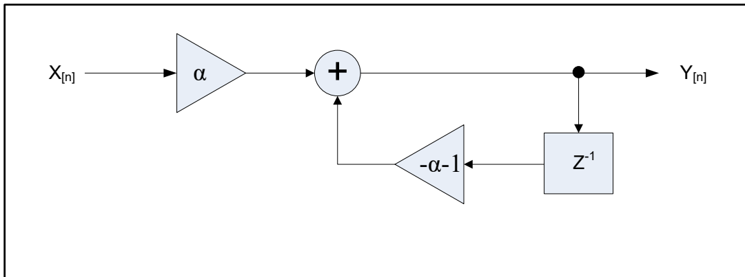
Figure 3-6 High-Pass Single Pole IIR
