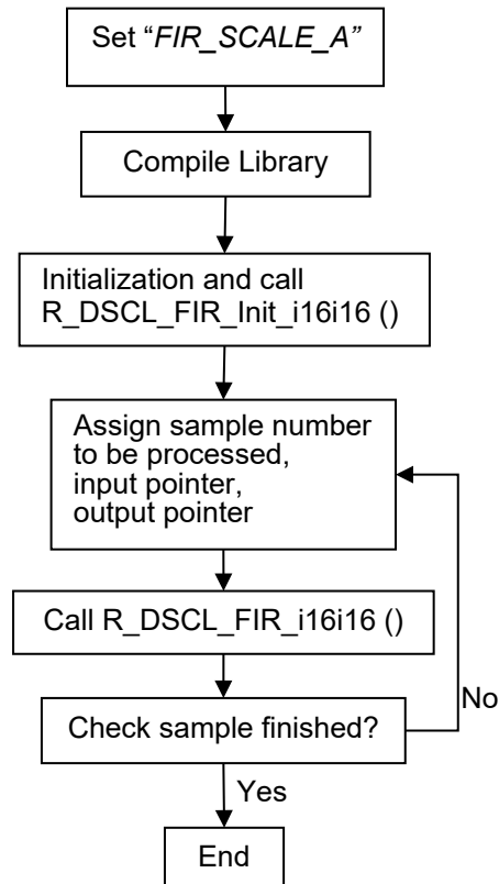
Figure 3-2 Processing flow
