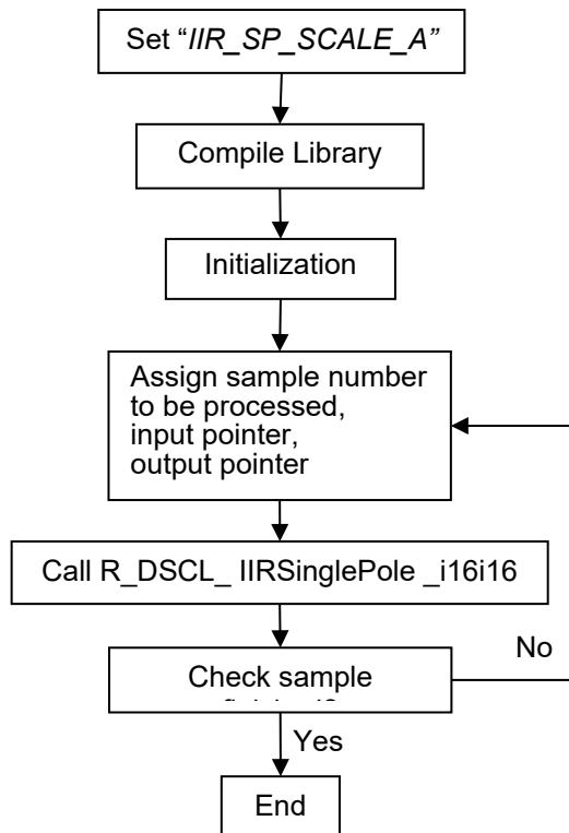
Figure 3-7 Processing flow
