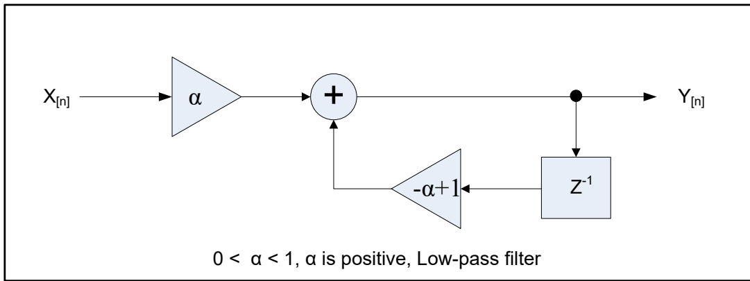
Figure 3-5 Low-pass Single Pole IIR
