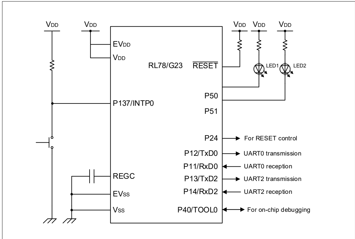
Figure 4-1 Hardware Configuration
