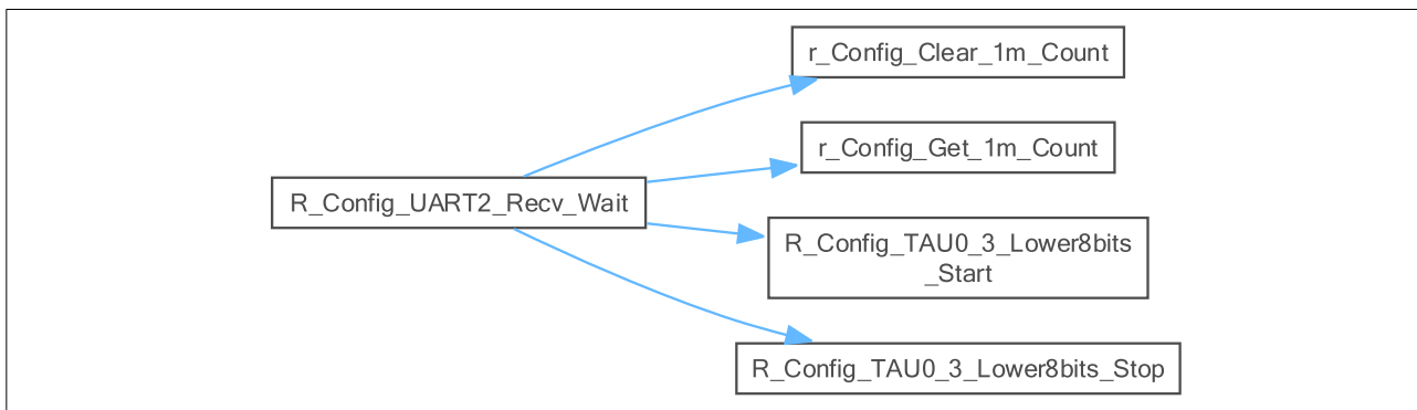
Figure 5-54 Call Graph of R_Config_UART2_Recv_Wait
