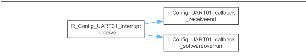
Figure 5-48 Call Graph of R_Config_UART01_interrupt_receive
