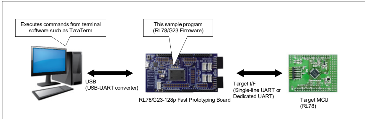
Figure 1-1 Online Mode
