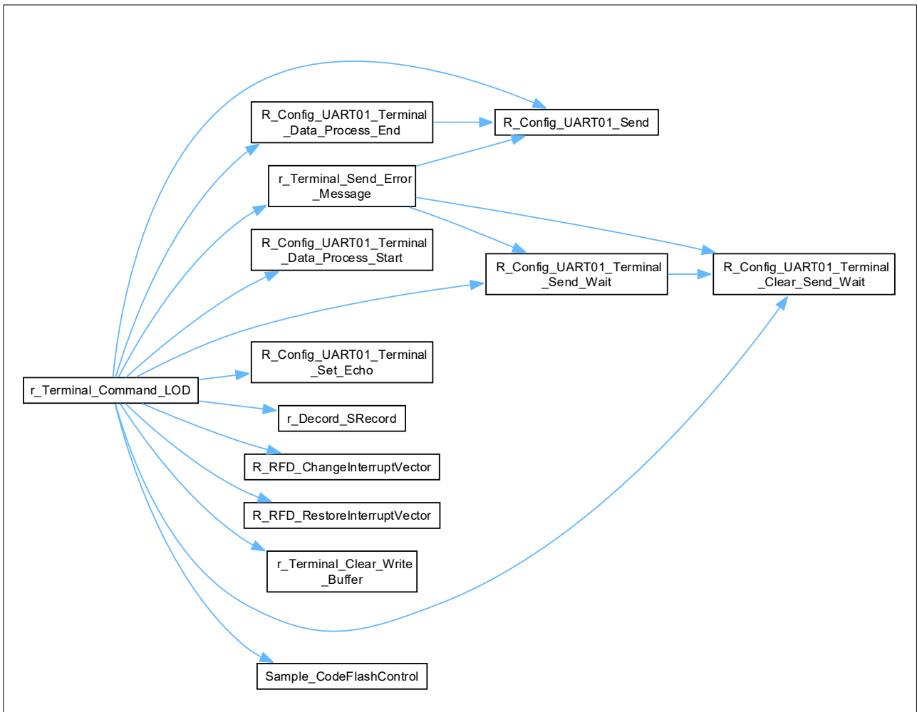
Figure 5-13 Call Graph of r_Terminal_Command_LOD
