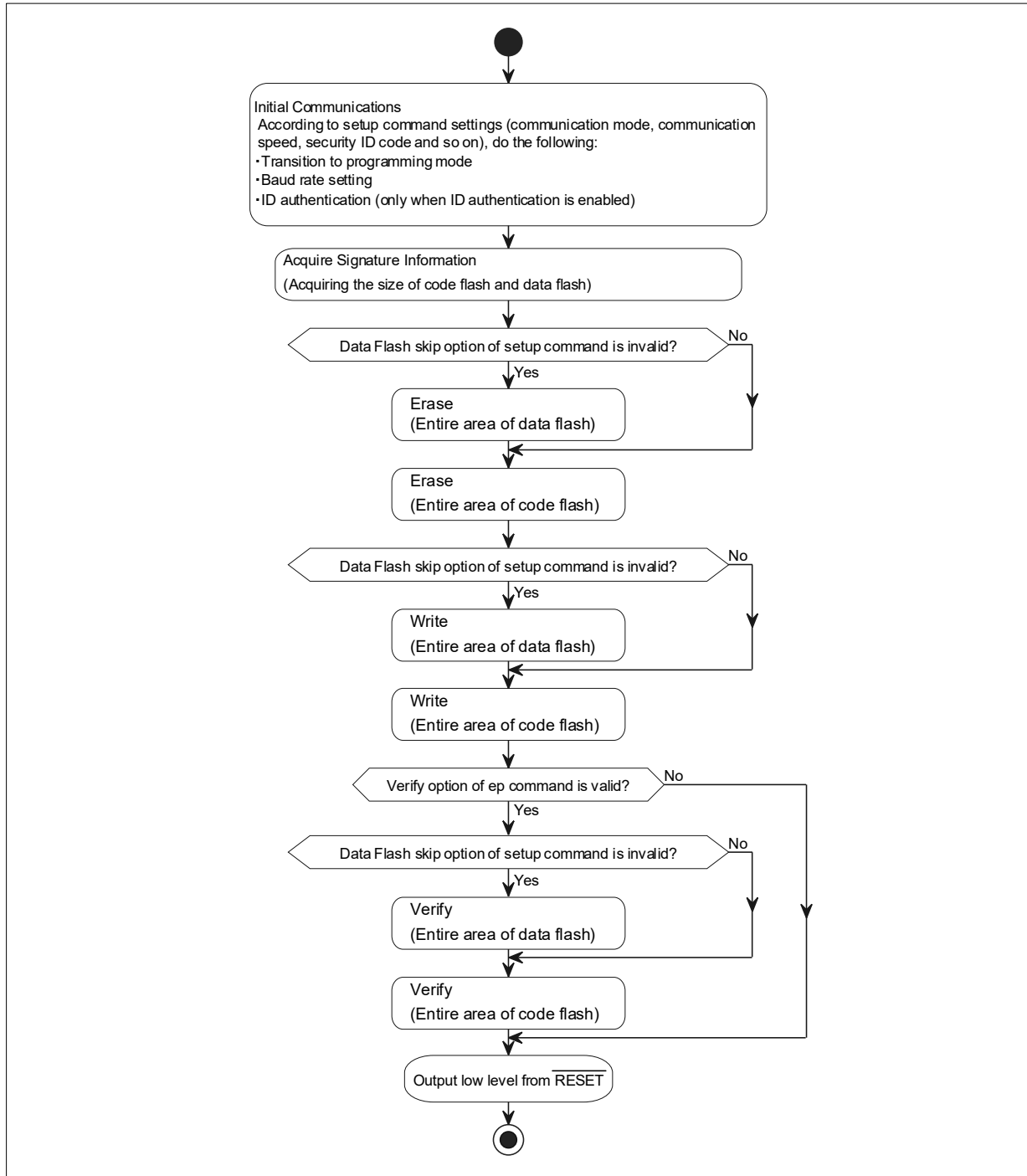
Figure 3-6 Offline Mode
