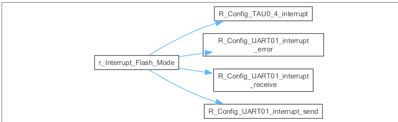
Figure 5-56 Call Graph of r_Interrupt_Flash_Mode
