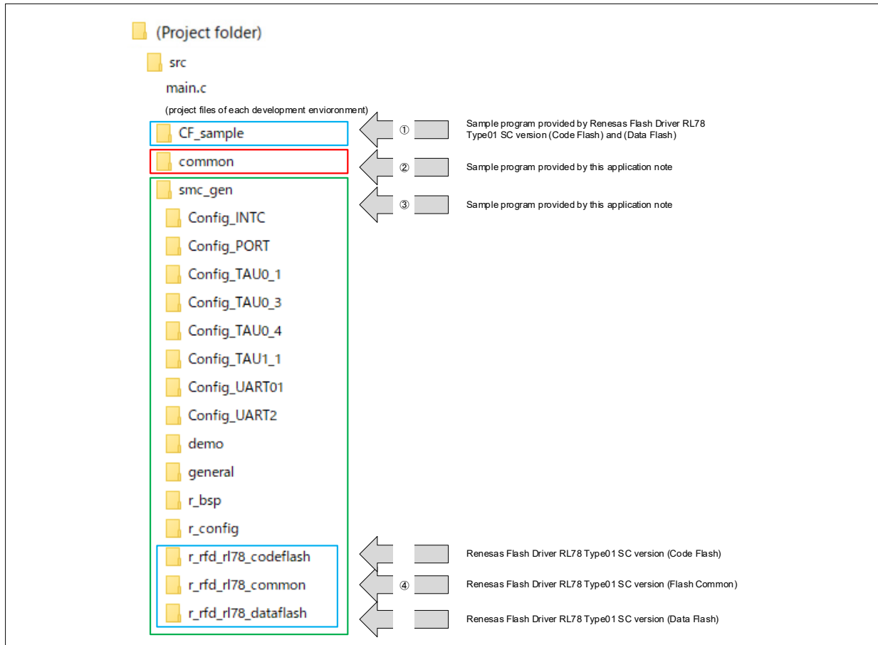
Figure 5-1 Folder Structure of Sample Program
