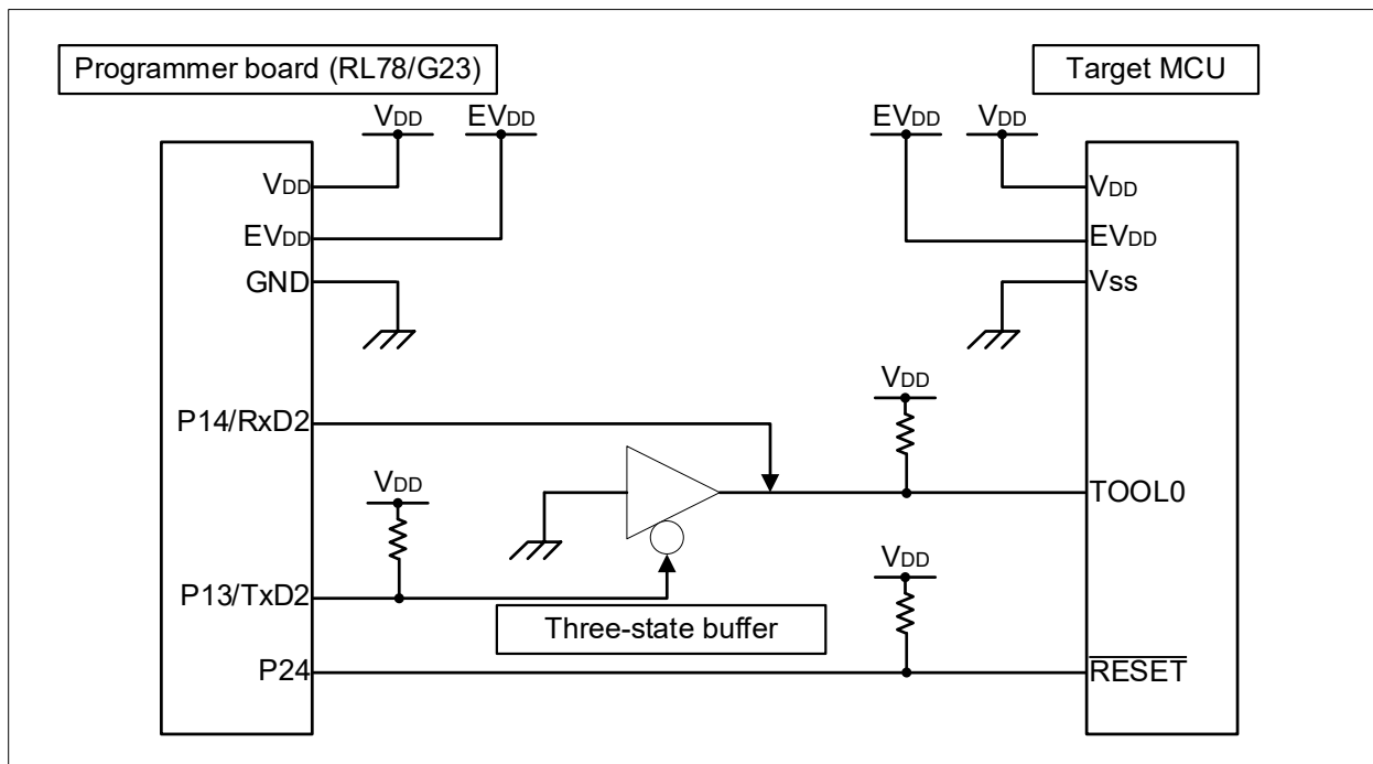
Figure 4-3 Single Line UART (VDD ≠ EVDD)
