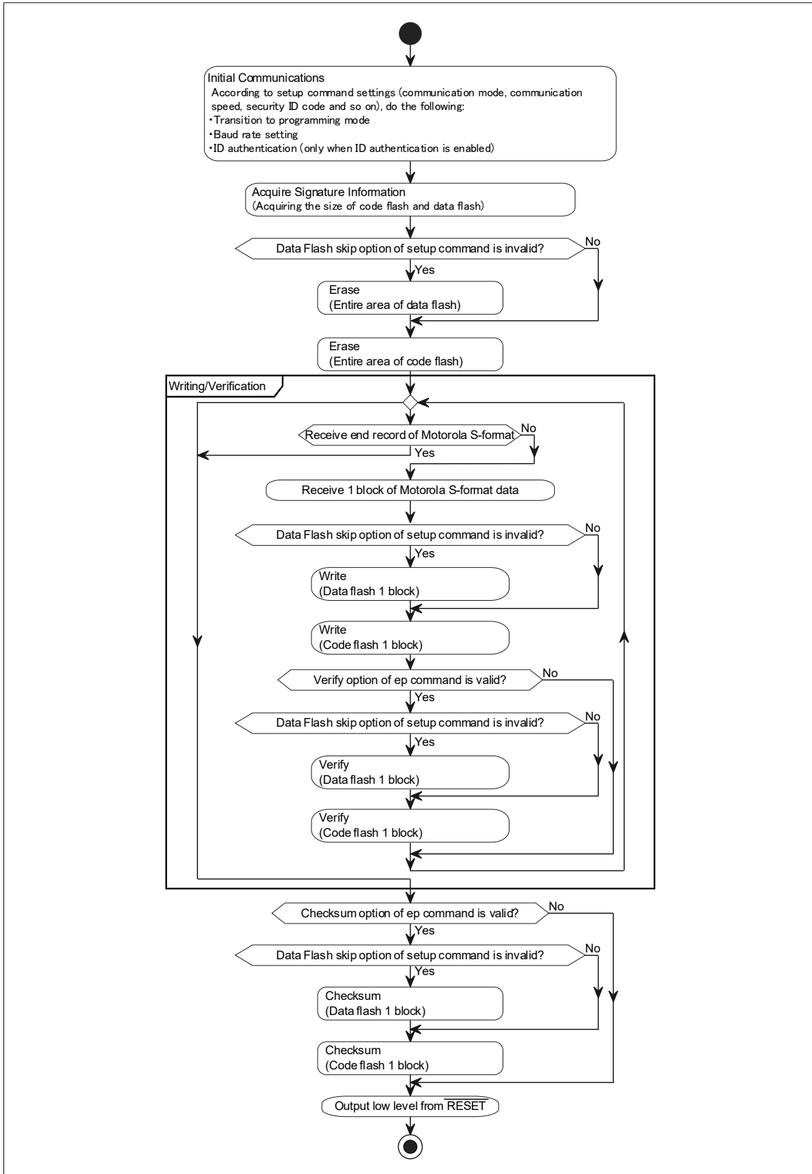
Figure 3-5 Online Mode
