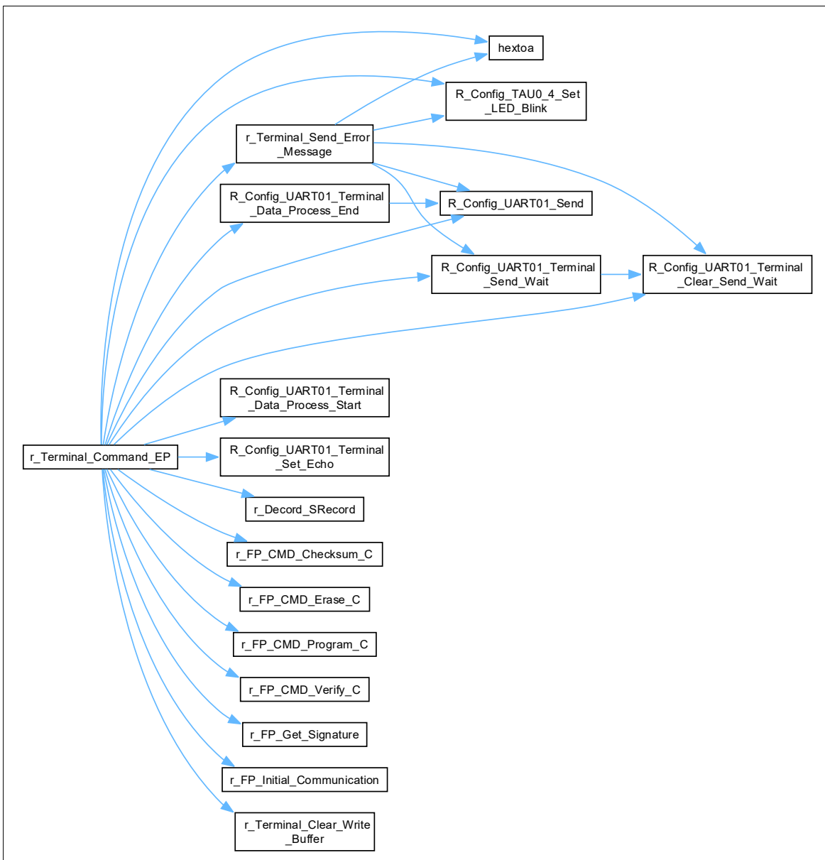
Figure 5-14 Call Graph of r_Terminal_Command_EP
