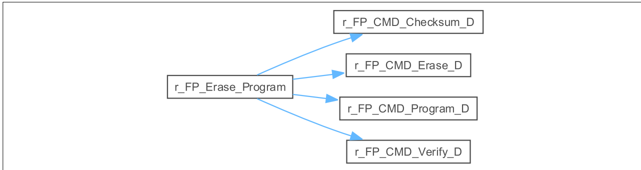
Figure 5-37 Call Graph of r_FP_Erase_Program
