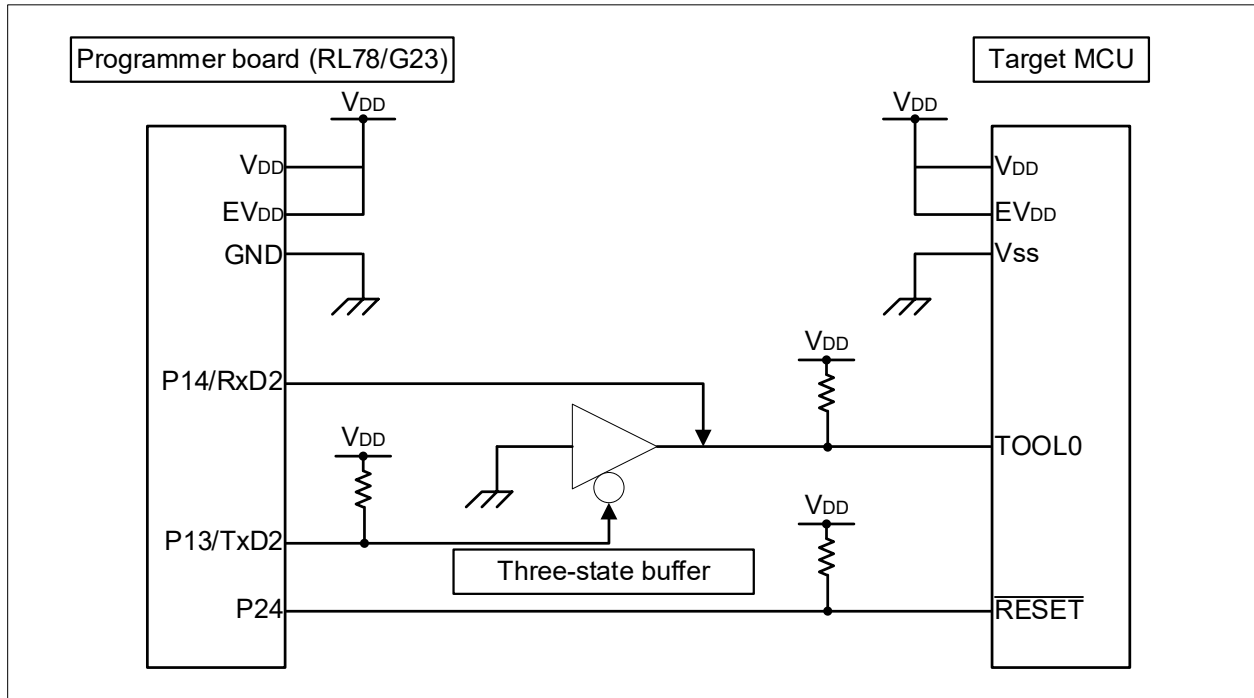
Figure 4-2 Single Line UART (VDD = EVDD)
