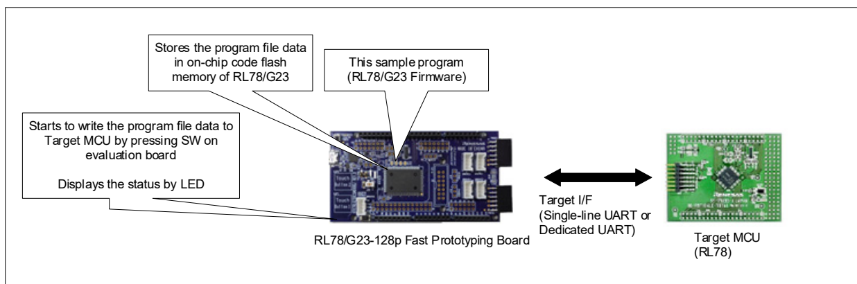
Figure 1-2 Offline Mode
