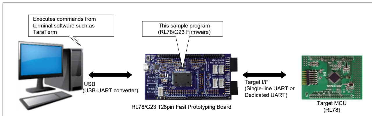
Figure 1-1 Online mode
