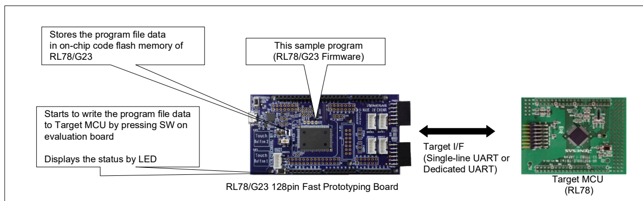
Figure 1-2 Offline mode
