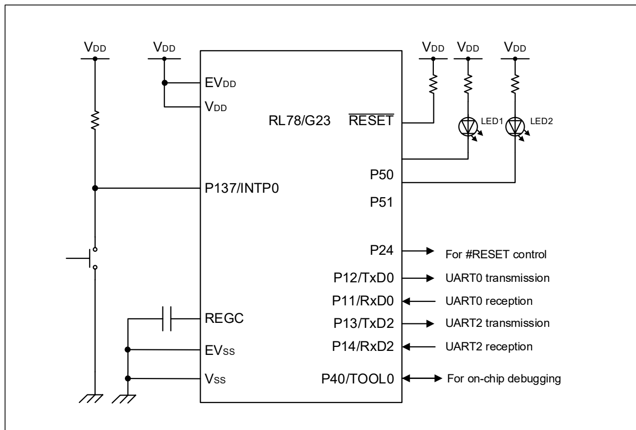
Figure 4-1 Hardware Configuration
