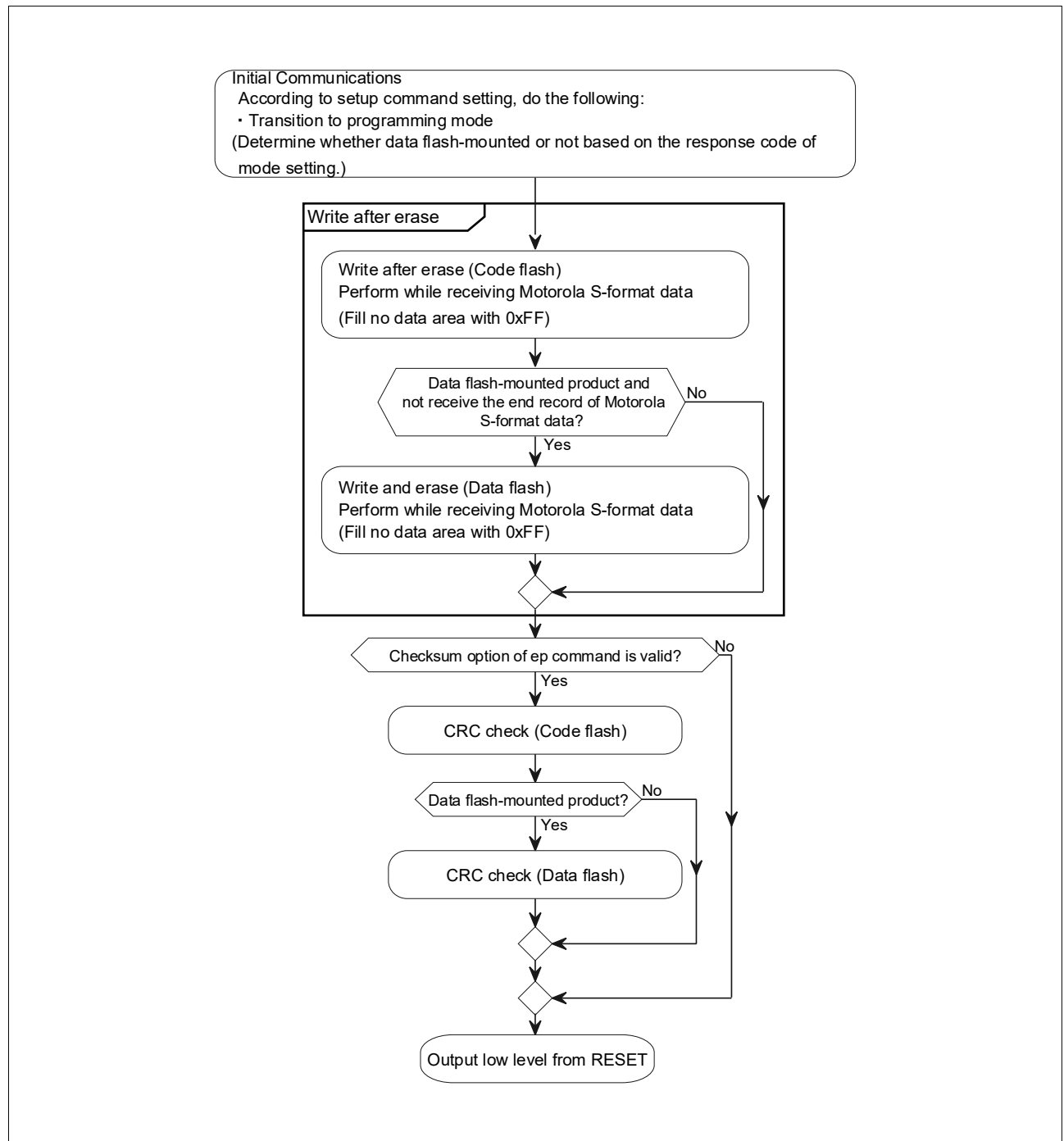
Figure 3-5 Online Mode
