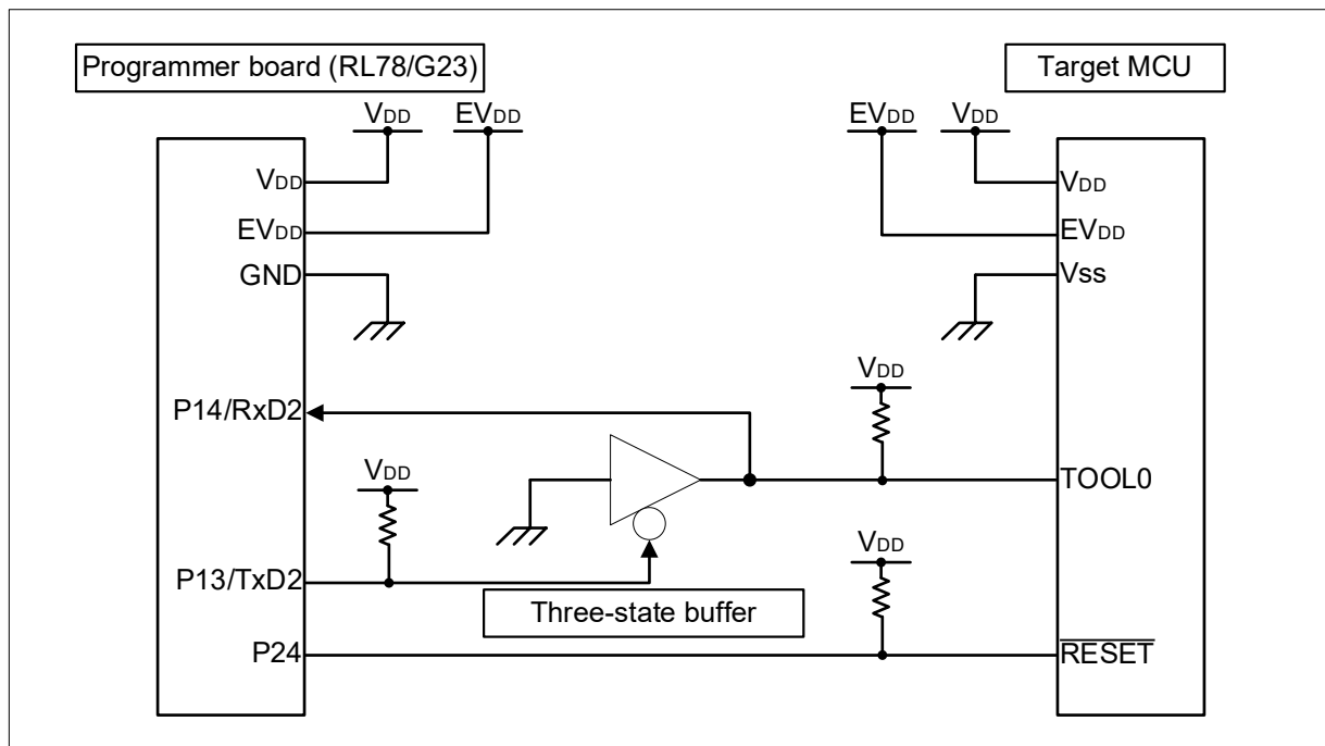
Figure 4-2 Single Line UART
