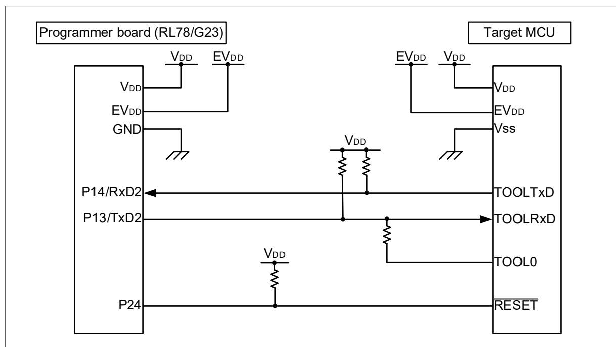
Figure 4-3 Dedicated UART
