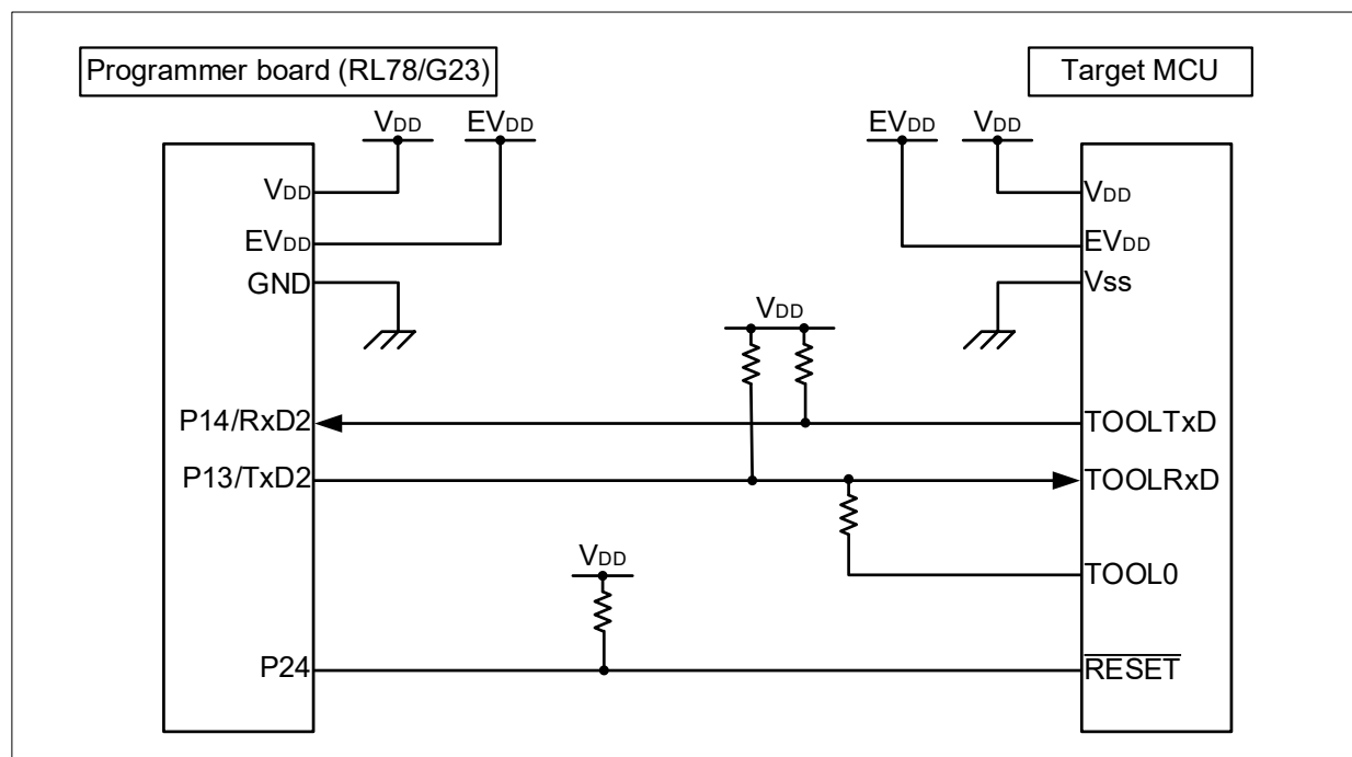
Figure 4-3 Dedicated UART
