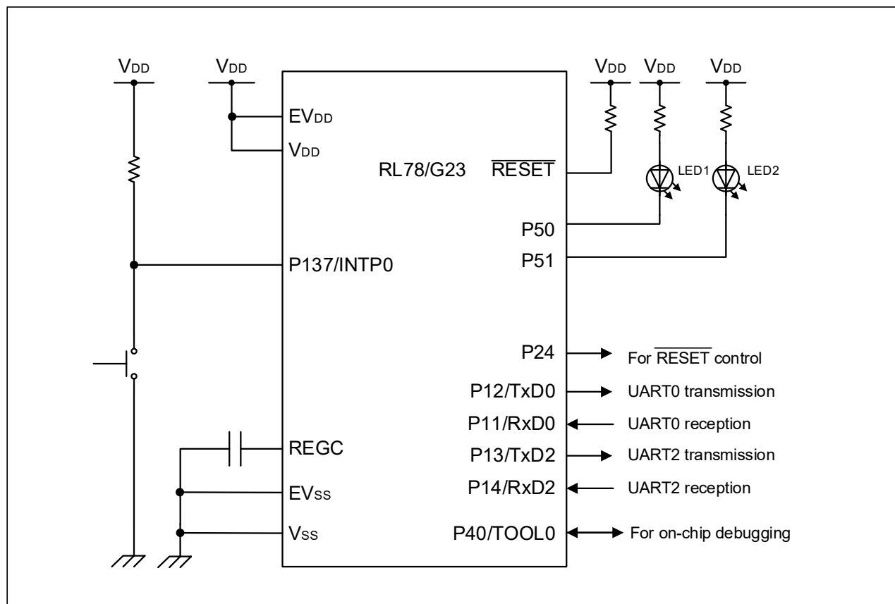
Figure 4-1 Hardware Configuration
