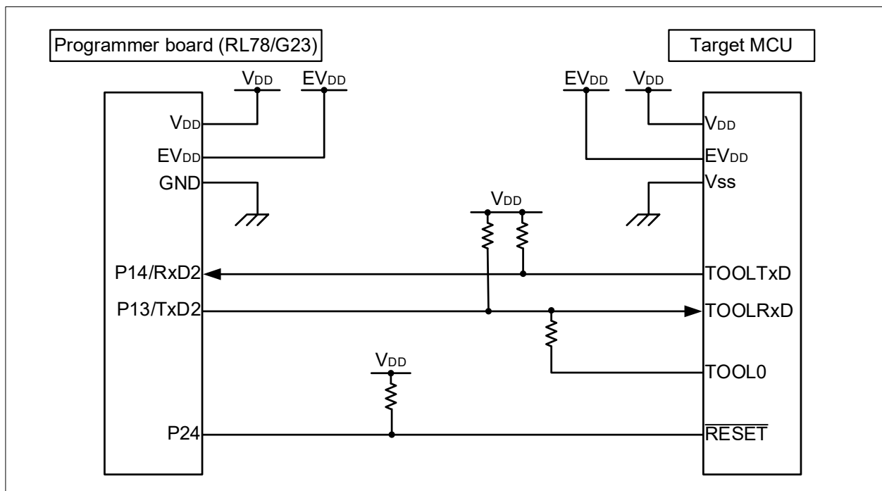
Figure 4-3 Dedicated UART
