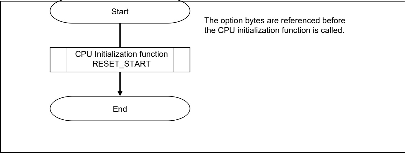
Figure 5.1 Overall Flowchart
